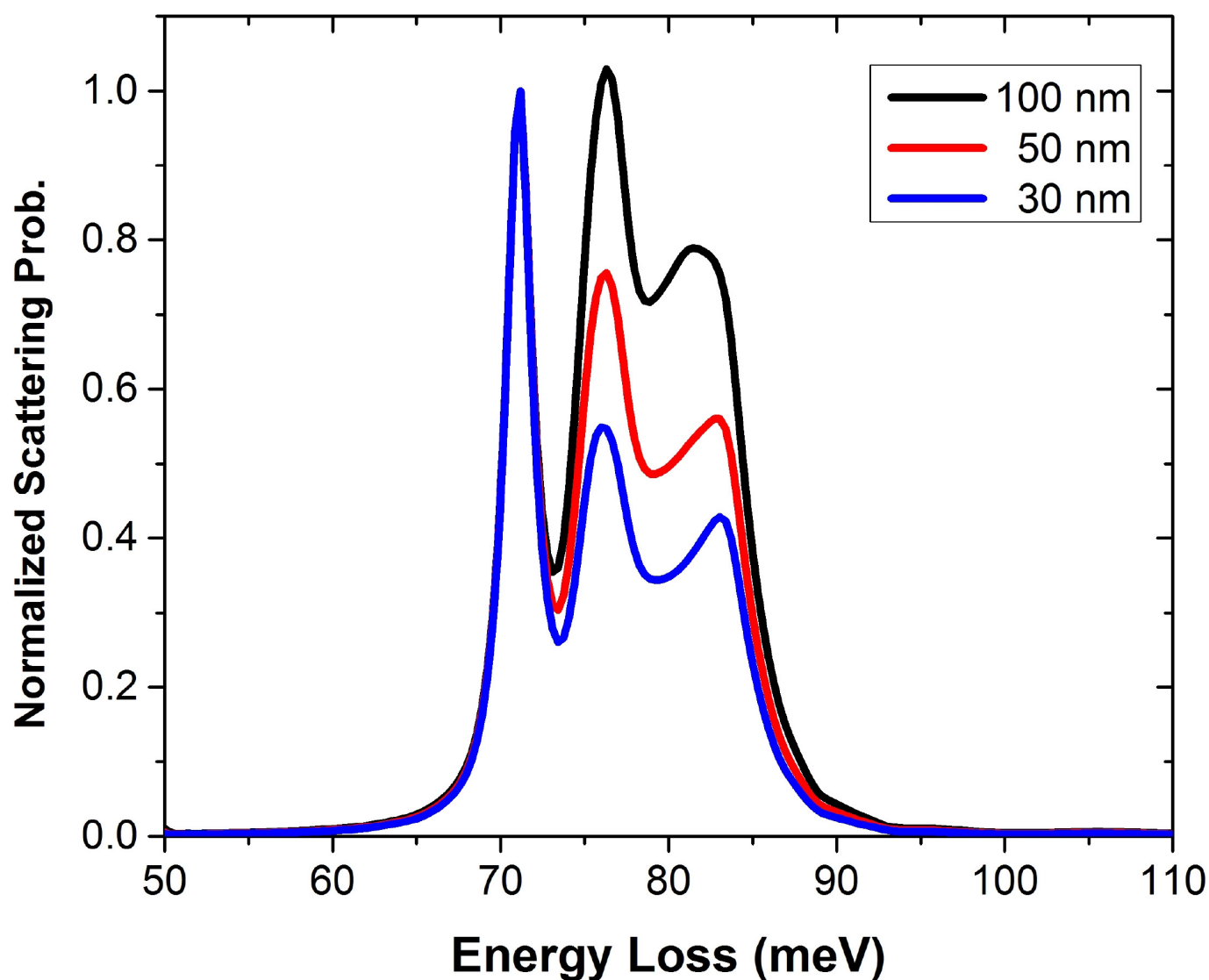
Extended Data Figure 3 | Simulated EELS probabilities for cubes of different sizes, considering an electron probe in the aloof geometry in the middle of the cube face (5 nm away from the surface). At this location, the probe is able to excite corner, edge and face SPhP modes with different probabilities, as shown in Extended Data Fig. 1b (green curve).
