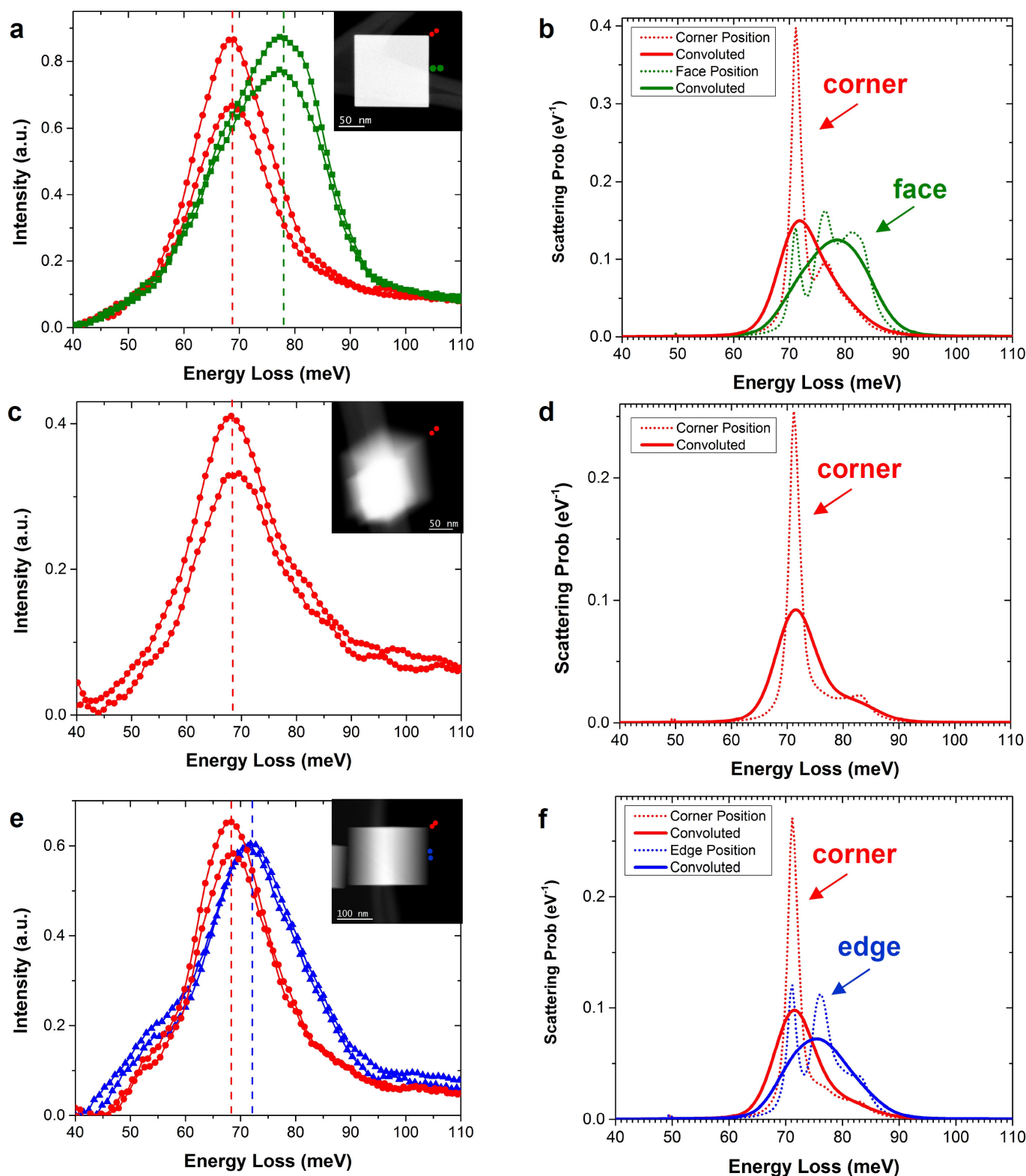
Extended Data Figure 1 | Excitation of corner, face and edge SPhP modes in approximately 150-nm MgO cubes. The excitation occurs in the aloeof geometry and the probe positions are indicated by dots in the ADF images (see insets of a , c and e ). a , c , e , Experimental EELS spectra for cubes oriented along the [001], [111] and [110] directions, respectively. b , d , f , Simulated EELS probabilities (dotted lines) corresponding to the configurations shown in a , c and e , respectively. The continuous lines are theoretical curves that correspond to the convolution of the dotted lines with a Gaussian function with a width of 10 meV, which accounts for the
