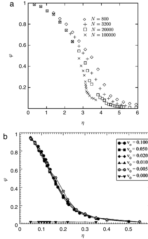
Fig. 32. Order parameter ( \phi ) versus noise ( \eta ) in the SVM. (a) The different kind of points belong to different system sizes. (b) The different curves belong to different v_0 velocities, with which each particles move. As it can be seen, the concrete value of v_0 does not effect the nature of the transition (except when v_0 = 0 , that is, when the units do not move at all).
