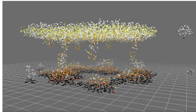
Fig. 57. (Color online) Simulation results, in which the motivational level of the individuals are taken into account. Large herring populations with small motivational synchronization tend to form multilayered schools in which the layers are connected by cylindrical shaped “bridges”. The motivational level depends primarily on the age of the fish: mature herrings are denoted with yellow color (online), ovulating ones are orange to red, spawning individuals are black and white color registers spent herring.
