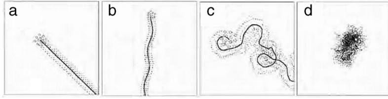
Fig. 45. Trajectories with various control parameters, obtained from numerical simulations. The solid line shows the center of mass. (a) marching, (b) oscillation, (c) wandering, and (d) swarming. Source: Adapted from Sugawara et al. (2007).
