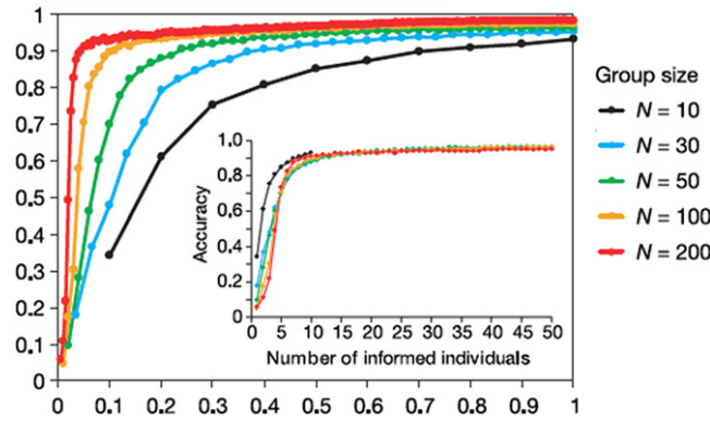
Fig. 62. (Color online) SPPs following simple rules can compose systems in which a few informed individual is capable to guide the entire group towards a preferred direction. The accuracy of the group (following the rules given by Eqs. (57)–(59)) increases asymptotically as the portion of the informed individuals increases.
