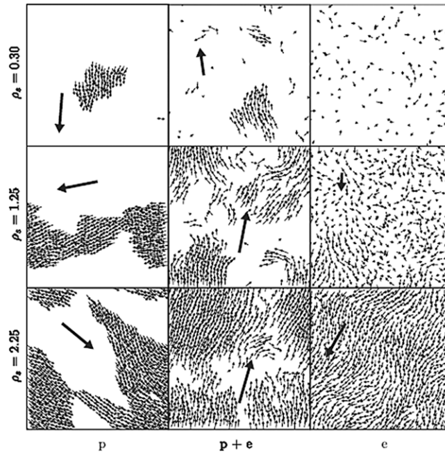
Fig. 59. The global collective motion emerging from escape and pursuit behaviors. \rho_s is the rescaled density , which is defined as \rho_s = Nl_s^2/L^2 , where N is the total number of the individuals, l_s is their interaction range and L is the size of the simulation field. The simulations were carried out by using periodic boundary conditions. The column denoted by p shows the typical spatial configurations for the pursuit-only case, e for the escape-only case, and p + e when both interactions are present. The large arrows indicate the direction and speed of the mean migration. As it can be seen on the top row, at low rescaled densities the emergent patterns strongly vary according to the strength of the escape and pursuit interactions.
