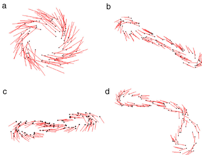
Fig. 35. (Color online) (a) A “mill”, (b) a “rotating chain” without intersection, (c) with one junction, and (d) with two self-intersections.
