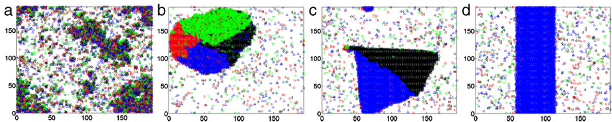
Fig. 40. (Color online) As the particles in the model exhibit an increasing tendency to align, different pattern arise: (a) orientational disorder, while particles self-segregate. (b) traffic jam, (c) glider, and (d) band. The colors code the four possible orientation: red is for 'right', 'left' is depicted with black color, green marks 'down', and 'up' is coded with blue. Source: From Peruani et al. (2011).
