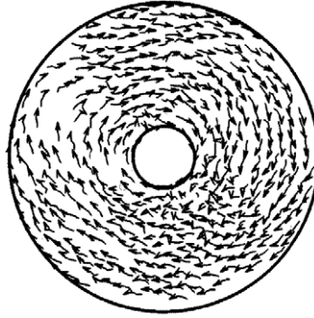
Fig. 51. A stationary state of the system characterized by short-range repulsion among the cells (defined by Eq. (49)) using reflective circular walls. Source: From Czirák et al. (1996).
