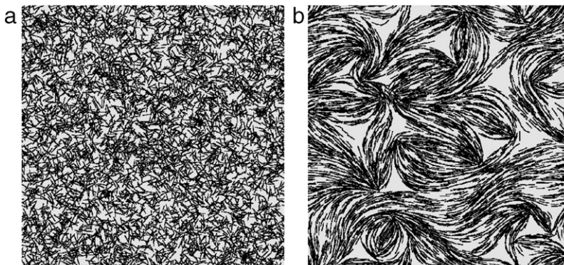
Fig. 50. Simulation results of the bacteria motion and pattern formation deep inside the colony. (a) In the initial setup the cells are randomly distributed. (b) The inner area of the colony after 3 h of evolution.
