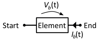
FIG. 2. Arbitrary two-terminal component on a branch, b , between two nodes (dots). The voltage, V_b(t) , over the component is defined from the start of the branch to the end of the branch. The current, I_b(t) , through the branch is defined in the opposite direction.
