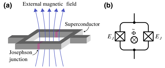
FIG. 5. A dc superconducting quantum interference device (dc SQUID). (a) Implementation of a dc SQUID. (b) Corresponding circuit diagram.
