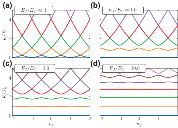
FIG. 17. The energies of the lowest-lying states of the single Cooper-pair box and transmon qubit as a function of the bias charge n_g . The difference between the two lowest bands is approximately equal to E_J at the avoided crossing.
