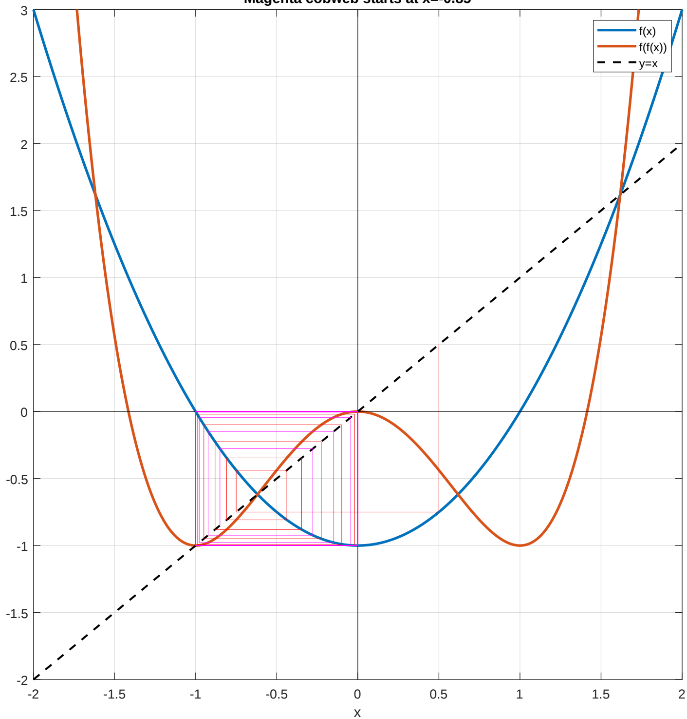
f(x) and f(f(x)) Red cobweb: starts at x=0.5 Magenta cobweb: starts at x=-0.85
