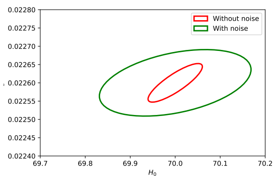
Plot of the confidence ellipse from the two constrained cosmological parameters.
