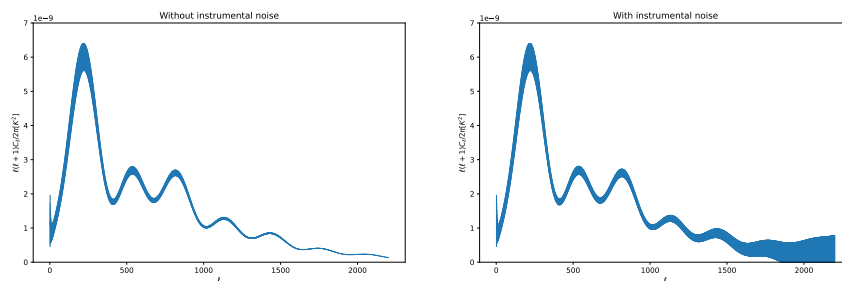
Plot of the uncertainty on the CMB spectrum.
