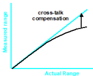
Figure 8. Crosstalk compensation
