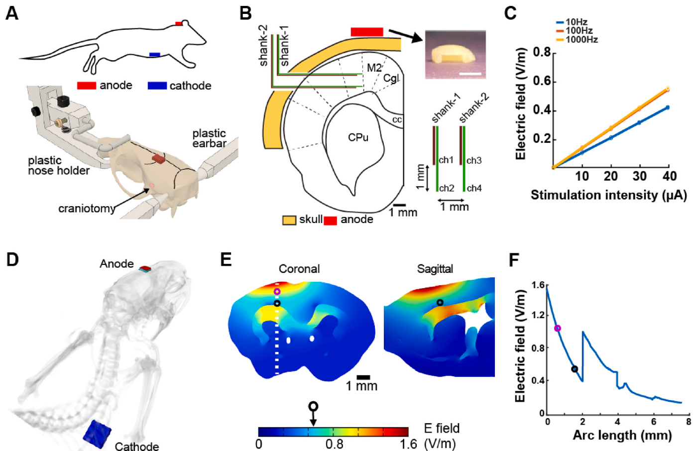
Fig. 1. Measurement and modeling of tES-induced electric field in motor cortex. (A) Electric field measurement in the motor cortex of rats. Top: An electrode is affixed to the skull above the primary motor cortex (3 by 3 mm platinum plate, anode), and a return electrode is implanted inside the chest wall (10 by 10 mm platinum mesh, cathode). Bottom: 3D-printed nose holders and ear bars are used to isolate the animal from the metallic components of the stereotactic frame during measurements. The rat skull is shown inside the nose holder with skull electrode (red rectangle) and craniotomy in the parietal bone. (B) Schematic of the position of recording electrodes in the motor cortex. Note that electrodes were inserted from the lateral side of the skull through the temporal craniotomy. Top, right: Customized holder for the stimulation electrode (scale bar is 3 mm). Bottom, right: schematic of the custom-built, 2-shank, 4-channel tungsten recording matrix. Each shank had 2 recording channels (both ch1 and ch2 and shank-1 and shank-2 are separated by 1 mm). (C) Increasing stimulation intensity induces an increasing electric field in the motor cortex. The reduced slope of the 10 Hz condition could be induced by the built-in 0.7 Hz high-pass filter of the preamplifier. (D) Anatomically accurate FEM model including skull electrode (red) and gel (green) and chest electrode (blue). (E) Distribution of field magnitude estimated with the current flow model in the coronal and sagittal plane at 40 \mu A current. (F) Field amplitude as a function of distance from the cortical surface moving in radial direction (Arc length). The discontinuity is due to a discontinuity in conductivity (white matter of corpus colosseum has lower conductivity than gray matter, 0.126 S/m vs 0.276 S/m). (For interpretation of the references to colour in this figure legend, the reader is referred to the Web version of this article.)
