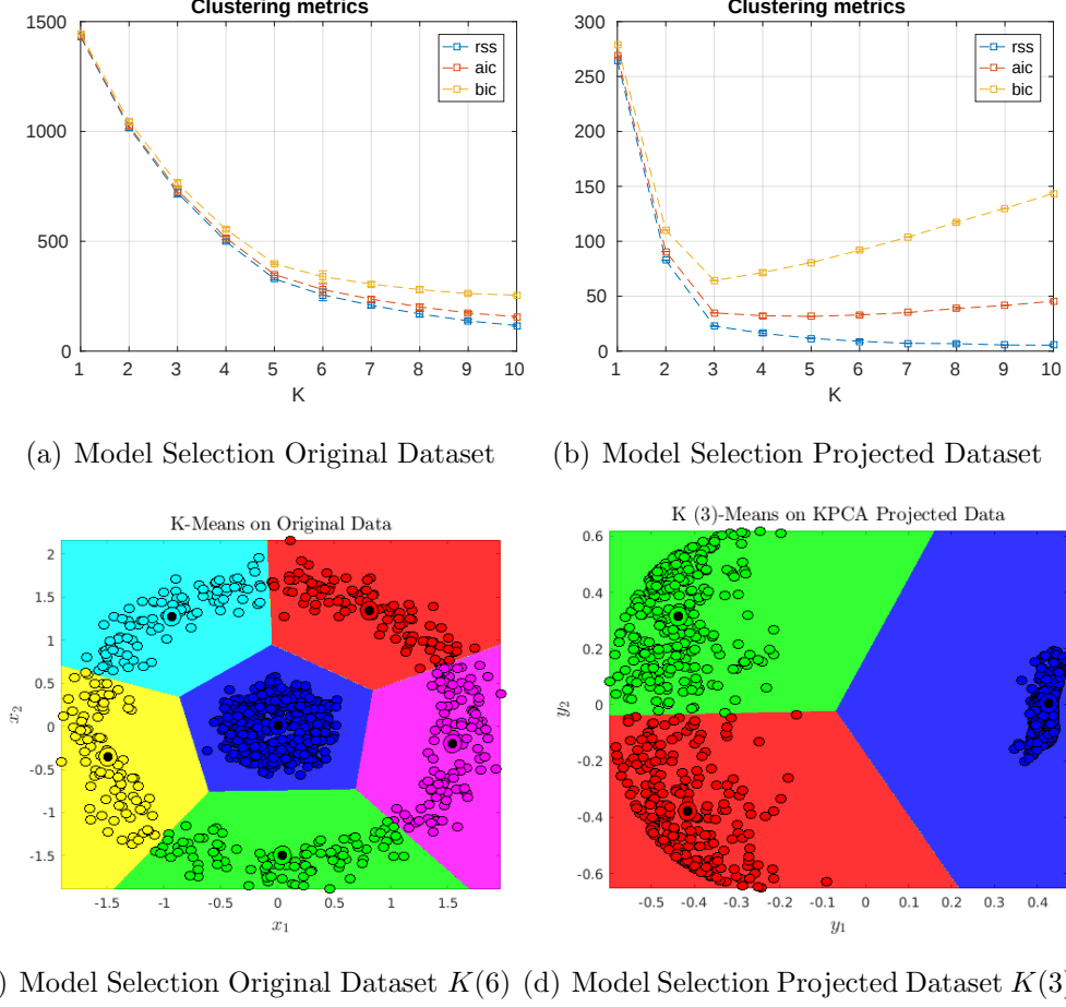
Figure 13: K -Means Model Selection on (a) Original Dataset and (b) Kernel PCA Projected Dataset with \sigma = 0.5 . According to these model selection procedures (c) Optimal K = 6 for the original dataset and (d) Optimal K = 3 for the projected dataset.
