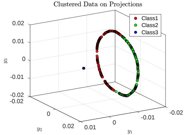
Figure 15: Circles Dataset Projected on first 2 Eigenvectors of Laplacian and clustered with K = 3 . Figure 16: Circles Dataset Projected on first 3 Eigenvectors of Laplacian and clustered with K = 3 .
