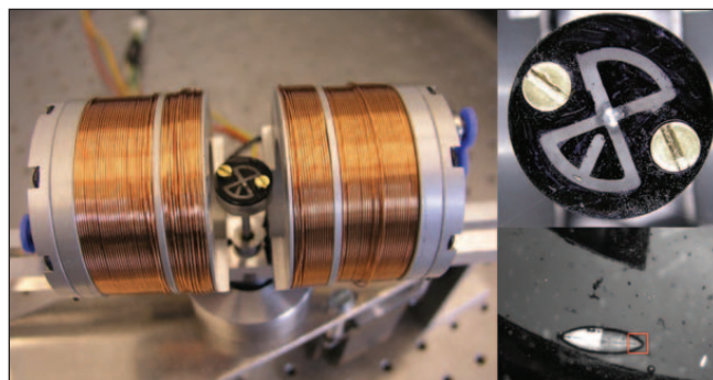
Figure 14. A 900\text{ }\mu\text{m} \times 400\text{ }\mu\text{m} assembled-MEMS microrobot navigating a fluid-filled maze. A motorized magnetic coil system provides computer-controlled field magnitude, orientation, and gradient.
