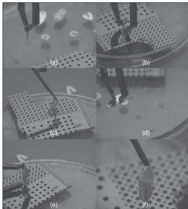
Figure 8. Sequence of a manual assembly process where component B of the microrobot is inserted in component A. (a) Component A is grasped and (b) inserted into a hole of the workbench. (c) UV-activated glue is applied. (d) Component B is picked up and (e) inserted into Component A. (f) The assembly of the two components is complete. The largest component in this microrobot (component B) is 940 \mu\text{m} long, 400 \mu\text{m} wide, and 50 \mu\text{m} thick.
