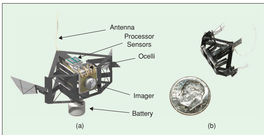
Figure 15. (a) Artist's conception and (b) current prototype of the micromechanical flying insect. Images courtesy Ronald S. Fearing and Robert J. Wood, University of California, Berkeley, USA.
