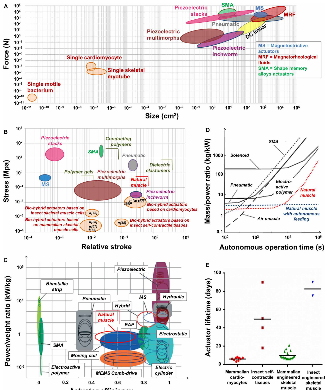
Fig. 5. Performance of biohybrid actuators and comparison with fully artificial counterparts. (A) Actuator force output versus its overall size. (B) Plotting of both artificial and biohybrid actuators in terms of stress produced versus relative stroke. Few references are reported in brackets for biohybrid actuators. (C) Plotting of artificial actuators and natural muscle in terms of power/weight ratio versus actuator efficiency (4). (D) Mass/power ratio, which takes into account both actuator and power source mass, versus actuator autonomous operation time. Some artificial actuation technologies are compared with natural muscle, assuming no periodical autonomous feeding (red line) and periodical autonomous feeding (blue line). Data in (C) and (D) reprinted from (4) with permission from Wiley. (E) Lifetimes of “general-purpose” biohybrid actuators reported in the literature for the different categories analyzed in this paper.
