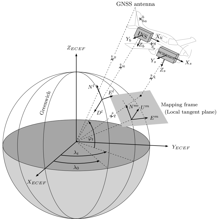
Figure 2.5: Geometry of direct sensor orientation.
