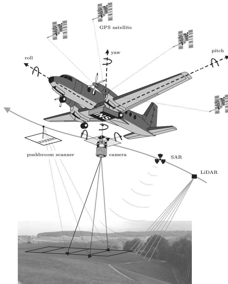
Figure 2.1: Use of navigation technology for sensor orientation.
