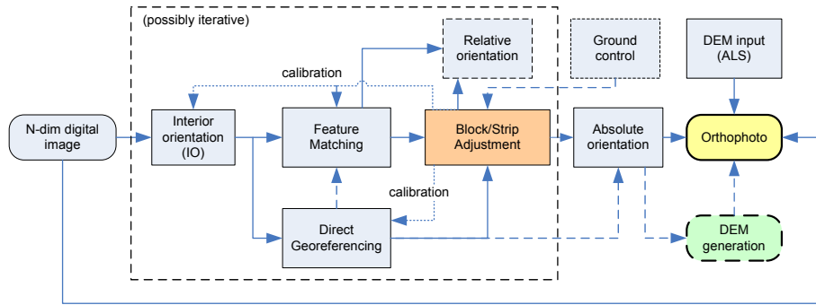
Figure 4.1: General overview of sensor fusion, with the optimization step denoted as block/strip adjustment, known also as assisted aerotriangulation (AAT).
