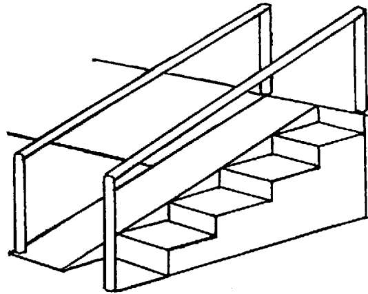
FIGURE 84. Combined ramp and stairs.
