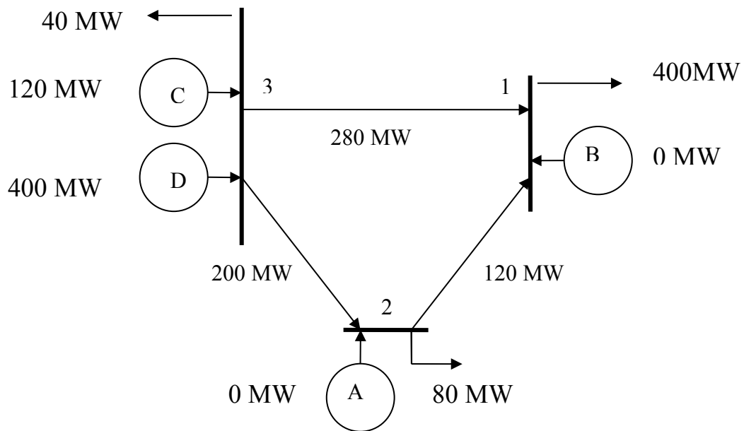
Figure 2 – Unconstrained economic dispatch
