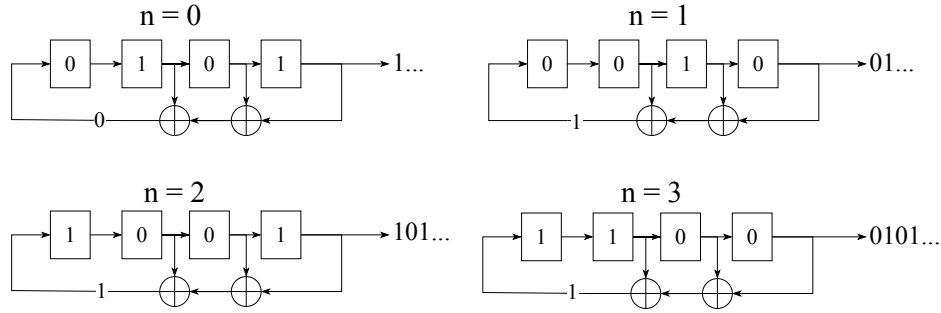
Figure 2.3: Illustration of Functionning principle of an LFSR
