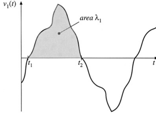
Fig. 15.2 An arbitrary transformer primary voltage waveforms, illustrating the volt-seconds applied during the positive portion of the cycle.
