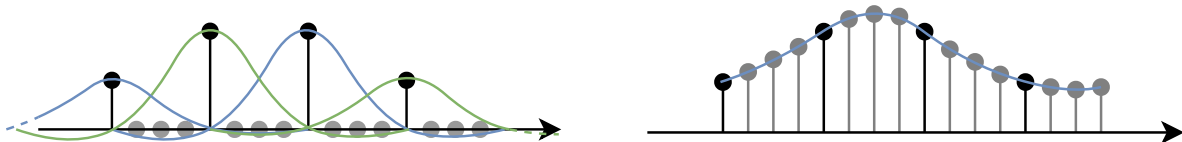
Figure 3.2: Signal before pulse shaping with symbol pulses illustration and signal after pulse shaping
