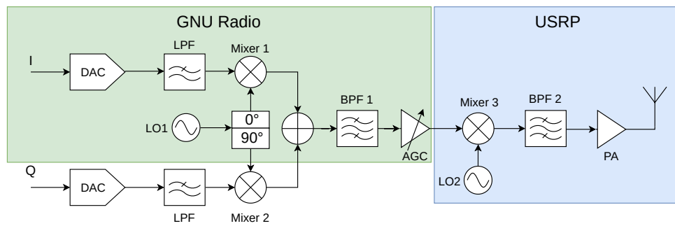
Figure 2.1: Superheterodyne Transmitter
