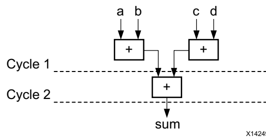
Figure 1-73: Adder Tree After Balancing
