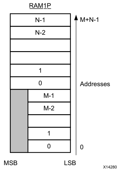
Figure 1-67: Memory for Horizontal Mapping
