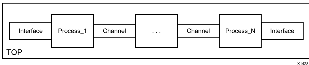
Figure 1-62: Parallel Process Architecture
