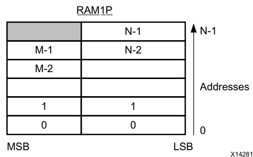
Figure 1-70: Memory for Vertical Mapping
