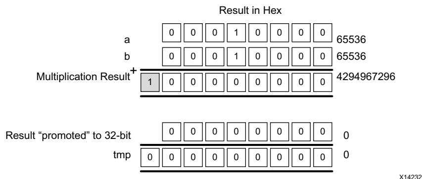
Figure 2-2: Integer Promotion
