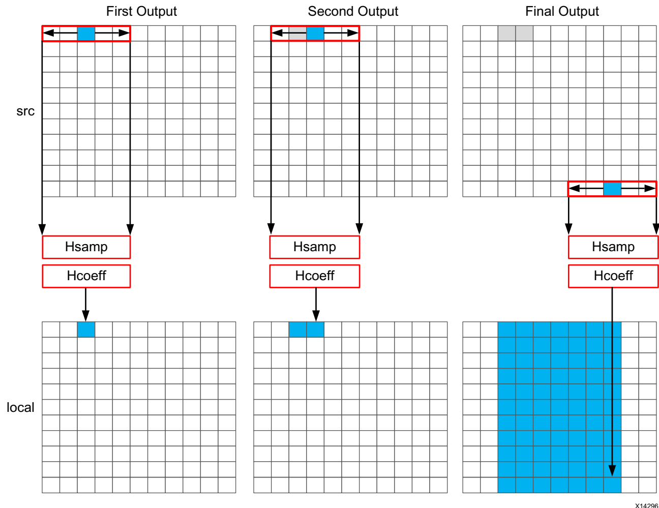
Figure 3-2: Horizontal Convolution
