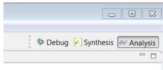
Figure 1-22: Analysis Perspective
