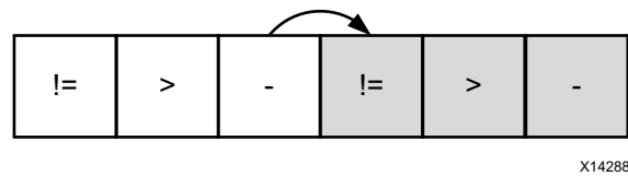
Figure 1-59: Scalar Dependency
