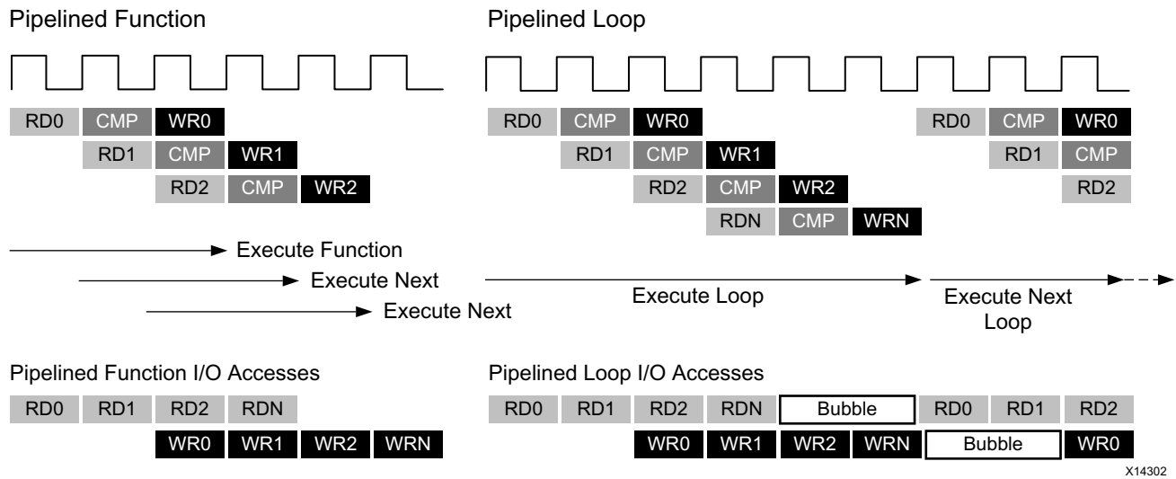
Figure 1-52: Function and Loop Pipelining Behavior
