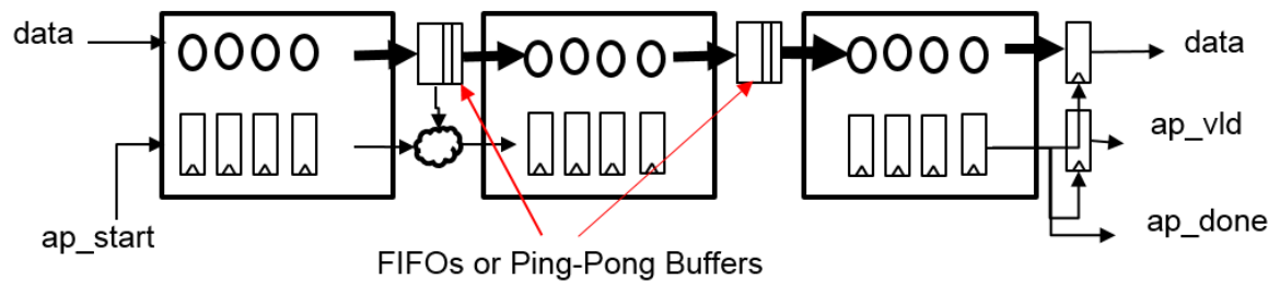
Figure 1-64: Structure Created During Dataflow Optimization
