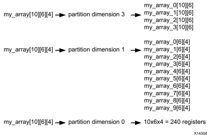
Figure 1-56: Partitioning Array Dimensions
