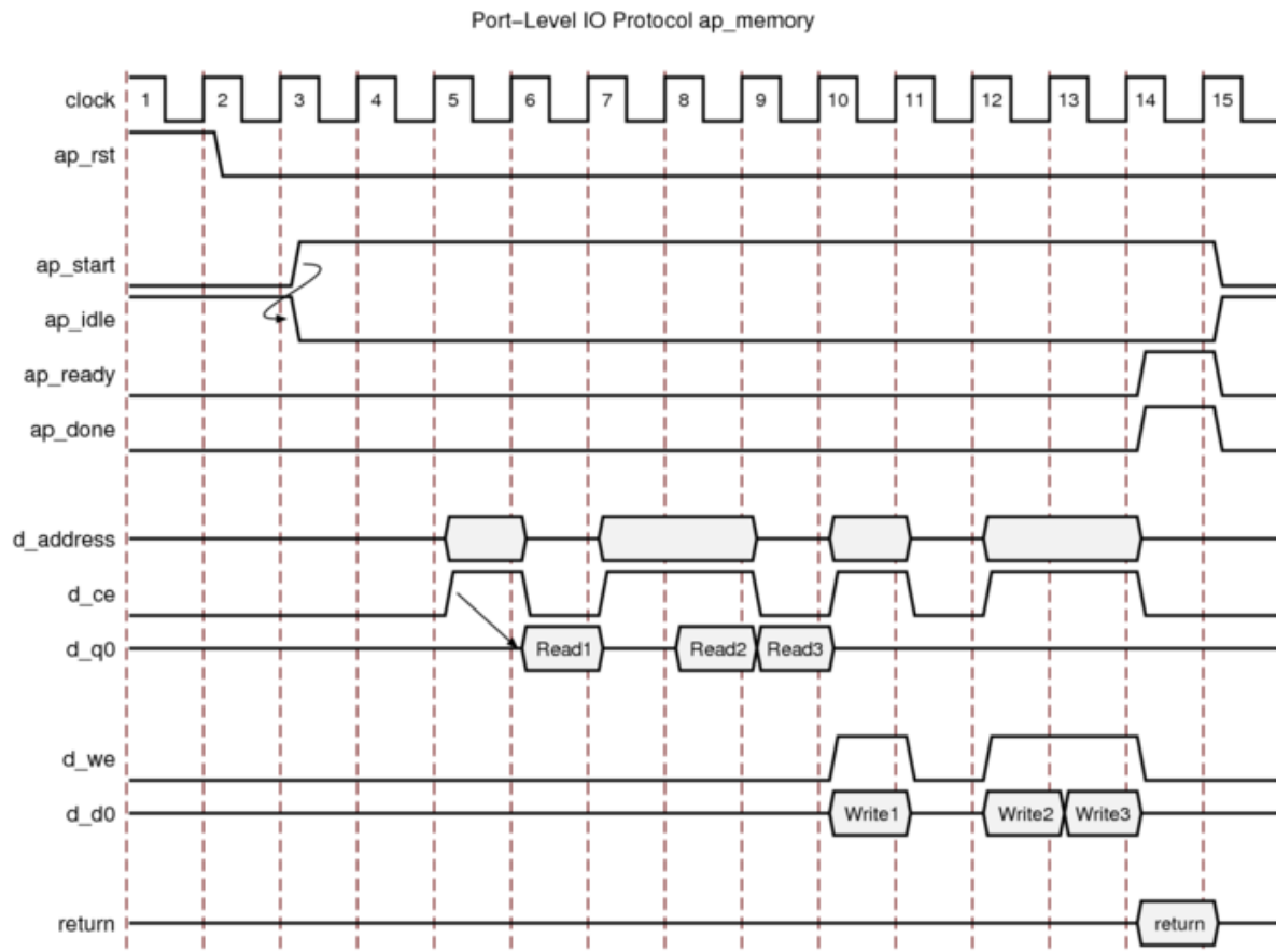
Figure 4-9: Behavior of ap_memory Interface
