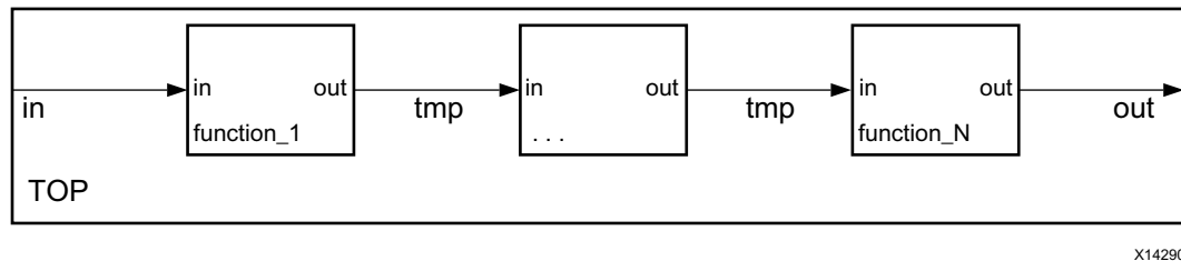
Figure 1-61: Sequential Functional Description
