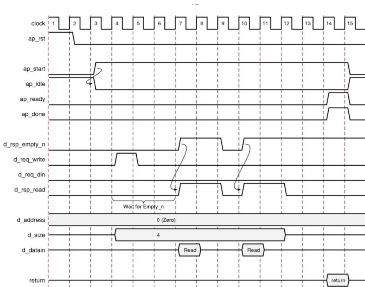
Figure 4-13: Behavior of ap_bus Interface: Burst Read
