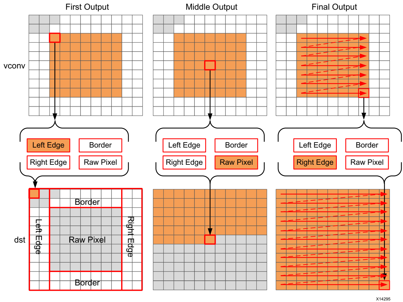
Figure 3-8: Streaming Border Samples
