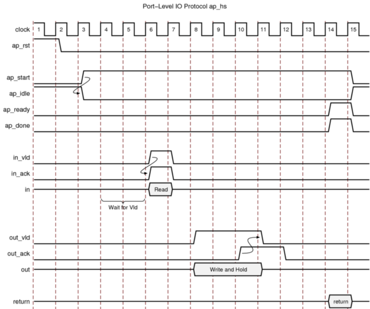
Figure 4-8: Behavior of ap_hs Interface
