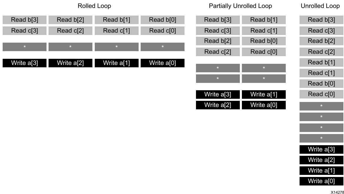
Figure 1-60: Loop Unrolling Details
