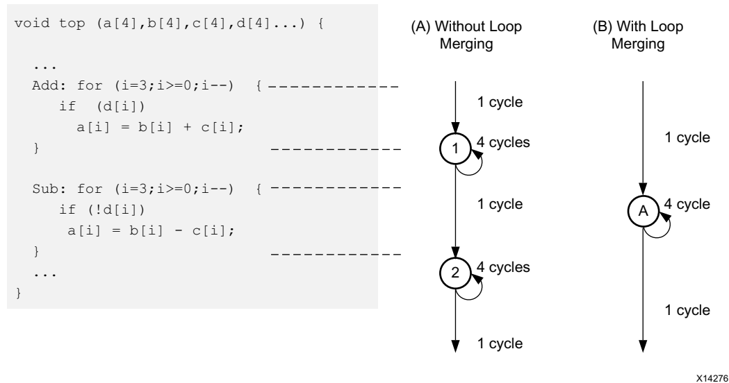
Figure 1-65: Loop Directives
