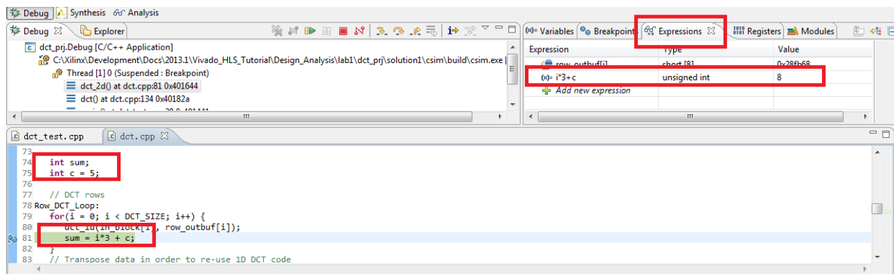
Figure 4-2: Monitoring Expressions
