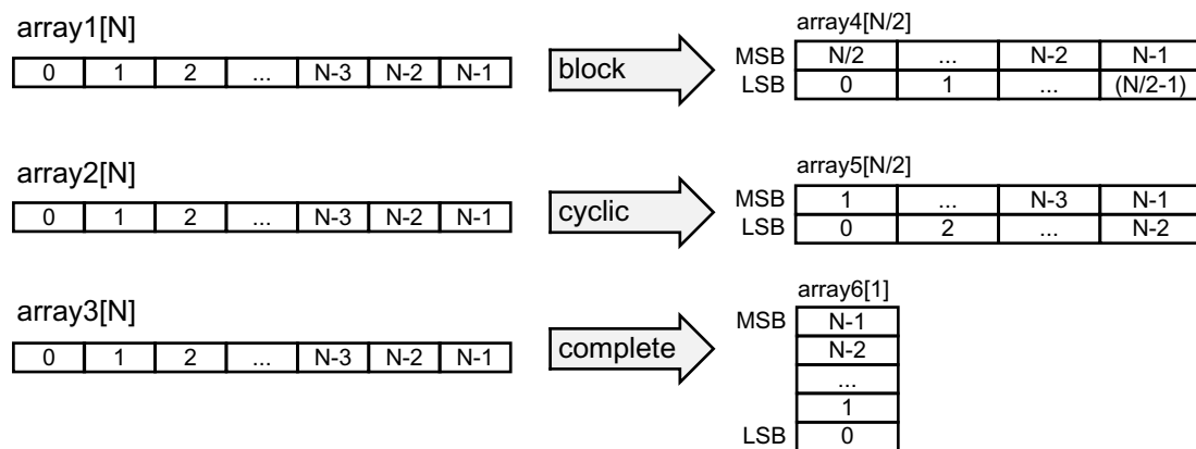
Figure 1-71: Array Reshaping
