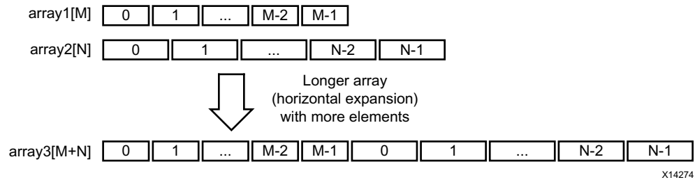
Figure 1-66: Horizontal Mapping
