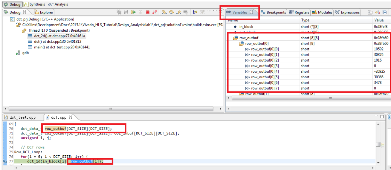
Figure 4-1: Monitoring Variables
