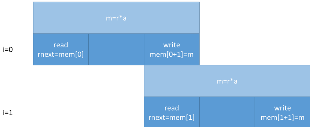
Figure 1-57: Dependency Example
