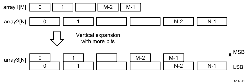
Figure 1-69: Vertical Mapping
