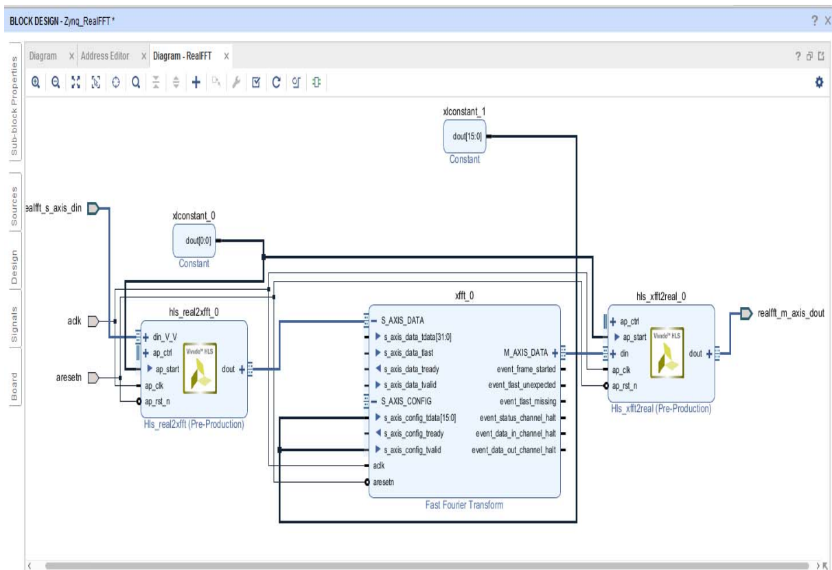
Figure 10-39: Final RealFFT Diagram
