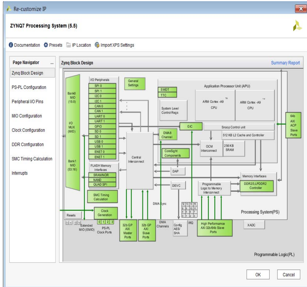
Figure 10-13: Configure the Zynq AP SoC
