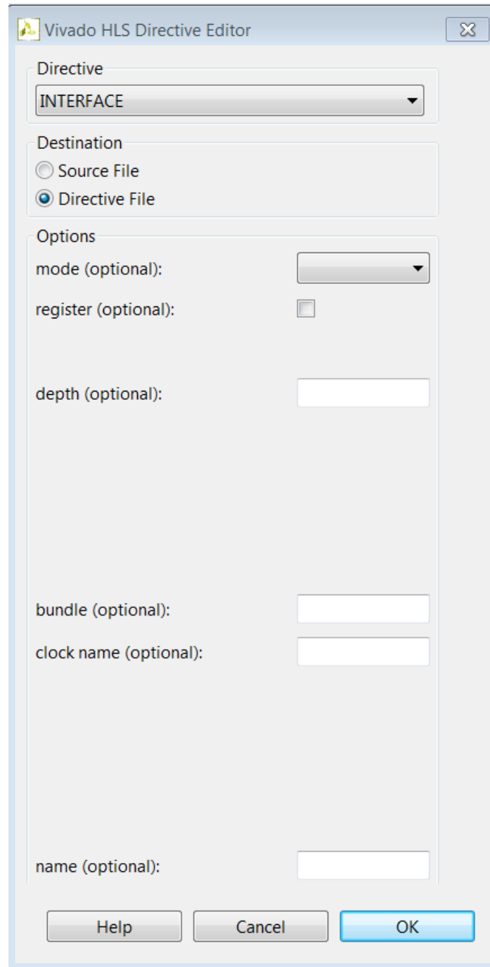
Figure 4-8: Directive Dialog Box for ap_ctrl_none
