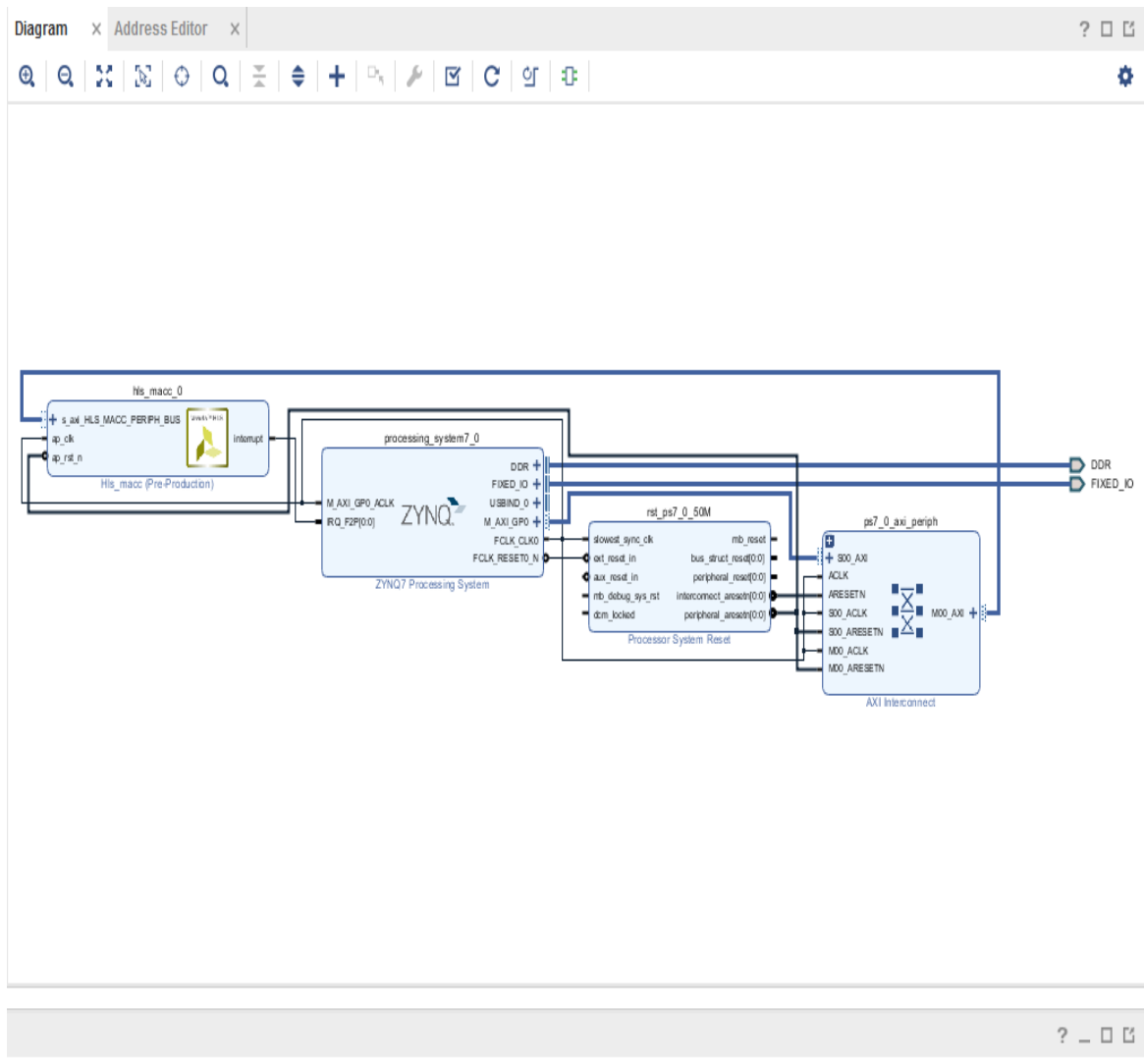
Figure 10-18: Design with AXI4 Interconnect
