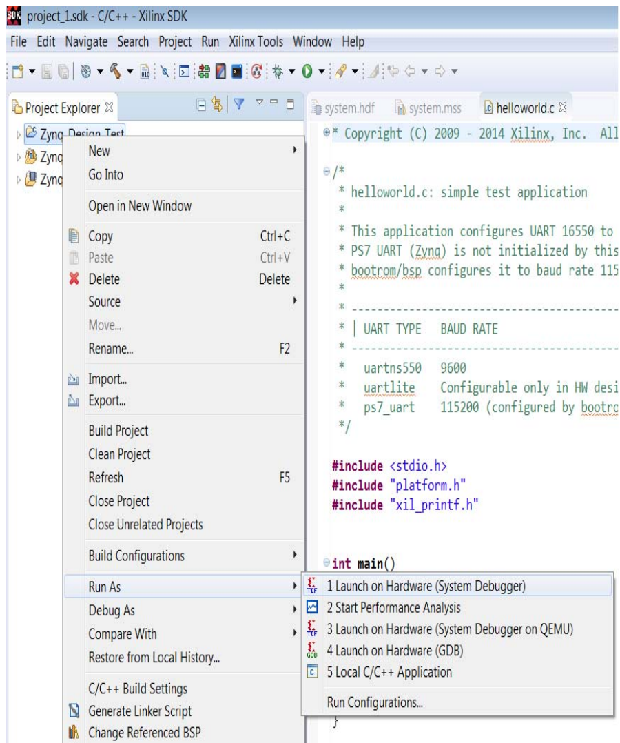
Figure 10-25: Run the Application Project
