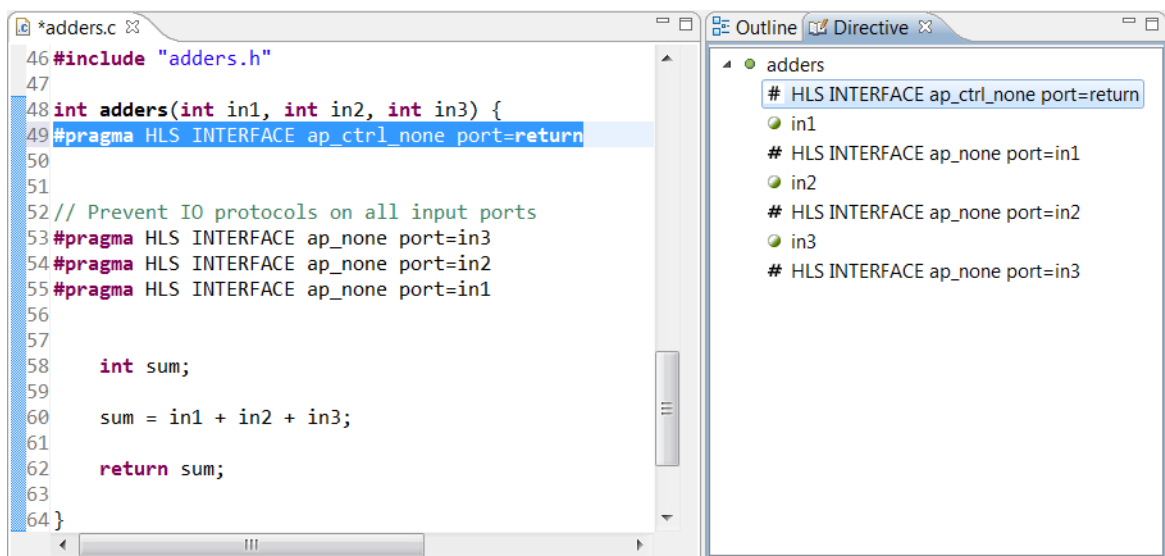
Figure 4-9: Block-Level Interface Directive ap_ctrl_none
