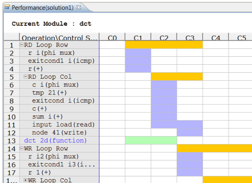
Figure 6-9: Expanded View of RD_Loop_Row
