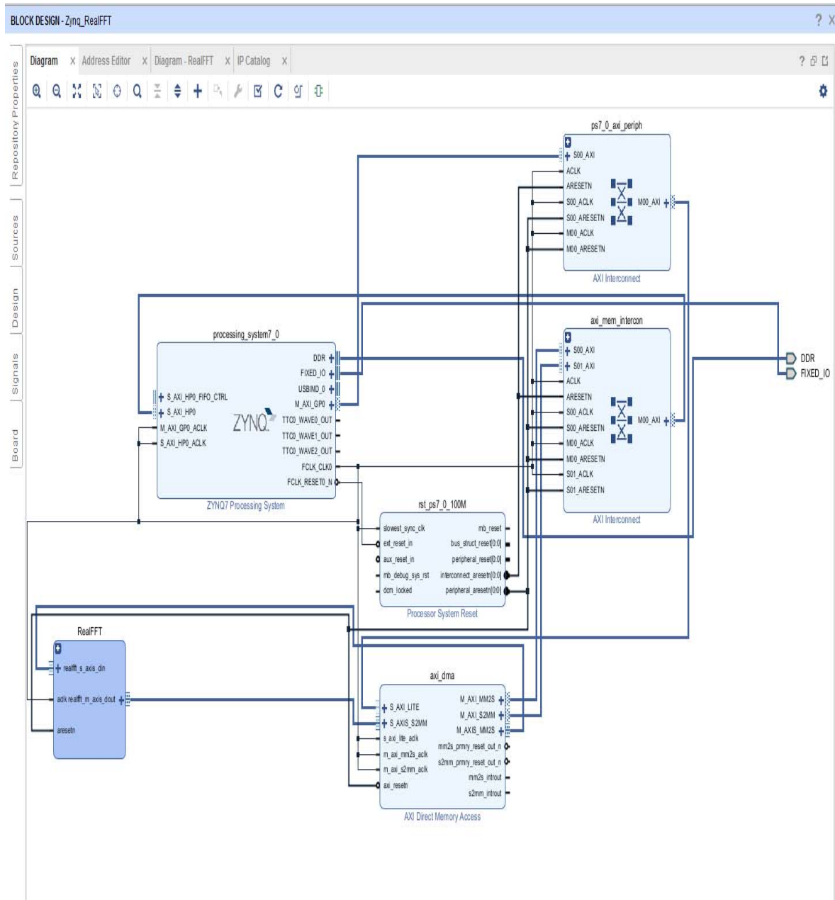
Figure 10-42: Zynq Diagram with Internal Connections
