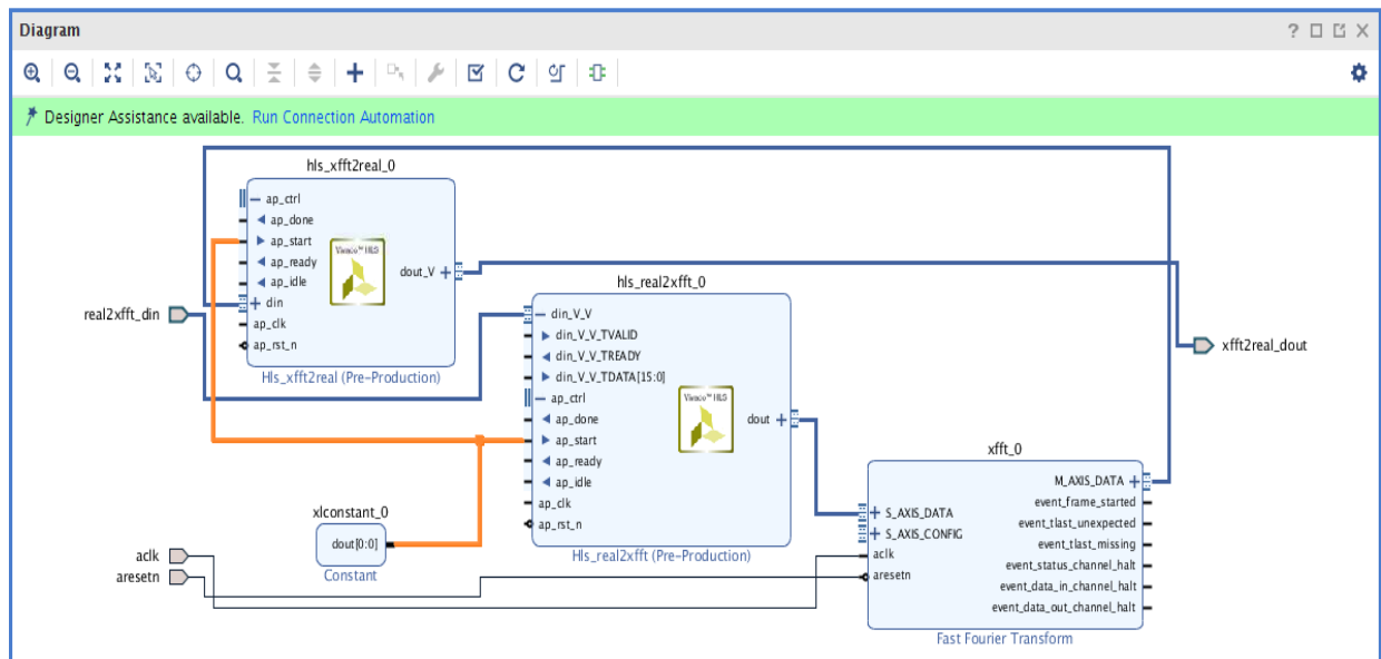
Figure 9-22: Connect AP_START to Constant
