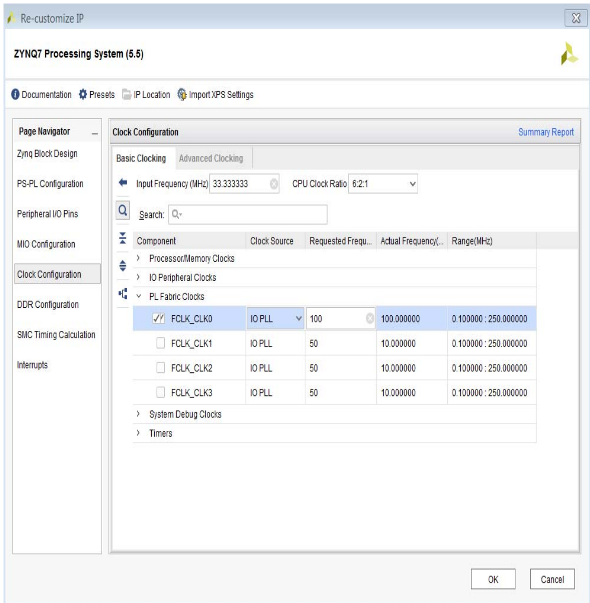
Figure 10-41: Configuring the Clock
