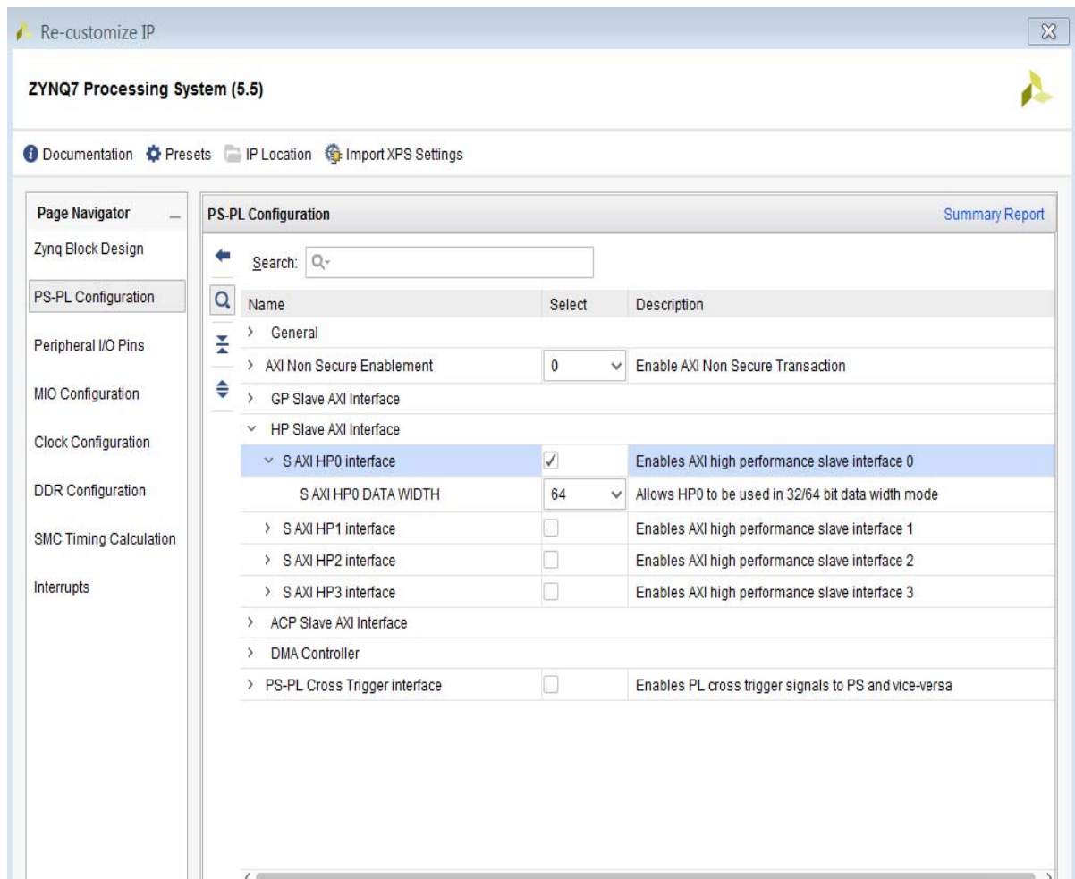
Figure 10-40: Configuring Port HP0
