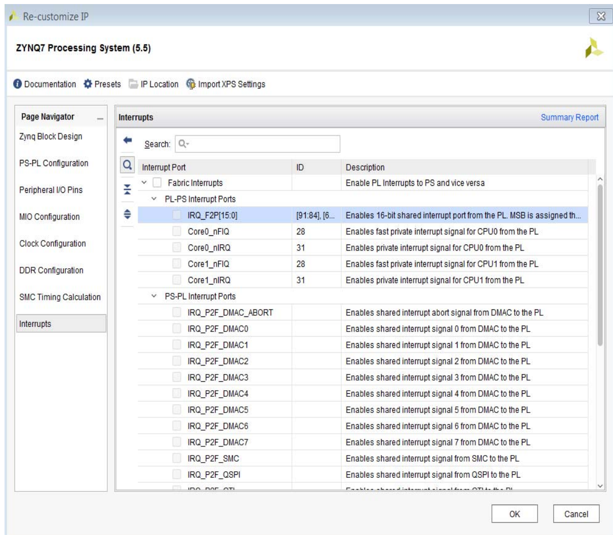
Figure 10-15: Zynq AP SoC Interrupt Configuration
