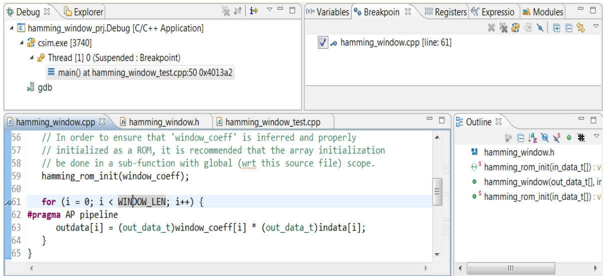
Figure 3-20: Debug Environment for C Validation Lab 3
