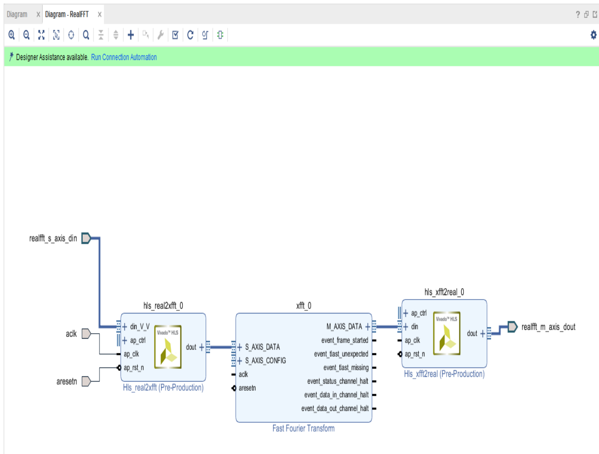
Figure 10-37: RealFFT Diagram with All Pins
