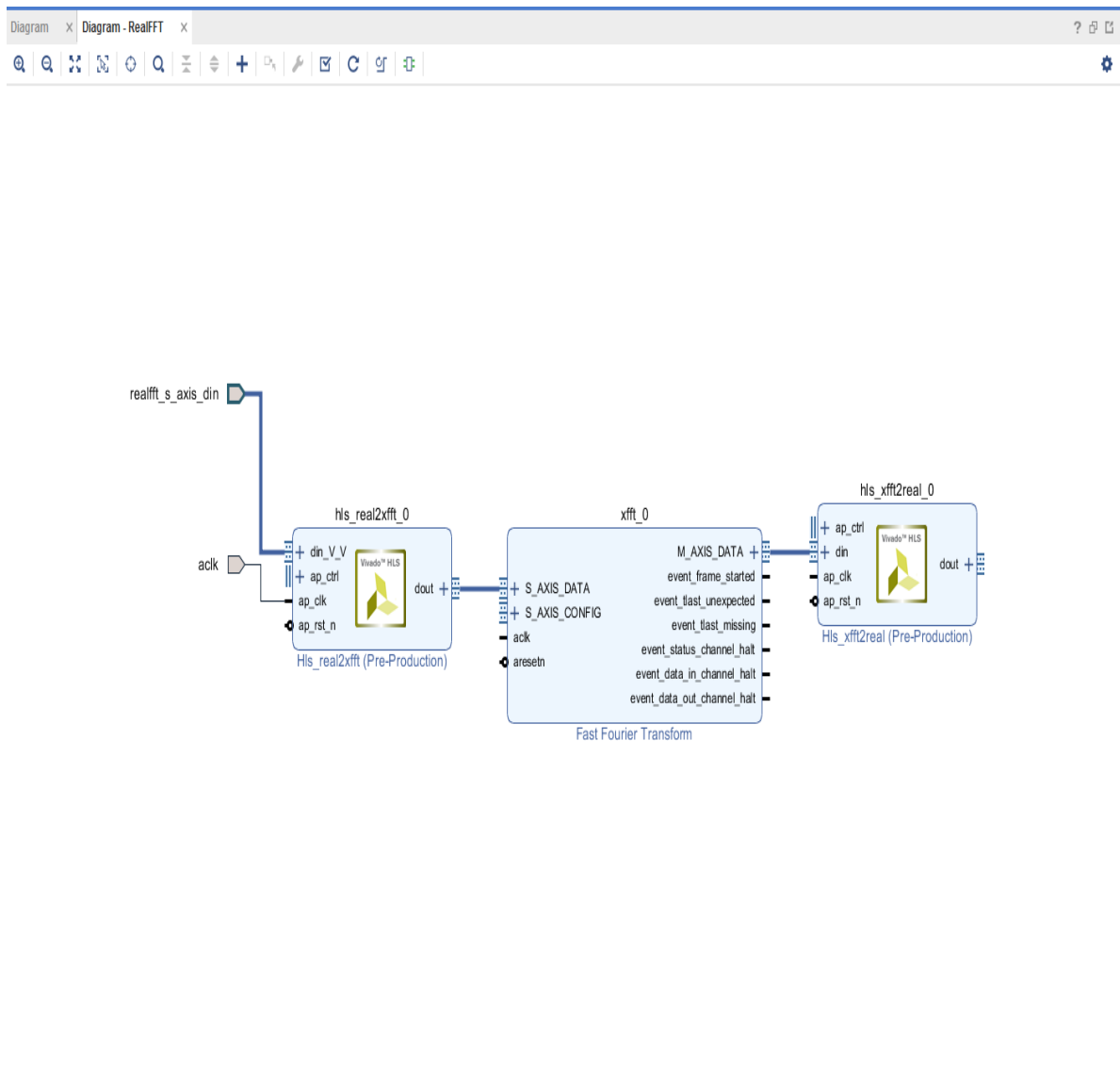
Figure 10-36: RealFFT Diagram with Interface Pin and Clock Pin
