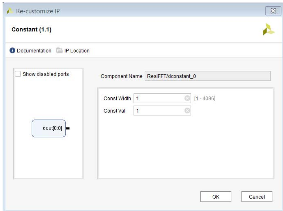
Figure 10-38: Create a Constant 1 Tie-Off
