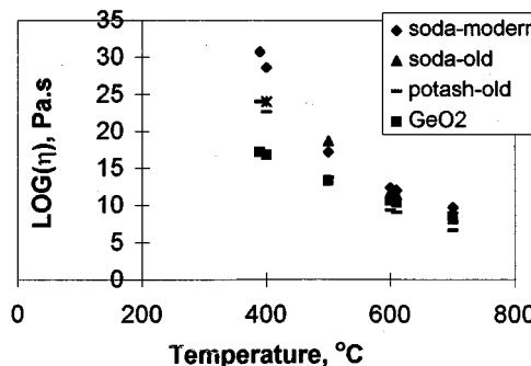
Fig. 1. Viscosity of different glasses as a function of temperature.
