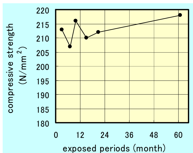
Figure 8. Time history records of compressive strength.
