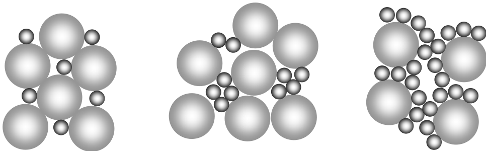
Figure 5.10 Schematization of possible agglomerating effects increasing the loosening effect. From left to right: without agglomeration, small particles agglomerating, small particles agglomerating to large particles.
