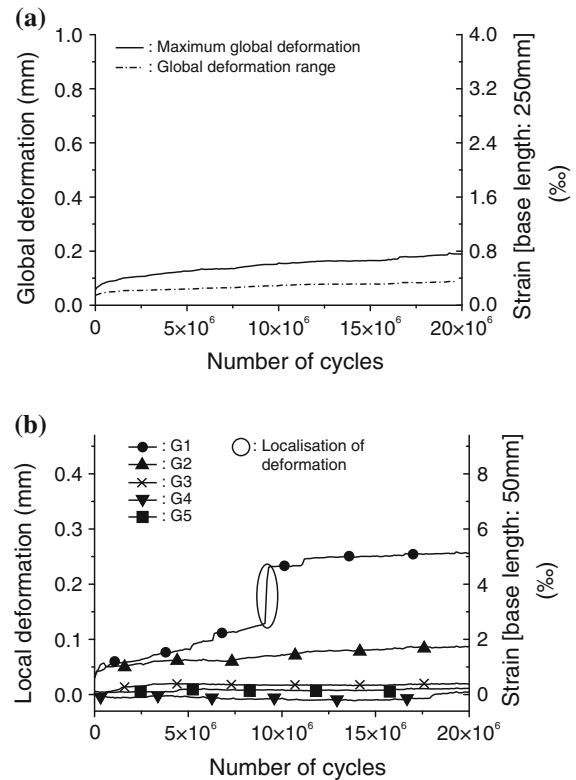
Fig. 8 Deformation growth curve of the S1-3_i test a global deformation and global deformation range, b local deformation
