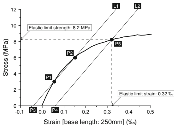
Fig. 3 Determination of elastic limit strength of UHPFRC
