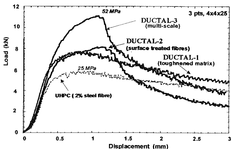
Figure 7 : New DUCTAL® materials : mechanical behaviour of concretes (3 pts bending)
