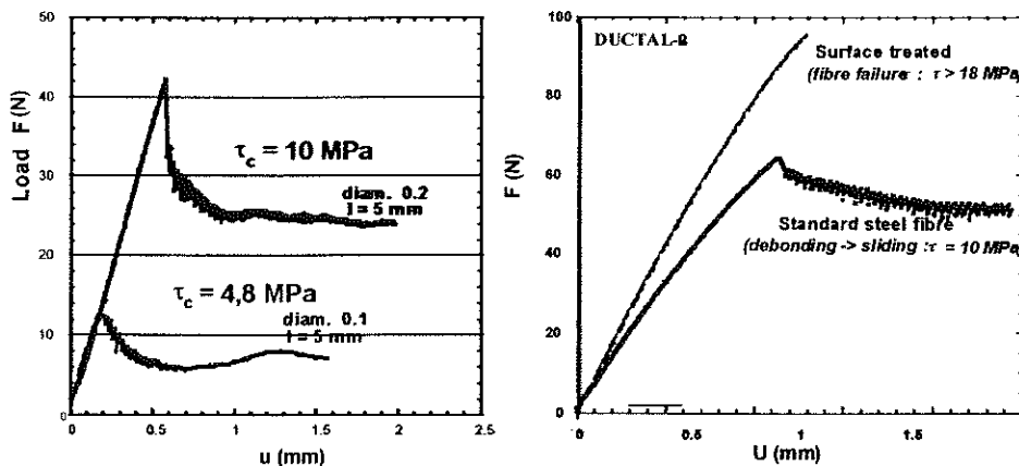
Figure 5 : Pull-out behaviour : a) effect of fibre diameter and embedded length b) effect of surface treatment (steel fibre)
