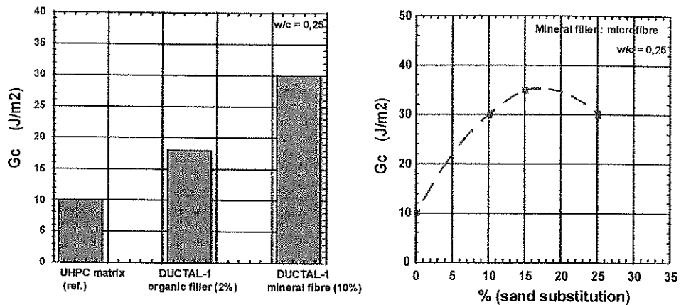
Figure 1 : Fracture toughness G_c of UHPC (ref.) and DUCTAL® concrete matrix.
