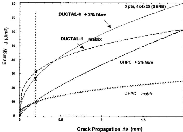
Figure 3 : Concrete damage resistance (J- \Delta a curve) : matrix and fibres contribution.
