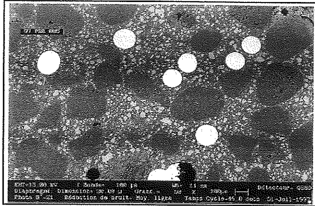
Figure 2 : Microstructure of DUCTAL ® concrete : fibre ( white circles ) and sand grains ( grey ellipse ) dispersed in a very dense cementitious paste.
