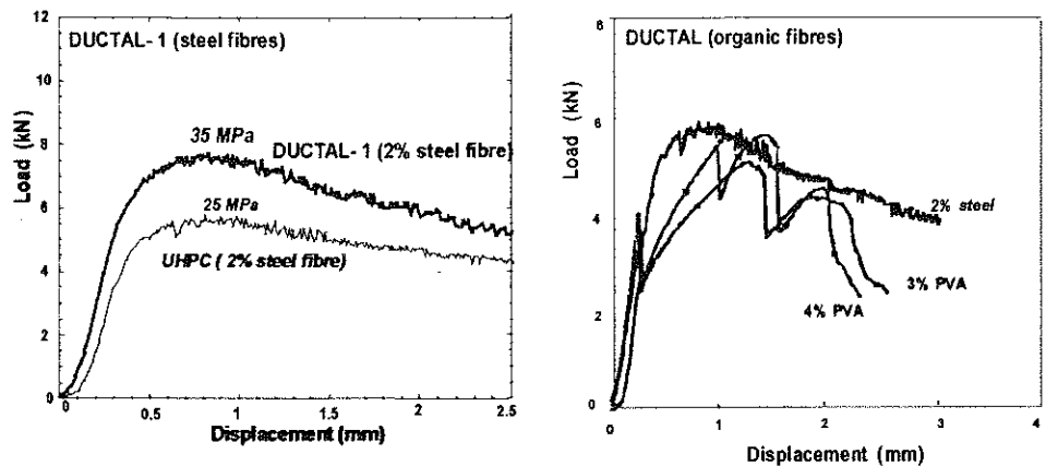
Figure 4 : Mechanical behaviour of fibre reinforced concrete (3 pts bending test)
