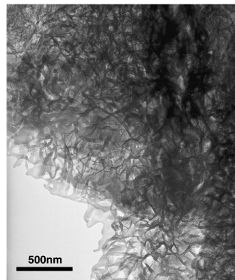
Fig. 23. Foil like C–S–H. From [59].
