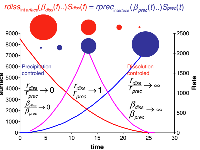
Fig. 5. This picture illustrates the dissolution-precipitation process in an ideal case; a spherical anhydrous particle dissolves to produce a hydrated spherical particle in the bulk solution. The surface of the dissolving particle decreases continuously and the surface of the hydrated particle increases continuously with the same law. For the equation to be satisfied, the dissolution interfacial rate must decrease and the interfacial precipitation rate must increase. This is achieved by the variations of the under and supersaturation respectively. The macroscopic hydration rate is at the maximum when the dissolving and precipitating surfaces are equal.
