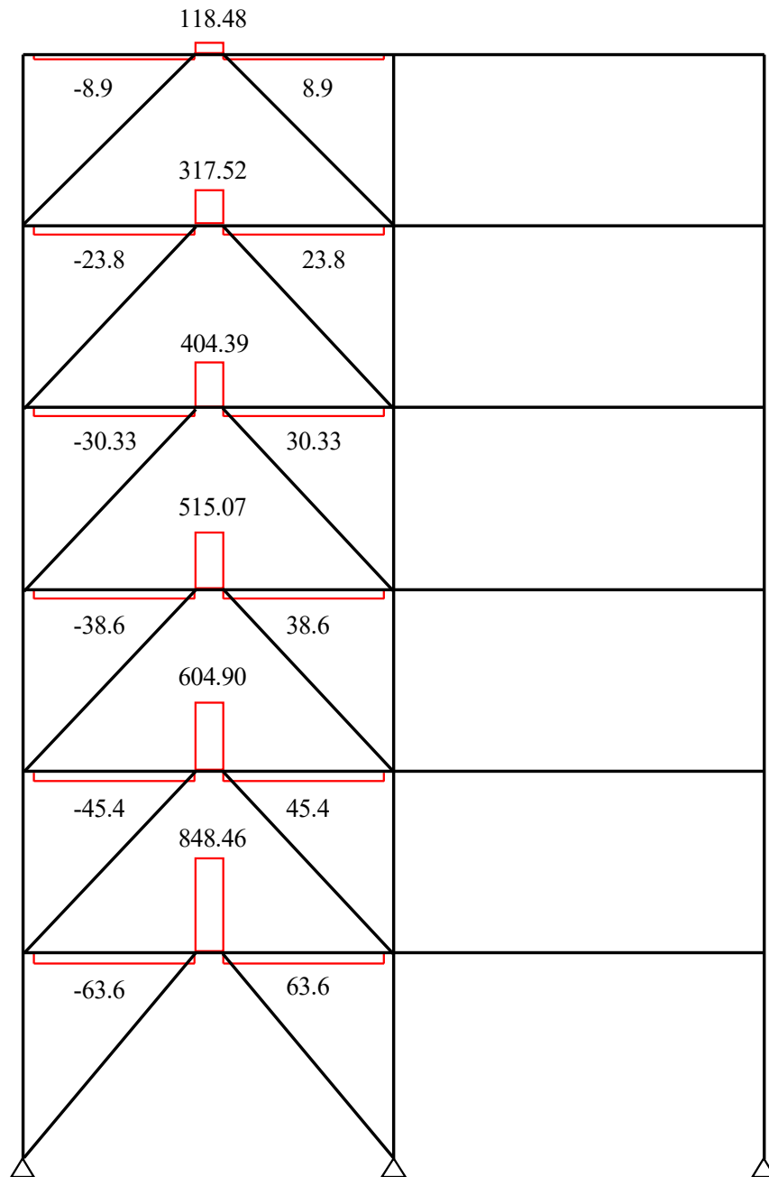
Figure 3. Shear force diagram for seismic loading (units in kN)
