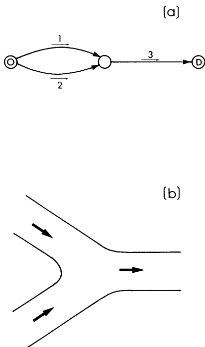
Figure 8.1 Network example with three links and one O-D pair: (a) the network representation; (b) the intersection represented by the middle node.
