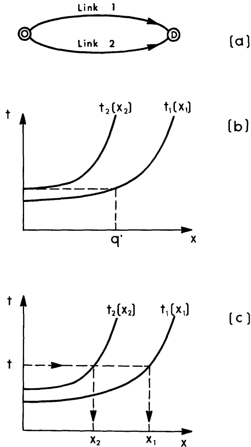
Figure 1.9 Equilibrium in a simple network: (a) a two-link network; (b) the two performance functions—if the flow is less than q' = x_1 + x_2 , it is assigned to link 1; (c) the travel time on both links is equal if the flow is higher than q' .
