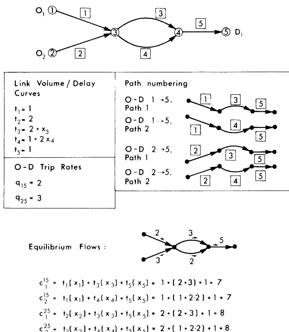
Figure 3.4 Equilibrium flows and path travel times in a network with two O-D pairs and five links.
