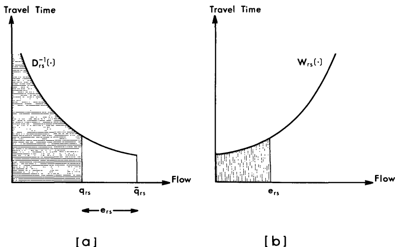
Figure 6.4 Inverse demand function and the associated argument-complementing function.
