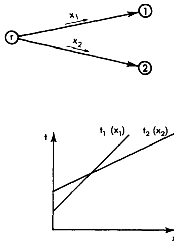
Figure 7.3 Network example with two O-D pairs and two links. The bottom figure shows the link performance functions.
