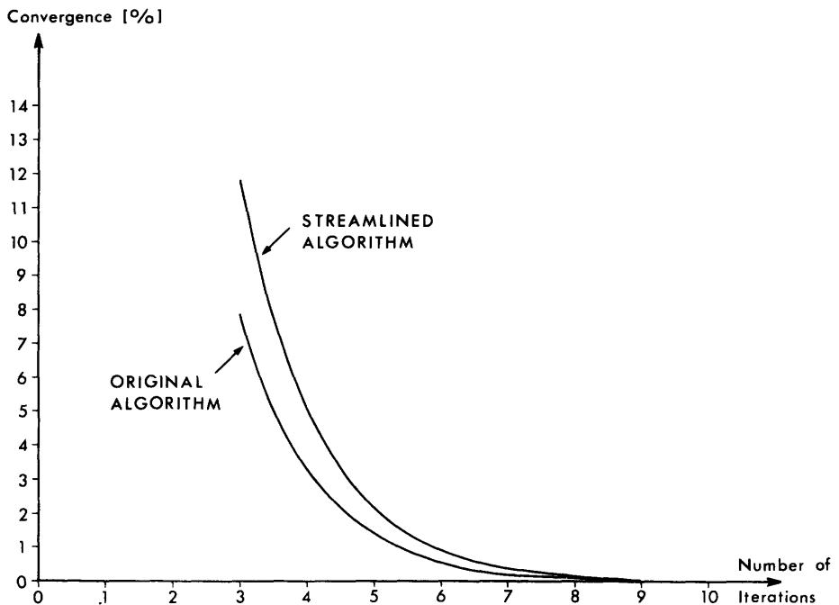
Figure 8.4 Convergence rates for the streamlined and the original diagonalization algorithm as a function of the number of iterations.
