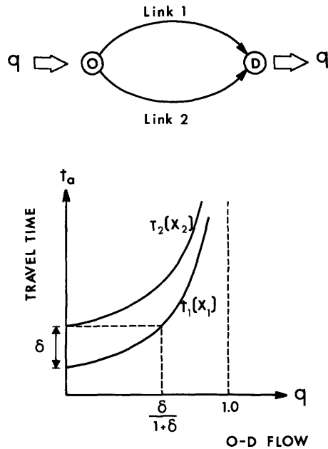
Figure 12.11 Simple network example with two links connecting one O-D pair. The bottom part shows the link performance functions.
