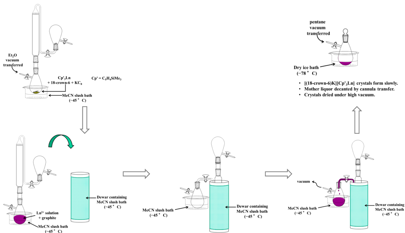
Figure 4. Procedure to make (\text{Cp}'_3\text{Ln})^- at -45\text{ }^\circ\text{C} by Schlenk techniques.
