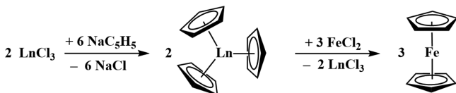
Scheme 1. Synthesis of \text{Cp}_3\text{Ln} and Reaction with \text{FeCl}_2 To Form Ferrocene
