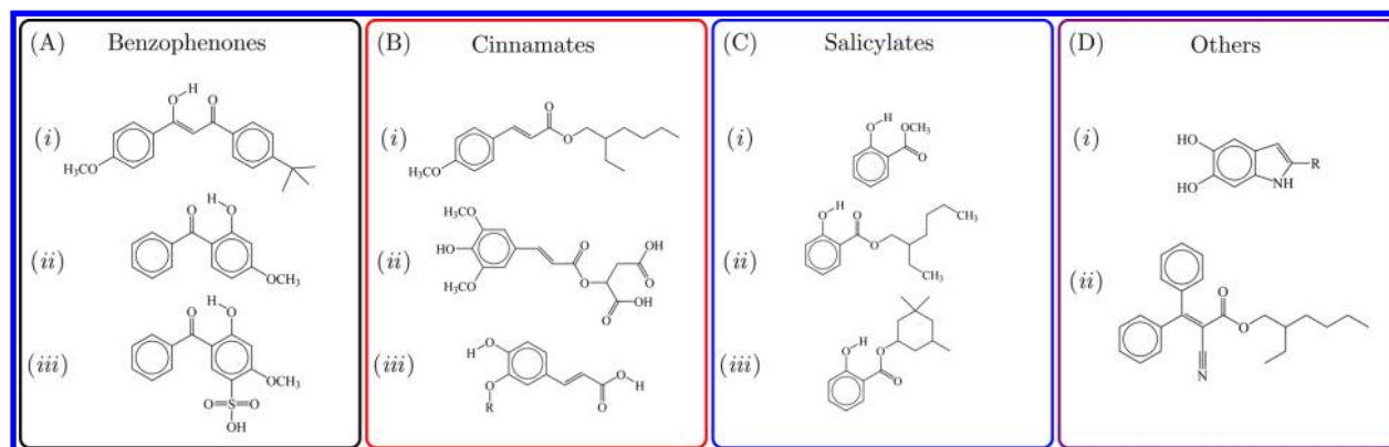
Figure 3. Common sunscreen organic filters. (A) Benzophenones: (i) avobenzone, (ii) oxybenzone, and (iii) sulisobenzene. (B) Cinnamates: (i) octyl methoxycinnamate, (ii) sinapoyl malate, and (iii) ferulic acid ( R = \text{CH}_3 ) and caffeic acid ( R = \text{H} ). (C) Salicylates: (i) methyl salicylate, (ii) octyl salicylate, and (iii) homomethyl salicylate. (D) Others: (i) 5,6-dihydroxyindole ( R = \text{H} ), 5,6-dihydroxyindole-2-carboxylic acid ( R = \text{CO}_2\text{H} ) and (ii) octocrylene.
