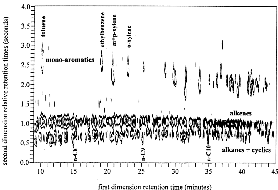
Fig. 12. GC \times GC analysis of cracked gasoline using column 1, 10 m DB-1 and column 2, 0.5 m OV1701 with an oven temperature programme of 2 °C/min from 30 to 200 °C [166].
