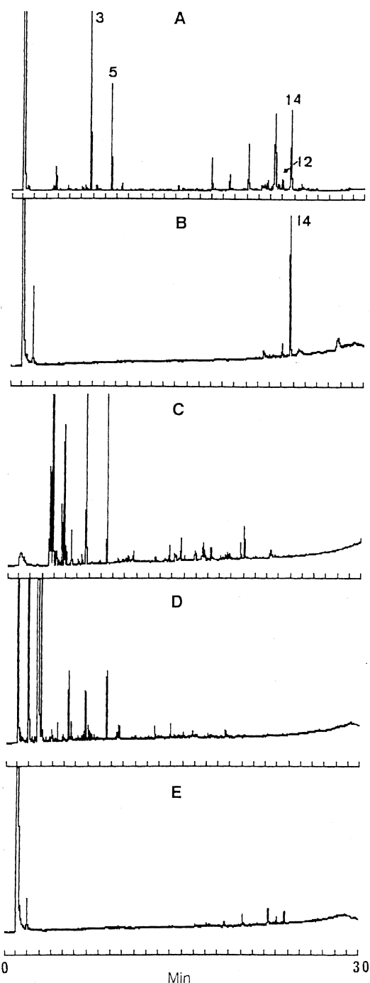
Fig. 1. Comparison of the gas chromatograms of extracts of feverfew obtained by different extraction methods. (A) SFE; (B) parthenolide standard; (C) steam distillation; (D) headspace analysis; (E) solvent extraction. Peaks: 3, camphor; 5 chrysanthemyl acetate; 12, dihydroparthenolide; 14, parthenolide [54].
