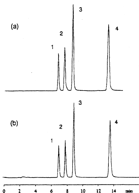
Fig. 5. Isocratic separation of a four-PAH mixture by (a) 1 µl loop injection and (b) fibre injection, 7 µm PDMS extraction for 30 min from 100 ppb of each compound spiked into water. Peaks: (1) fluoranthrene, (2) pyrene, (3) benz[a]anthracene and (4) benzo[a]pyrene [102].
