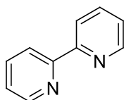
1,1'-bipyridine (bpy) -> ligand for transition metals
