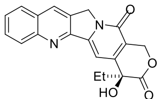
Camptothecin, Anti-cancer drug
