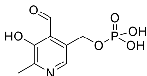
pyridoxal phosphate, co-enzyme, vitamine B6
