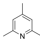
Collidine
