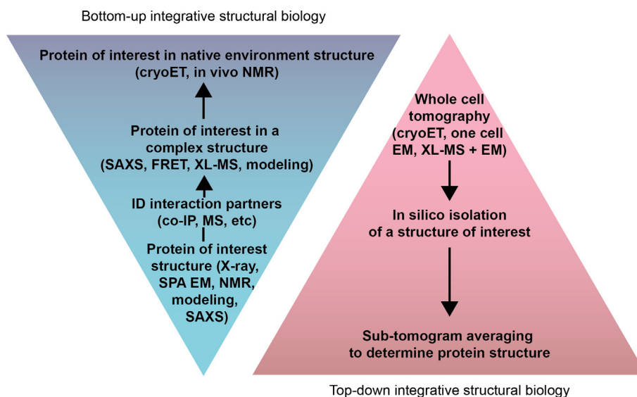
Fig. 4. Integrative structural biology flow chart. Traditional ISB is performed from bottom-up (blue triangle), starting with structures of individual components and building up to stable complexes and quinary interactions. With recent developments, ISB is beginning to be done from top-down starting from whole cell tomography providing the densities to map individual complexes (red triangle). (For interpretation of the references to colour in this figure legend, the reader is referred to the web version of this article.)
