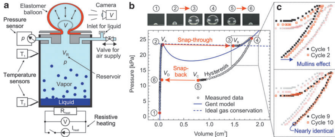
FIG. 2. (a) Schematic view of the experimental setup, including the clamped elastomer membrane after triggering the instability (Balloon state before the snap-through is indicated by a dotted curve), the camera for volume analysis, the pressure and temperature sensors, the resistive heating, the valve for supplying pressurized air, and the inlet to add liquid into the reservoir. (b) Measured data in the pressure-volume plane representing a full inflation and deflation cycle. The curve is traversed clockwise, starting and ending at state 1. Photos are taken at states 1 to 6. The snap-through and snap-back instabilities with the jumps in volume from states 2 to 3 and states 5 to 6 are indicated by arrows . The solid N-shaped curve is a theoretical fit according to the Gent model in Equations (1) and (2), and the dashed curve represents the ideal-gas conservation law for the enclosed air from Equation (4). (c) The detailed inset shows the change in behavior from the first to the 10th inflation/deflation cycle due to change in material properties.
