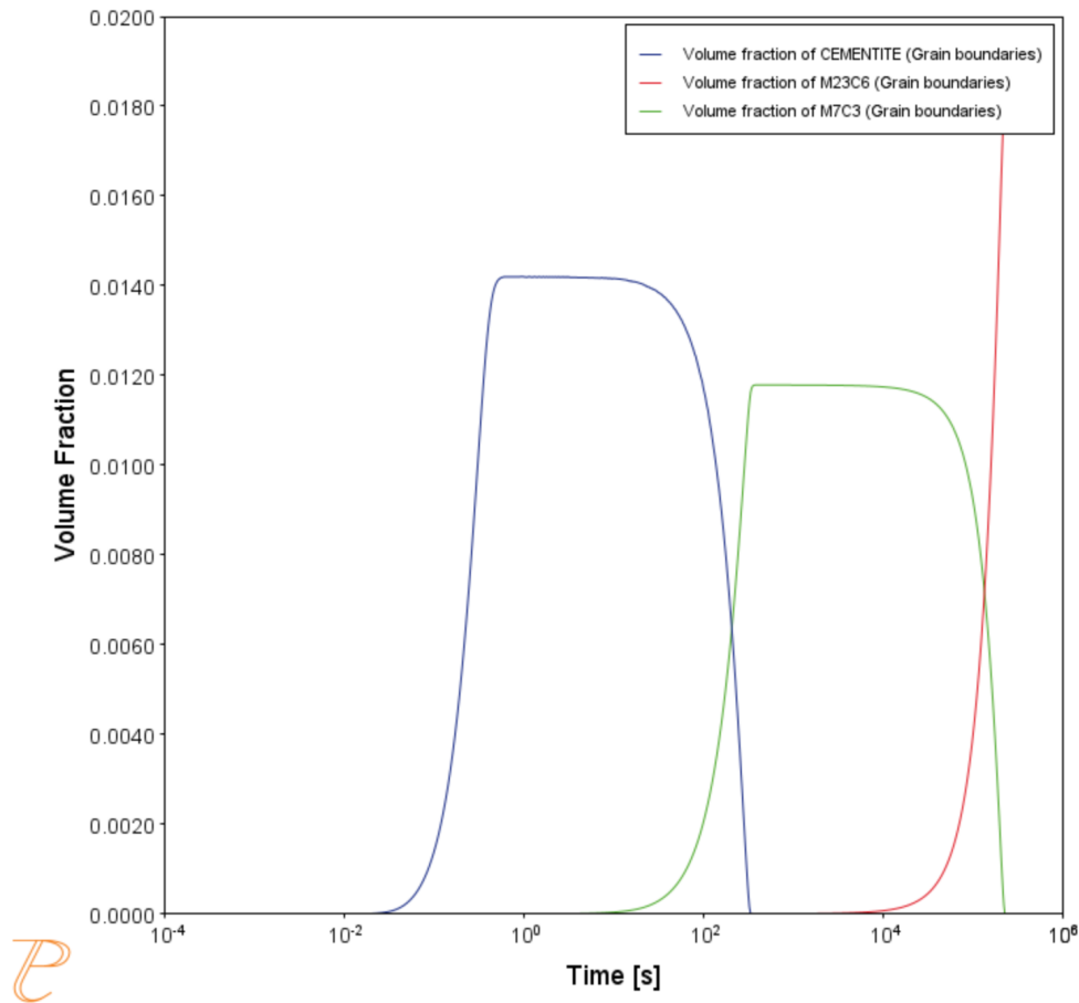
Figure 16: The Precipitation Calculator is used to do an isothermal calculation of the three phases (cementite, M23C6 and M7C3) where cementite and M7C3 are metastable phases.
