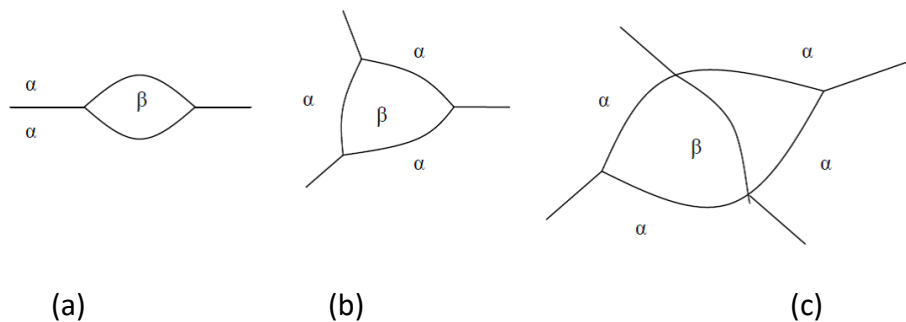
Figure 6: Non-spherical particles ( \beta ) that precipitate at grain boundaries of matrix phase ( \alpha ) (a) grain boundary (two-grain junction) (b) grain edge (three-grain junction) (c) grain corners (four-grain junction). Images taken from Zang [2004].
