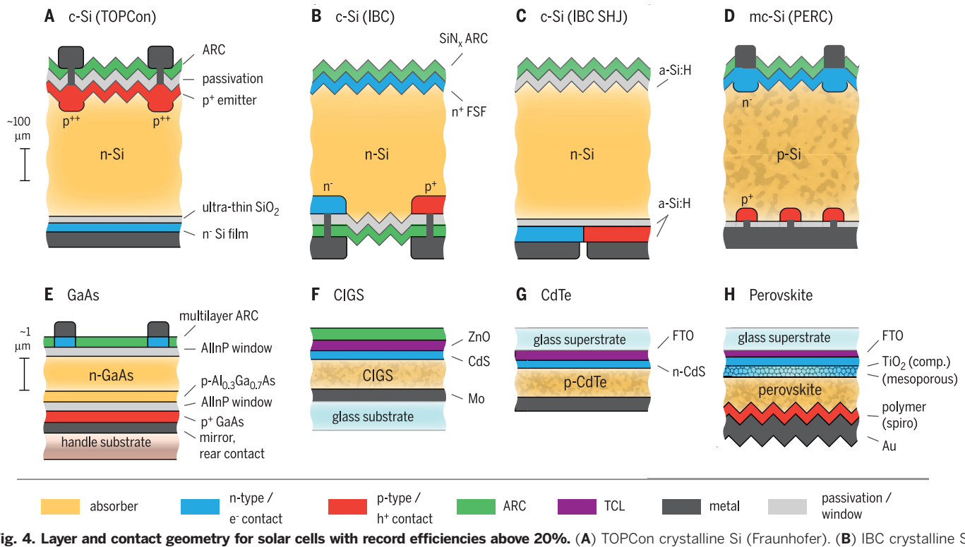
Fig. 4. Layer and contact geometry for solar cells with record efficiencies above 20%. (A) TOPCon crystalline Si (Fraunhofer). (B) IBC crystalline Si (SunPower). (C) Heterojunction IBC crystalline Si (Panasonic). (D) Multicrystalline Si (Trina Solar). (E) GaAs thin film (Alta Devices). (F) CIGS thin film (ZSW Stuttgart). (G) CdTe thin film (First Solar). (H) Perovskite thin film (KRICT). For industrial cells, the exact geometry is not publicly available.
