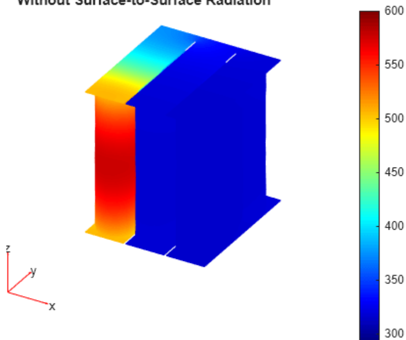
Temperature Distribution in Cells and Connectors Without Surface-to-Surface Radiation
