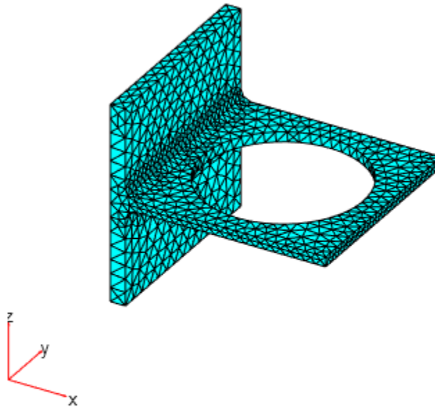
Mesh with Quadratic Tetrahedral Elements
