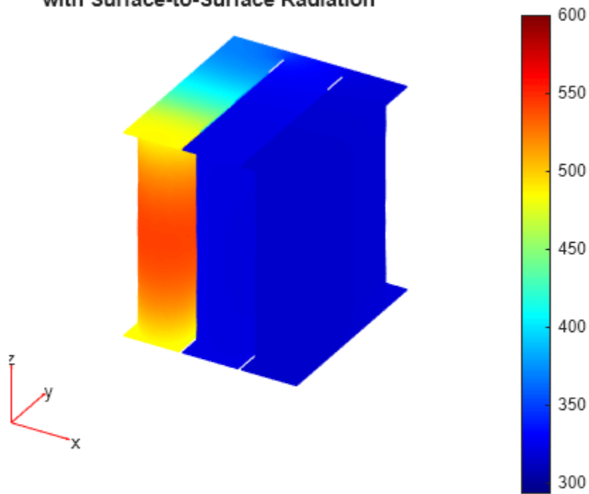
Temperature Distribution in Cells and Connectors with Surface-to-Surface Radiation
