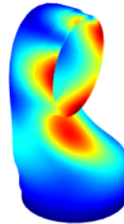
Flexible Mode 6 Frequency = 8001.39 Hz
