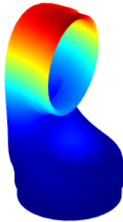
Flexible Mode 1 Frequency = 1933.67 Hz
