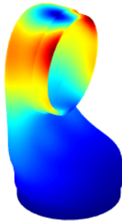
Flexible Mode 4 Frequency = 5098.99 Hz
