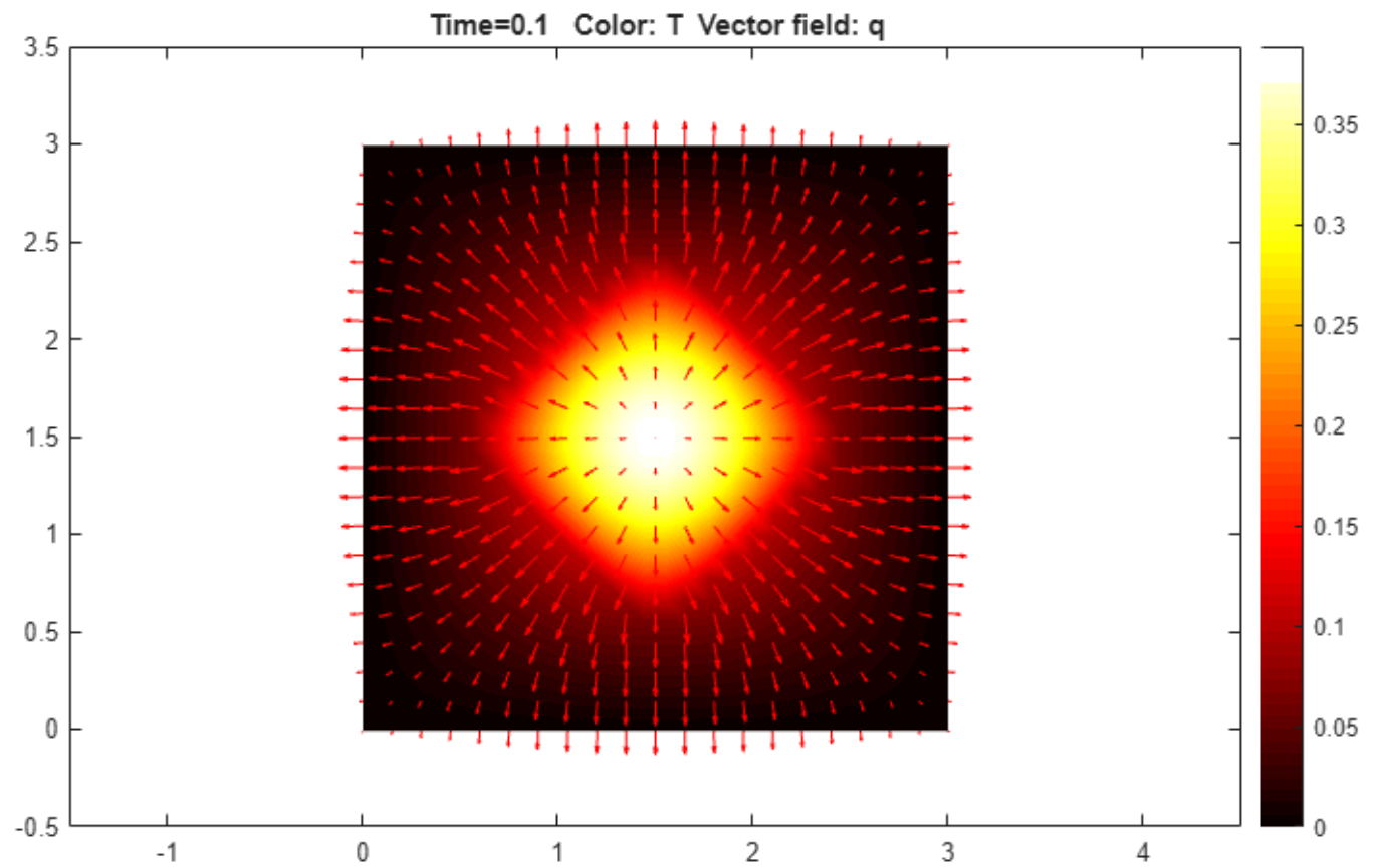
Temperature and Heat Flux
