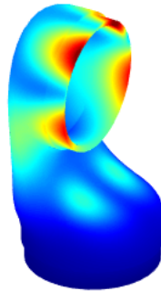
Flexible Mode 5 Frequency = 7754.5 Hz
