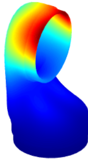
Flexible Mode 2 Frequency = 2636.48 Hz
