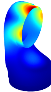
Flexible Mode 3 Frequency = 4947.05 Hz
