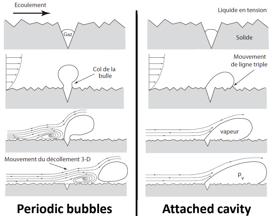
Mechanism of cavitation inception
