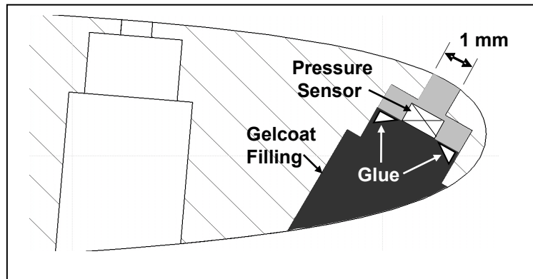
Sensors are flush-mounted on the suction side
