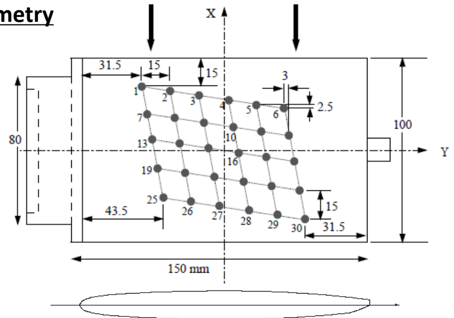
Sensors are flush-mounted on the suction side
