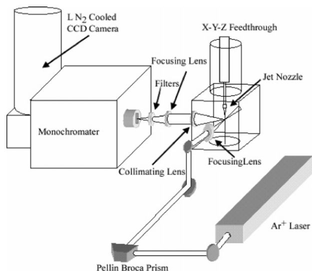
Figure 1. Schematic view of experimental apparatus.
