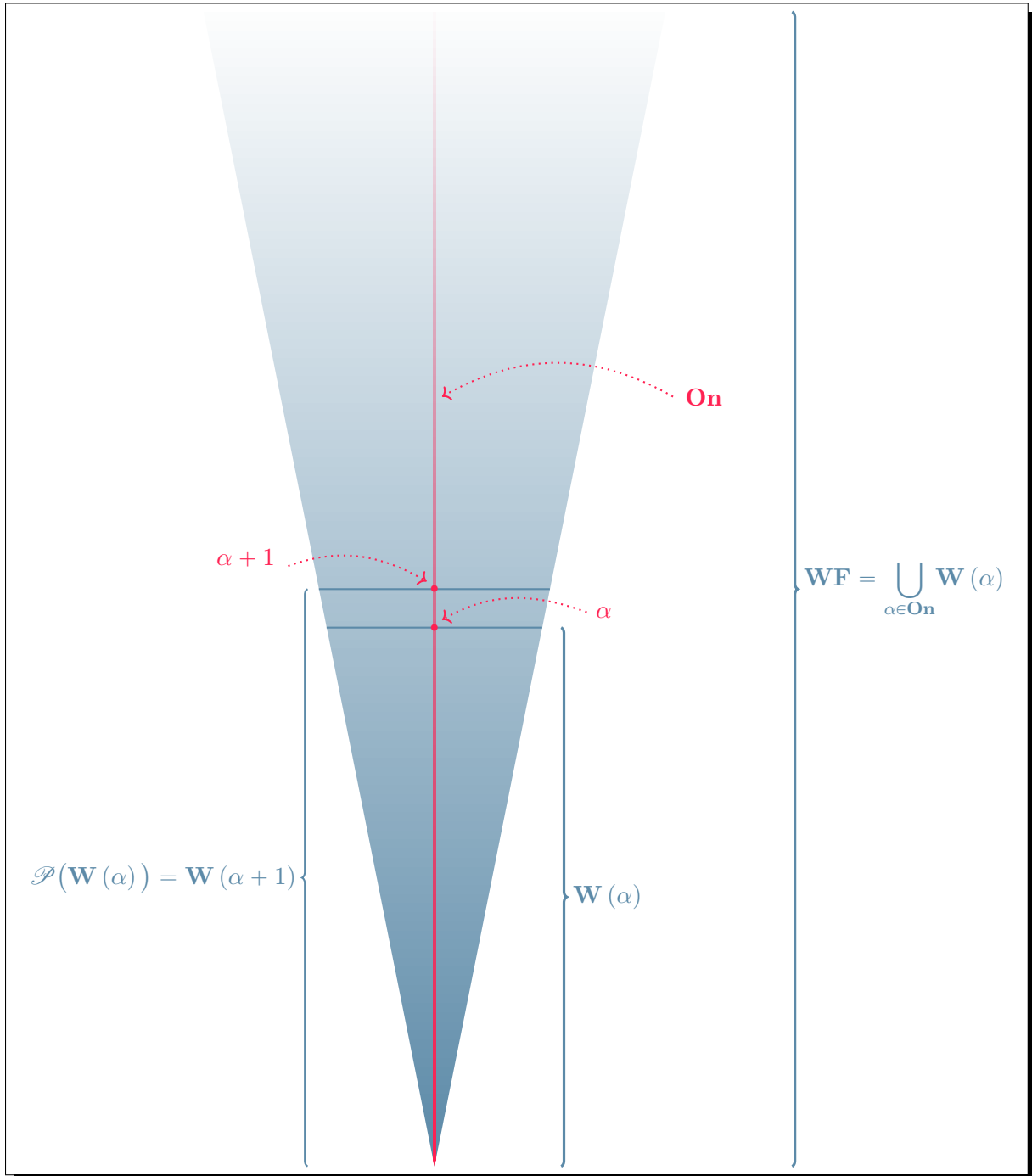
Figure 5.1: The Class of Well-Founded Sets \mathbf{WF} = \bigcup_{\alpha \in \text{On}} \mathbf{W}(\alpha) .
