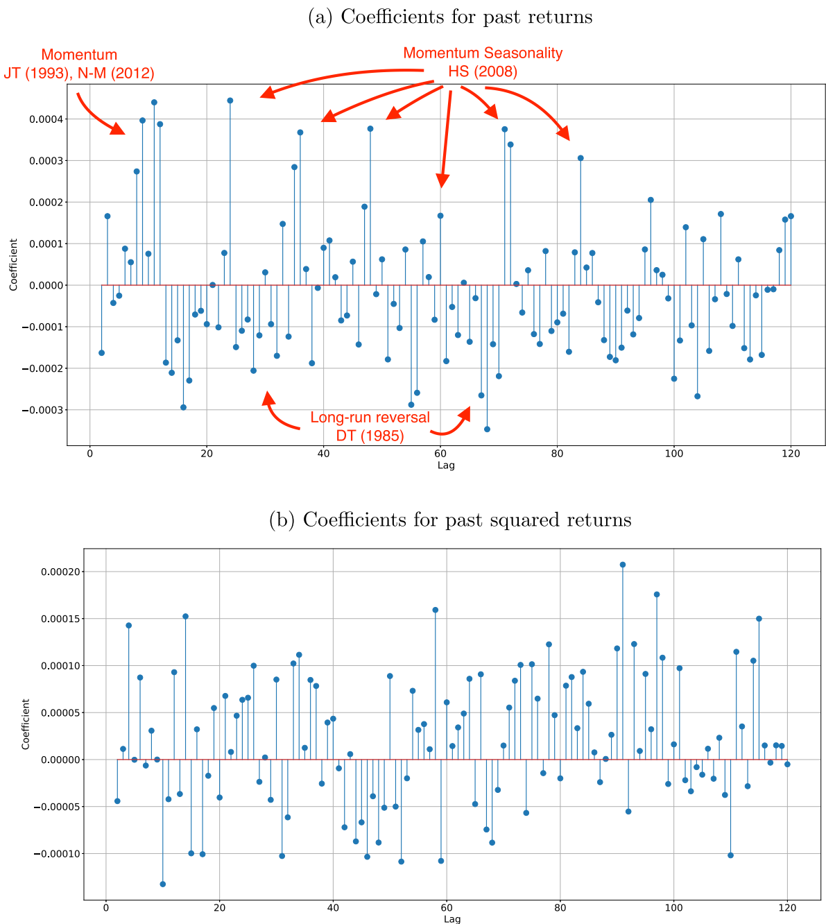
Fig. 7. Ridge regression coefficient estimates.
