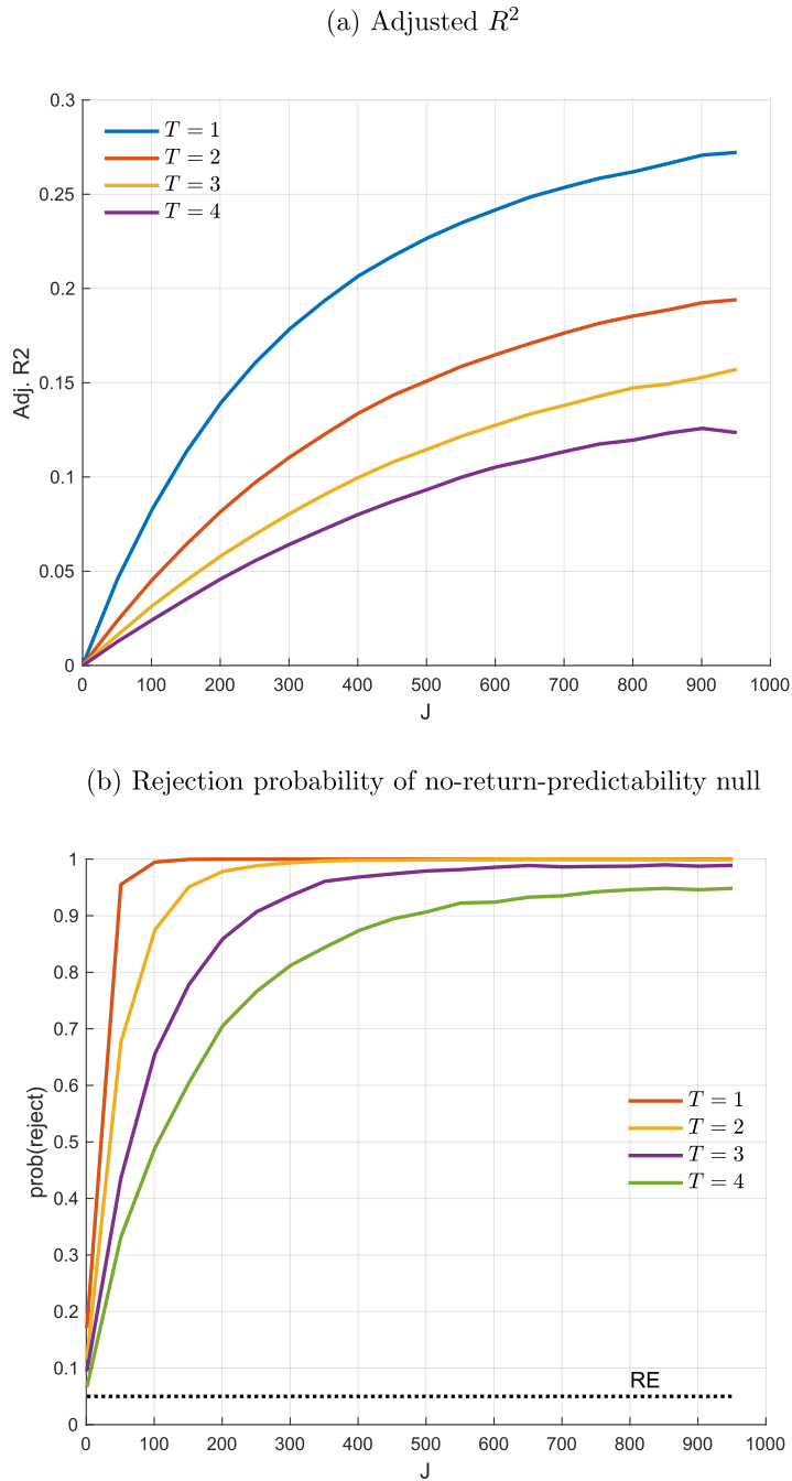
Fig. 3. In-sample return predictability tests. Based on cross-sectional regressions with N = 1000 assets and J predictor variables, predicting the last return in a sample of size T + 1 and where investors have learned about \mathbf{g} from a sample of size T . The test in panel (b) is a joint \chi^2 -test using all J predictors. It has an asymptotic 5% rejection probability under the rational expectations null hypothesis (where investors know \mathbf{g} ). The solid lines show the actual rejection probabilities when this test is applied in a setting where Bayesian investors with an objectively correct informative prior estimate \mathbf{g} .
