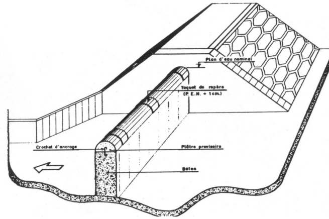
Security weir
