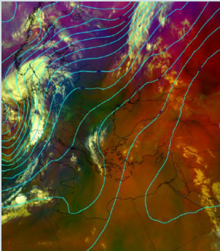
Very hot and dry air masses also appear as reddish colour tones in the Airmass RGB as can be seen in the above image over south-eastern Europe on 8 August 2017 at 18:00 UTC. This is not an indication of ongoing cyclogenesis or subsidence.
