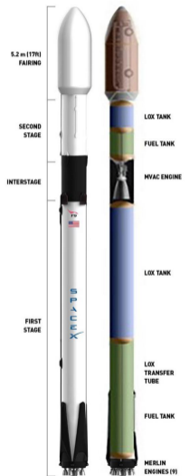
Figure 2-1: Falcon 9 overview SpaceX
