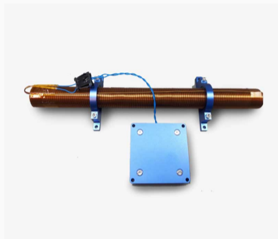
Magnetic Torquer MTQ800, AAC Clyde Space
