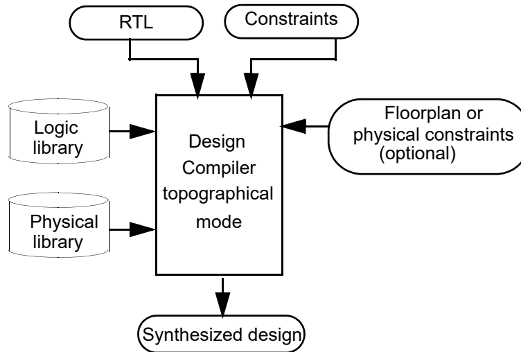
Figure 143 Inputs and Outputs in Design Compiler Topographical Mode
