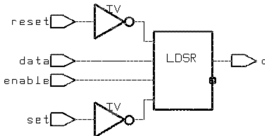
Figure 182 Synthesized Design for a D Latch With Asynchronous Set and Reset
