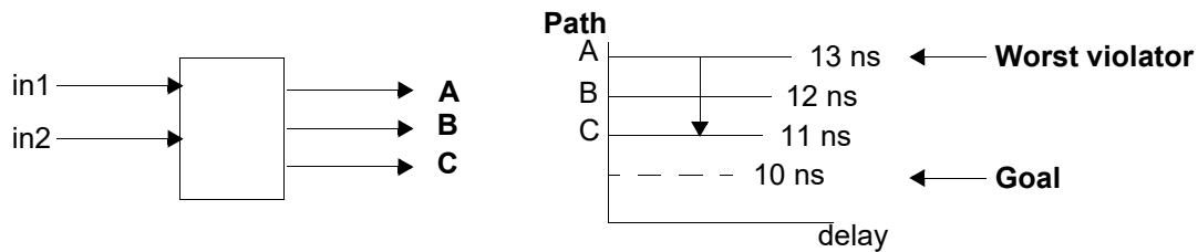
Figure 82 Critical Range Example
