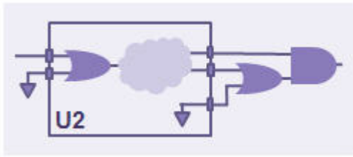
Figure 89 Design Before Boundary Optimization
