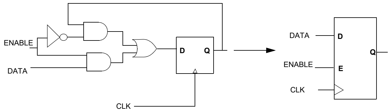
Figure 77 Sequential Optimization
