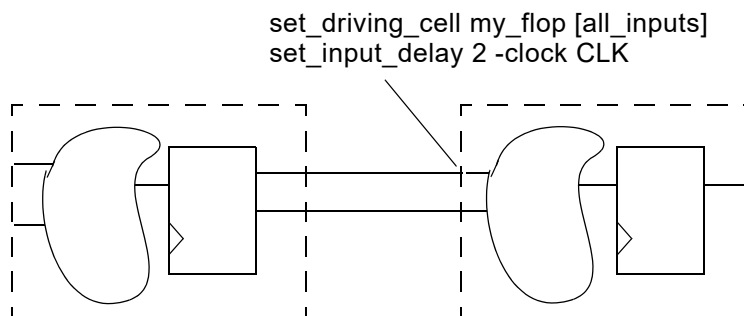
Figure 12 Registering All Outputs
