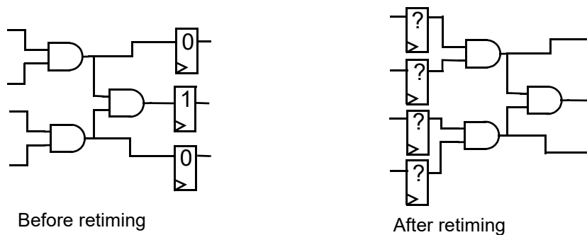
Figure 137 Impossible Backward Justification Example
