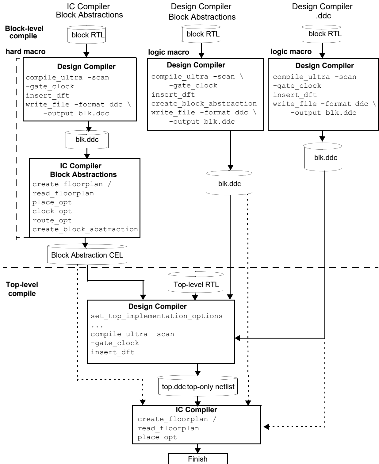
Figure 144 Overview of the Hierarchical Flow for Designs Containing Block Abstractions
