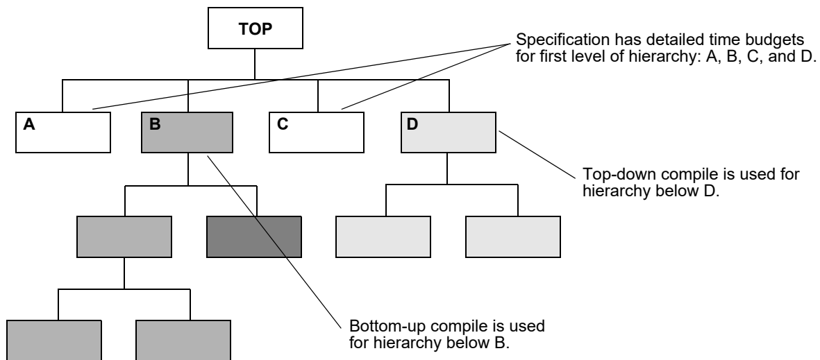
Figure 69 Mixing Compilation Strategies
