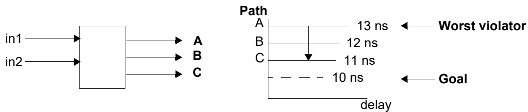
Figure 34 Critical Range Example
