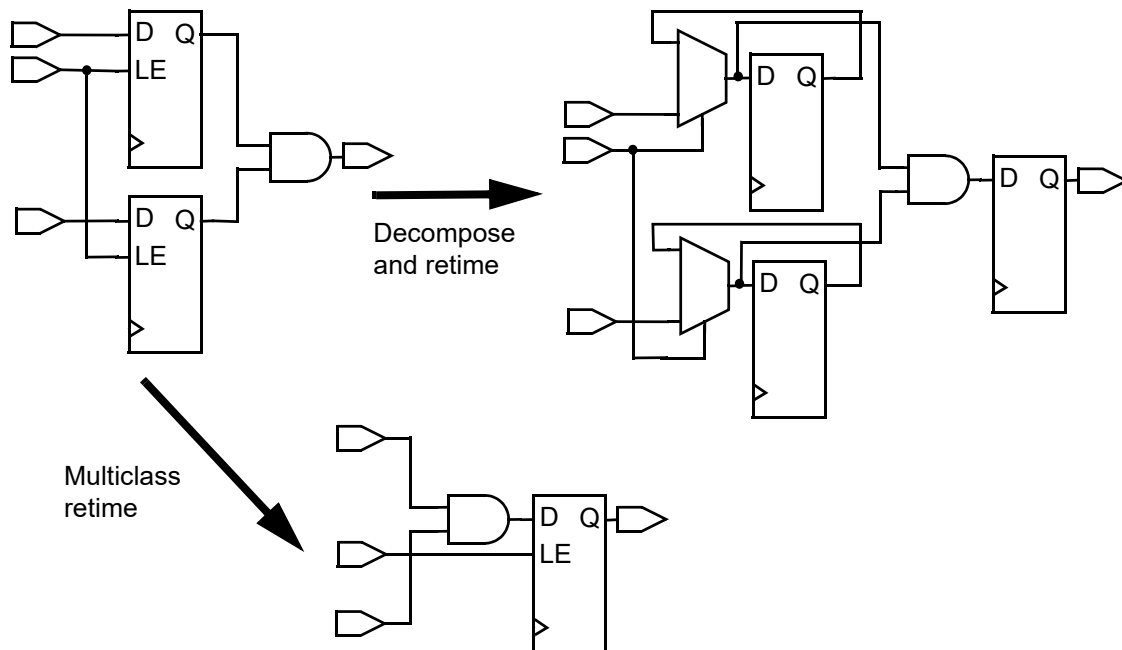
Figure 136 Reduced Area Through Multiclass Retiming
