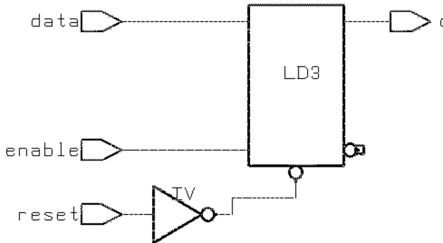
Figure 181 Synthesized Design for a D Latch With Asynchronous Reset
