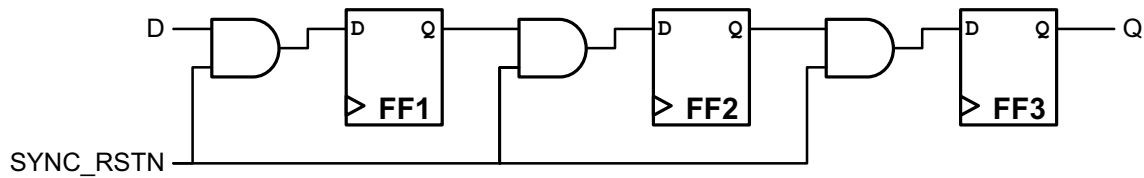
Figure 116 Example of Shift Register Identification with Synchronous Reset
