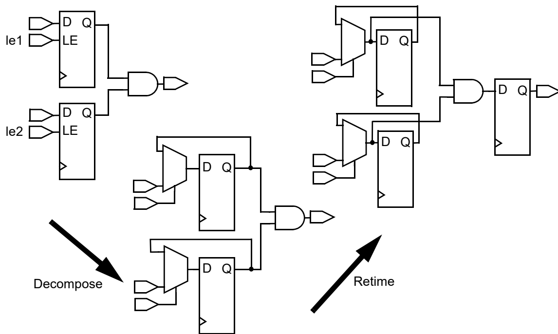
Figure 134 Forward Retiming of Decomposed Cells With Load Enable
