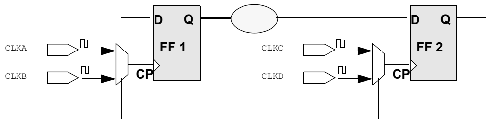
Figure 87 Multiple Clocks per Register
