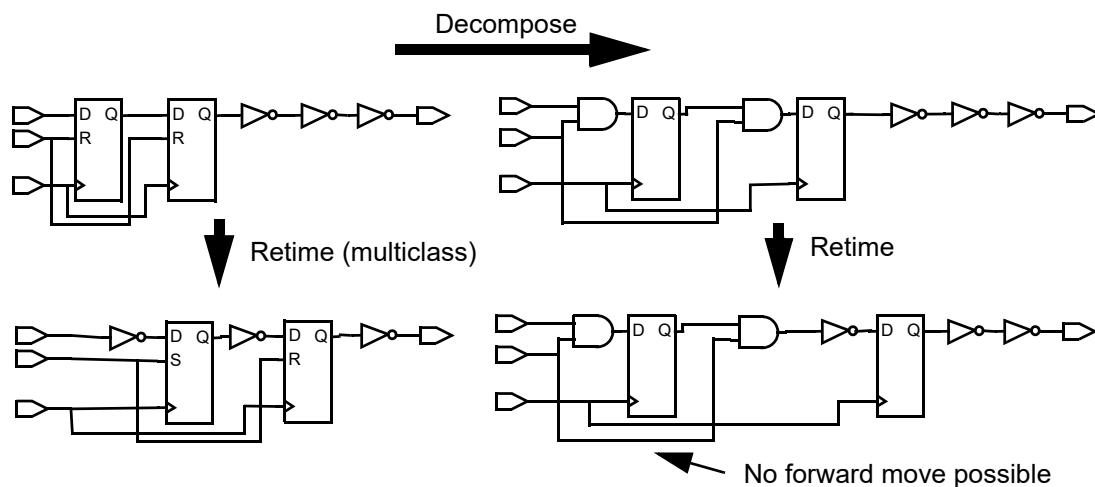
Figure 139 Reduced Mobility After Decomposition
