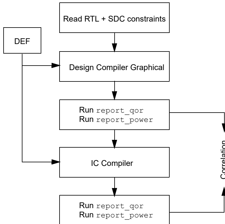
Figure 150 Correlation Measurement Between Design Compiler and IC Compiler
