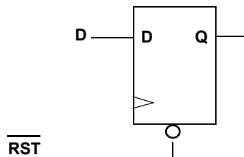
Figure 110 Mapping To Registers With and Without Synchronous Reset Pins
