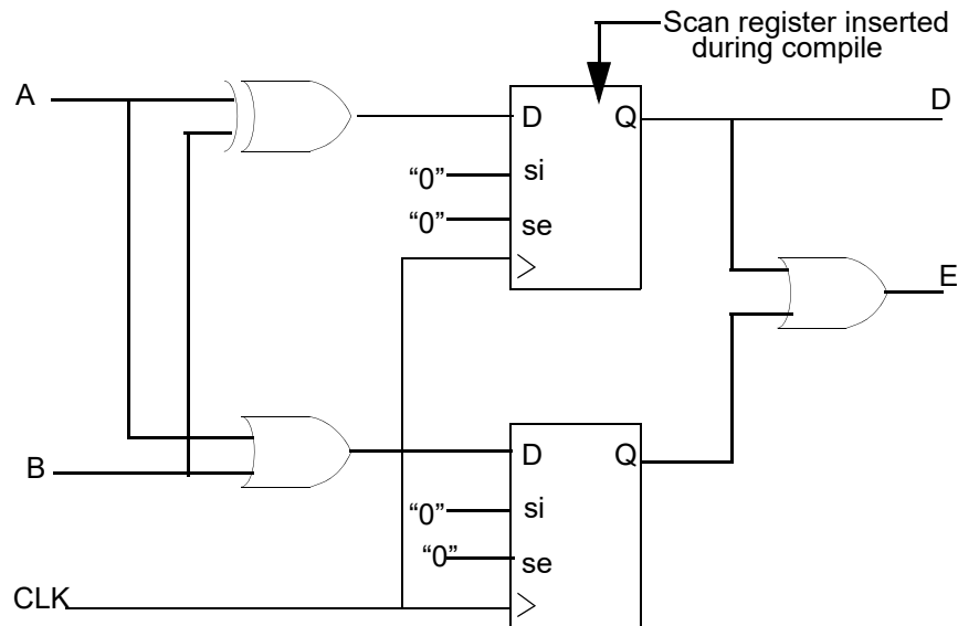
Figure 112 Result of Test-Ready Compile
