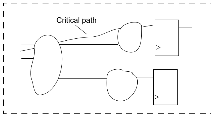
Figure 11 Keeping Related Logic in the Same Block
