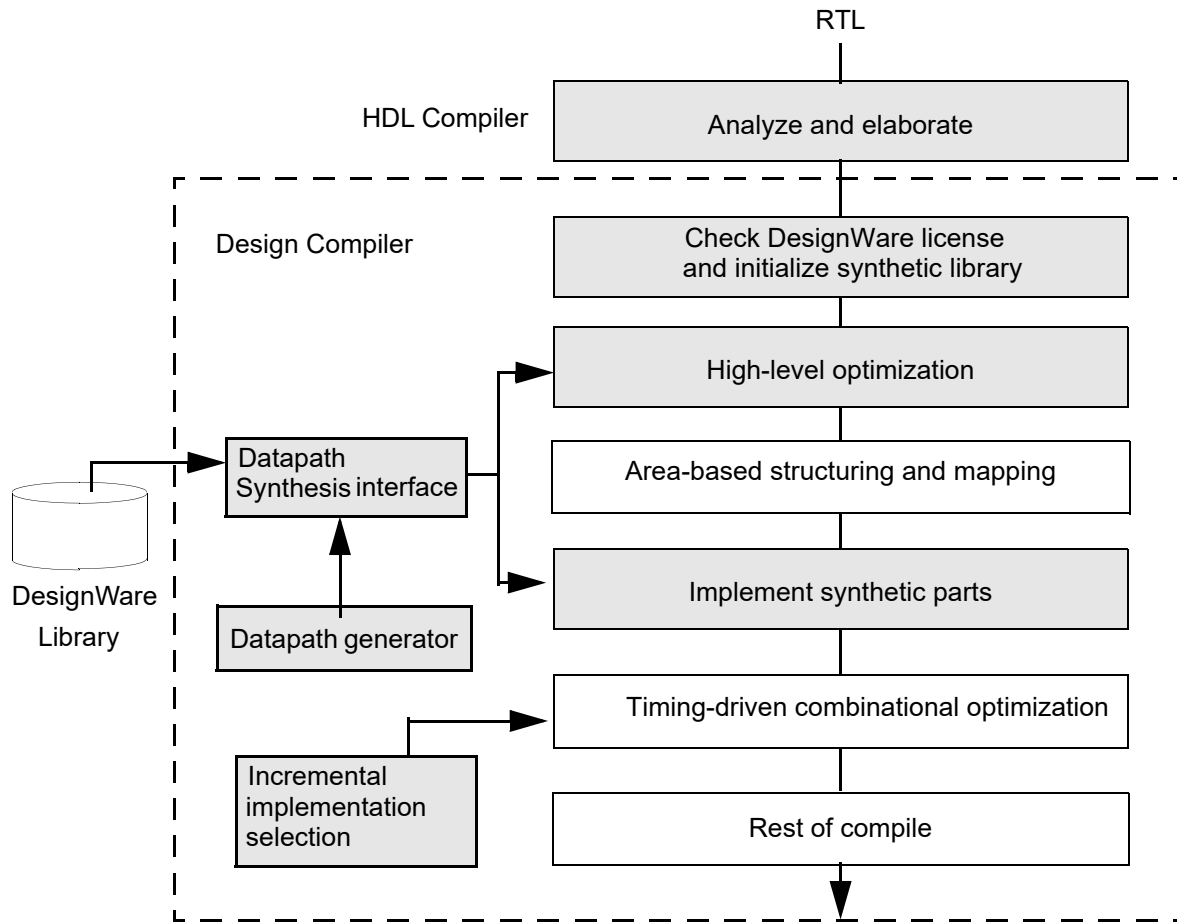
Figure 93 Optimization of Arithmetic Expressions
