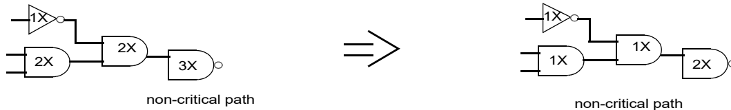
Figure 142 Example of Downsizing Cells During Area Recovery
