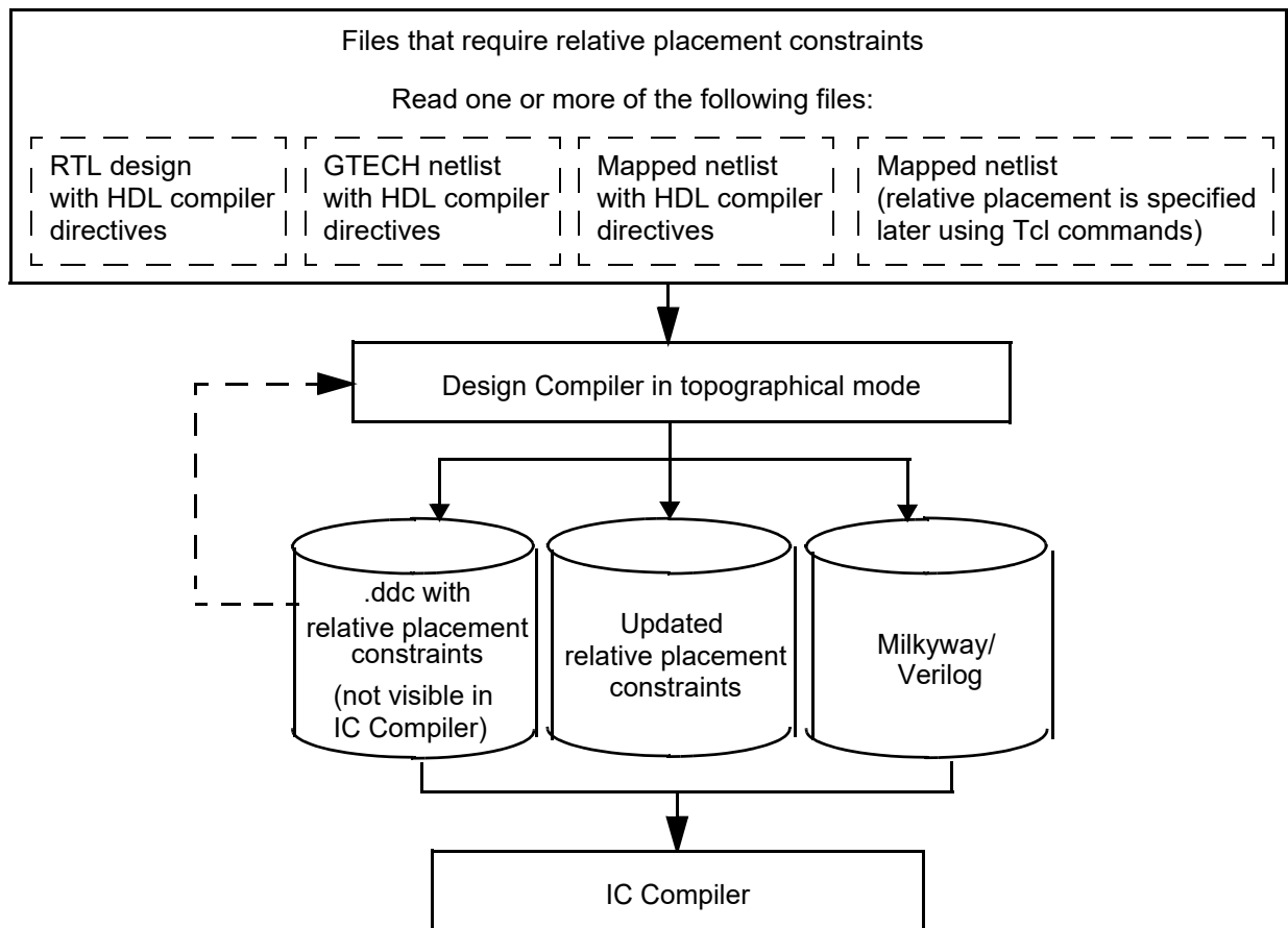
Figure 57 Relative Placement Flow
