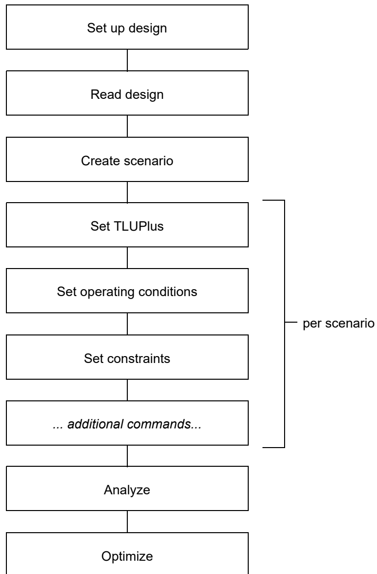
Figure 158 Basic Multimode Flow
