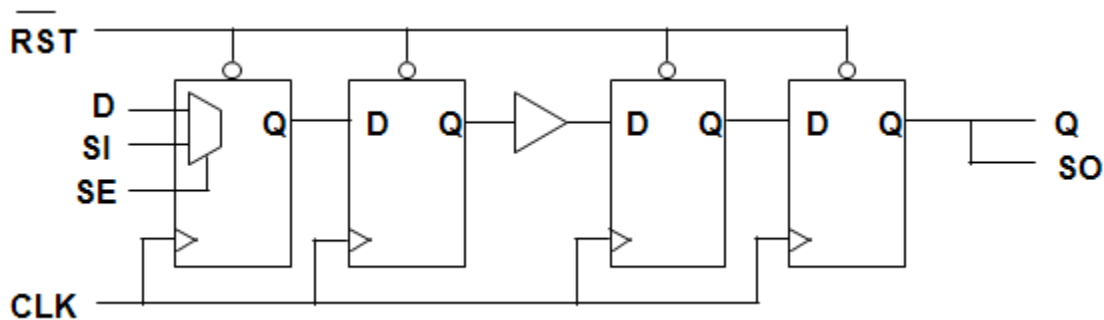
Figure 115 Example of Shift Register Identification
