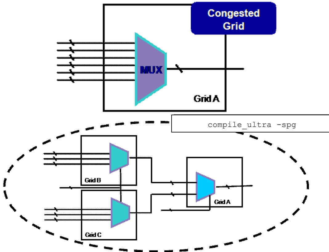
Figure 147 Optimizing RTL Structures to Minimize Congestion
