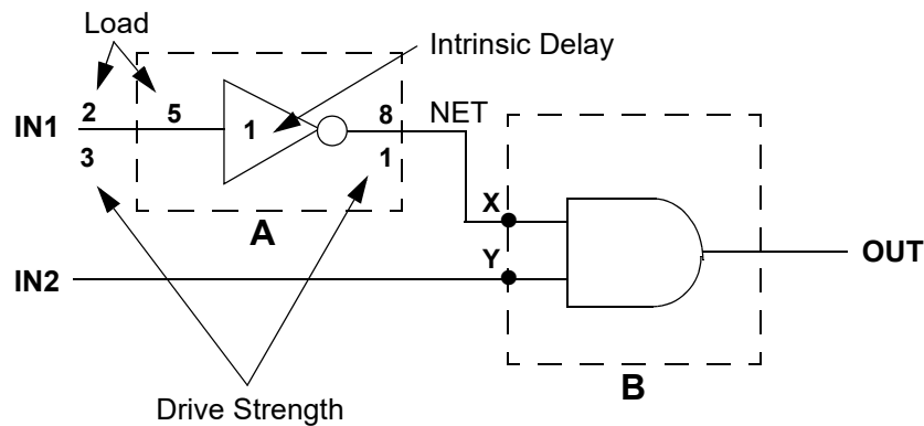
Figure 41 Design With Annotations for Timing Calculations
