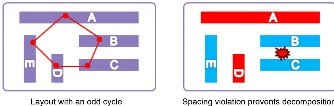
Figure 163 Odd-Cycle Violation
