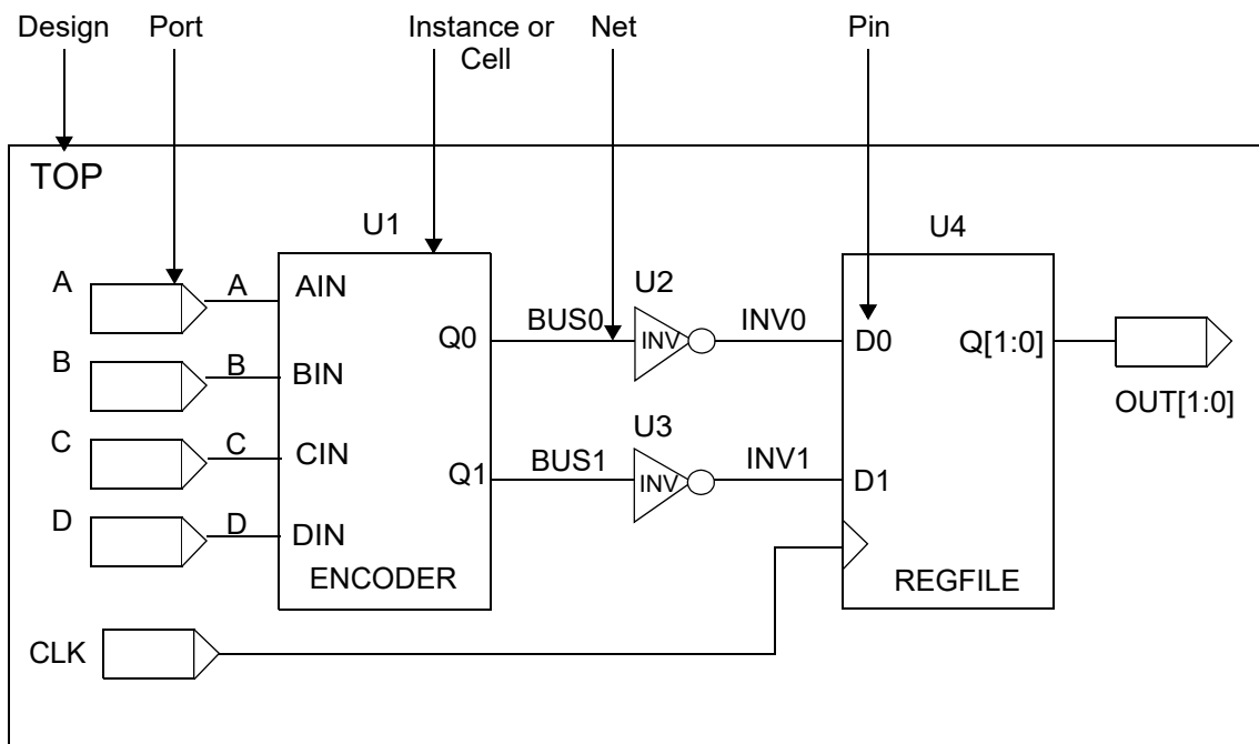
Figure 3 Design Objects
