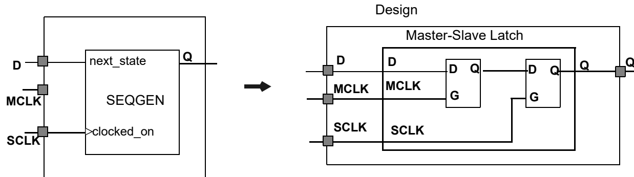
Figure 88 Generic Cell and Master-Slave Latch After Compilation
