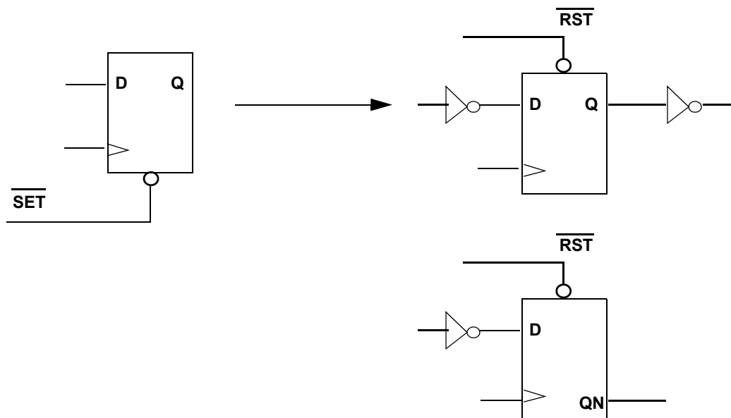
Figure 107 Output Inversion Transformations
