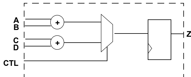
Figure 14 Keeping Sharable Resources in the Same Process
