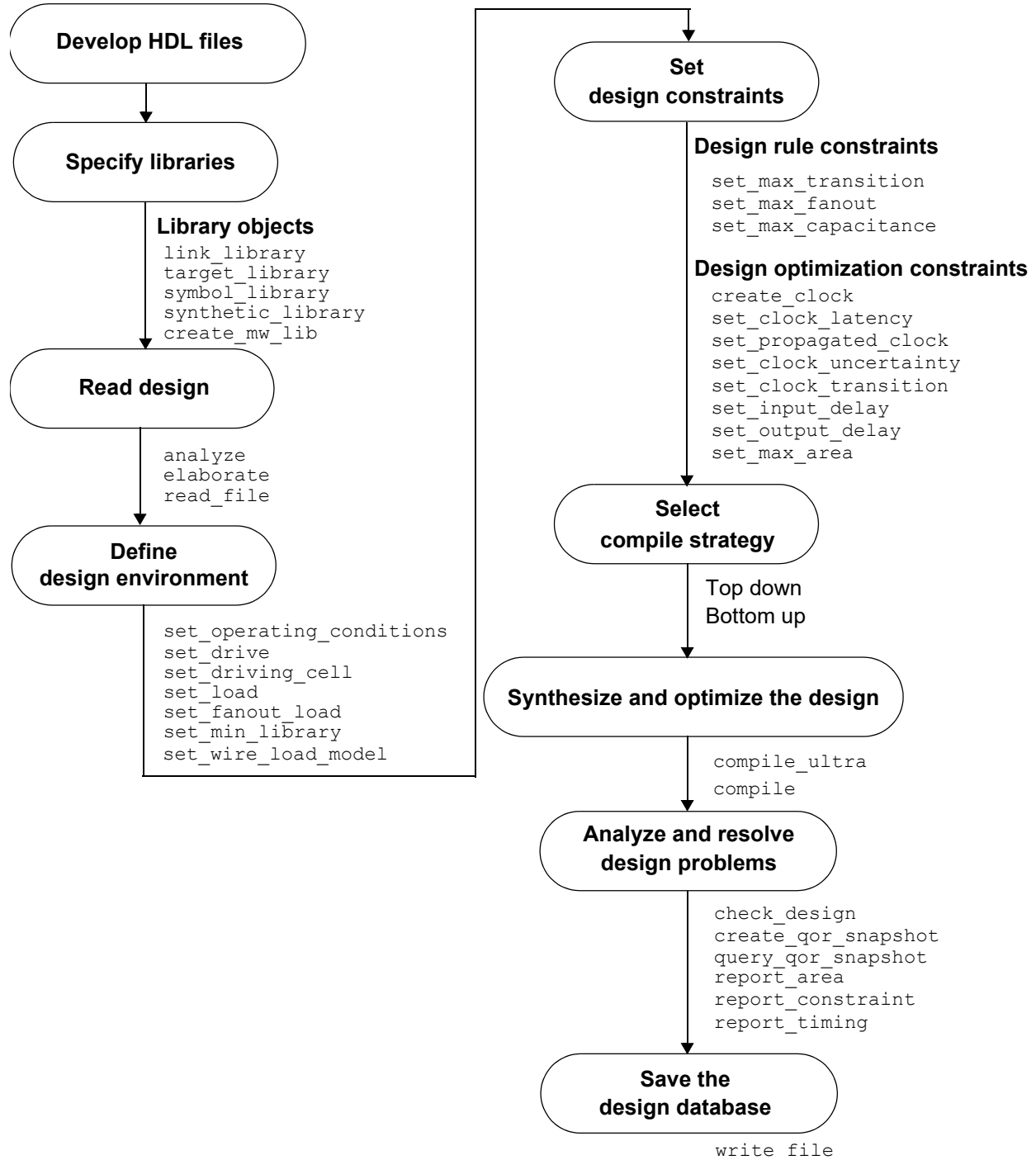
Figure 6 Synthesis Flow
