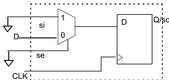
Figure 111 Example of a Scan Register Used During Test-Ready Compile
