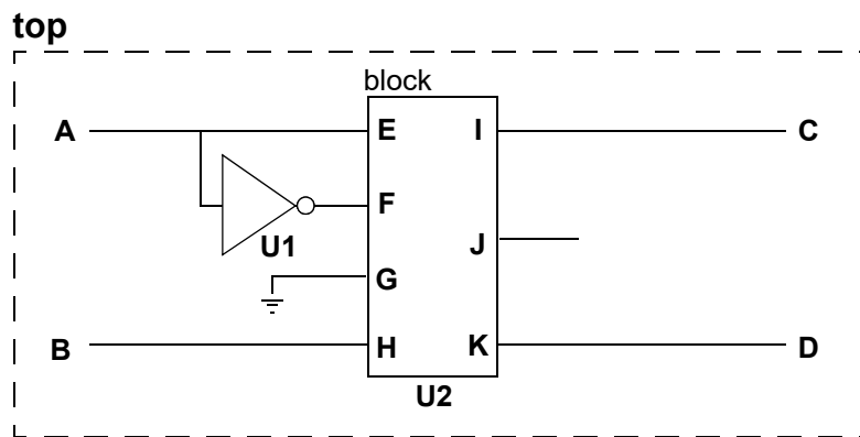
Figure 44 Characterizing Port Connection Attributes
