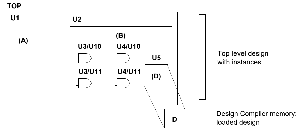
Figure 73 Ungroup Results
