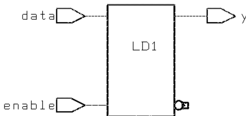
Figure 180 Synthesized Design for a D Latch
