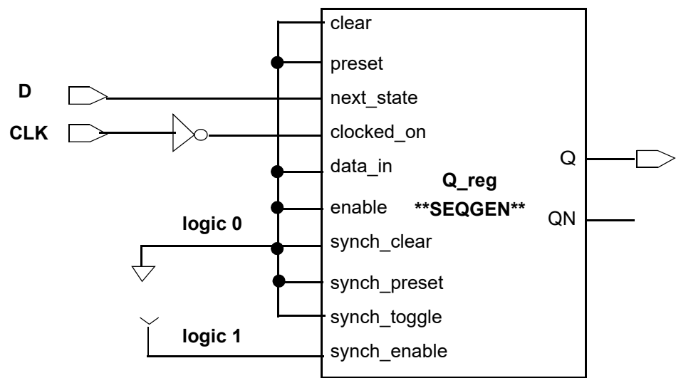
Figure 108 SEQGEN Created by HDL Compiler
