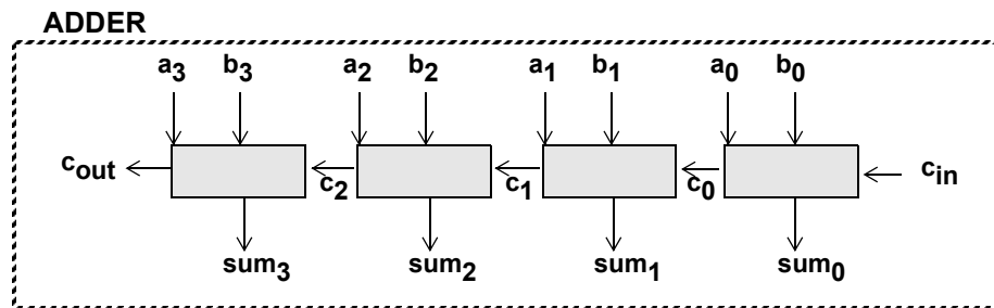
Figure 68 Hierarchical Design
