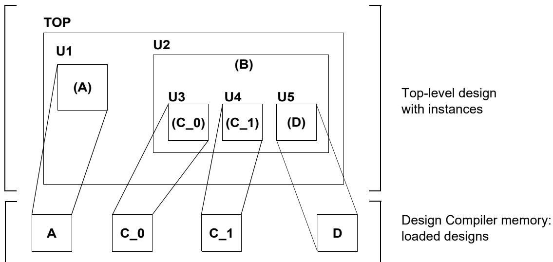
Figure 71 Uniquify Results
