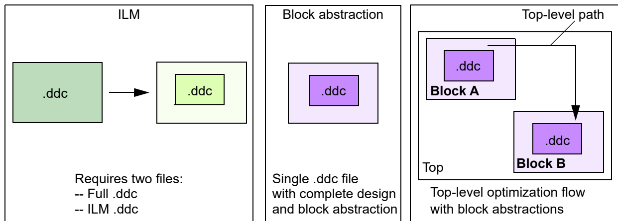
Figure 168 ILM and Block Abstraction Comparison
