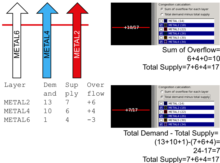
Figure 148 Congestion Example
