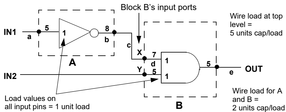
Figure 40 Loads After Characterization
