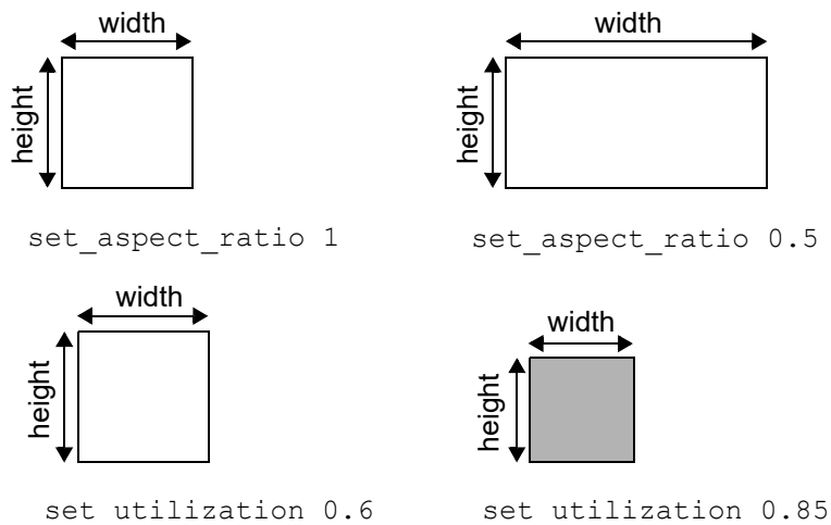
Figure 48 Using the set_aspect_ratio and set_utilization Commands
