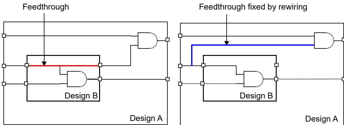
Figure 85 Feedthrough Fixed By Rewiring Up Through the Hierarchy
