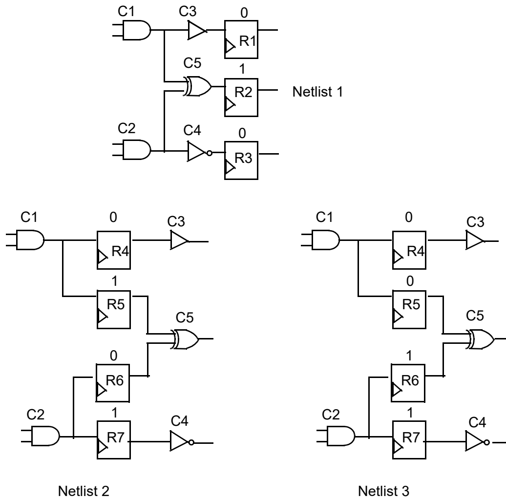
Figure 123 Adaptive Retiming for Registers with Conflicting Reset Values
