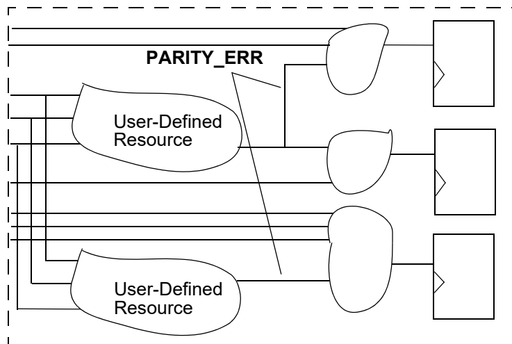
Figure 15 Duplicating User-Defined Resources
