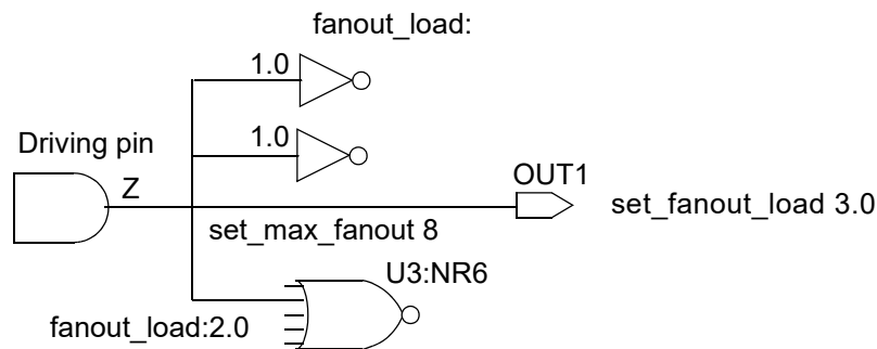
Figure 30 Calculation of Maximum Fanout
