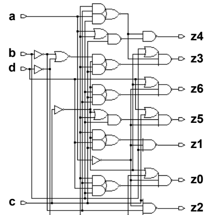
Figure 74 Logic-Level and Gate-Level Optimization for Design LED
