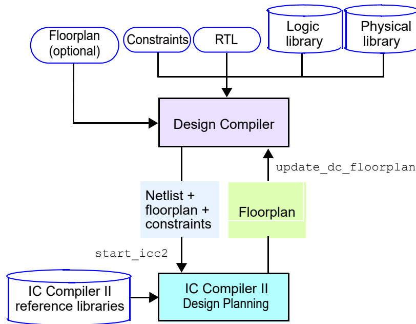
Figure 157 Flow From Design Compiler Graphical to Floorplan Exploration in IC Compiler II
