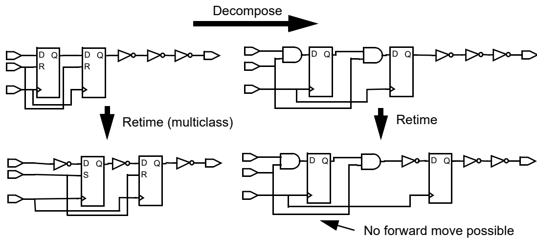
Figure 135 Reduced Mobility After Decomposition
