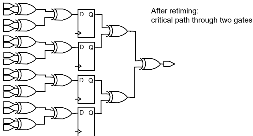
Figure 127 Circuit After Retiming
