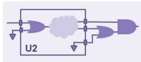
Figure 90 Design After Boundary Optimization With the compile_ultra Command
