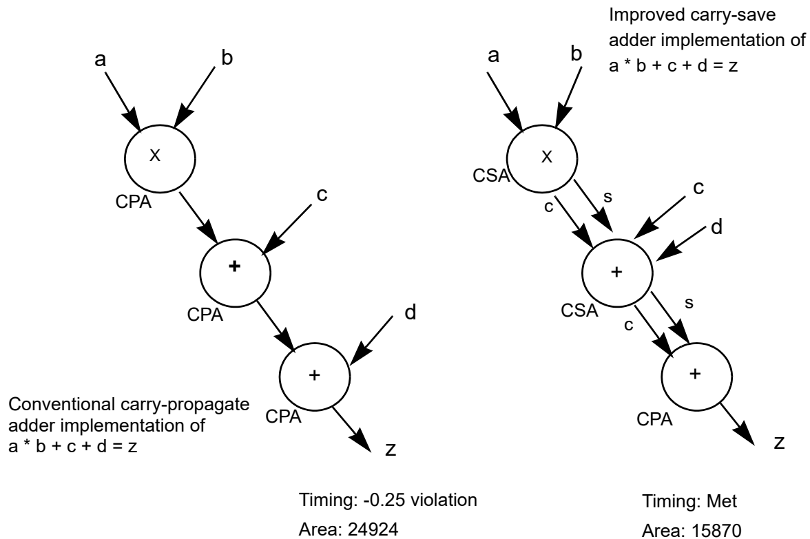
Figure 97 Conventional Carry-Propagate Adder and Faster, Smaller Carry-Save Adder
