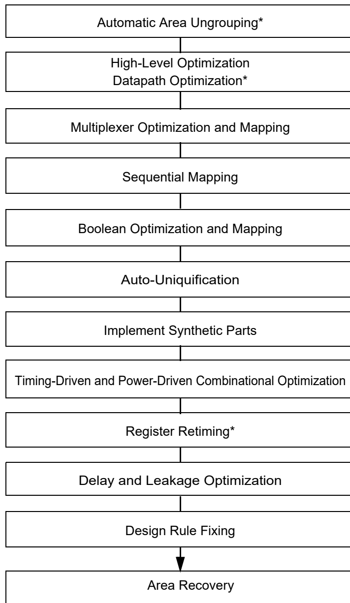
Figure 79 Optimization Flow
