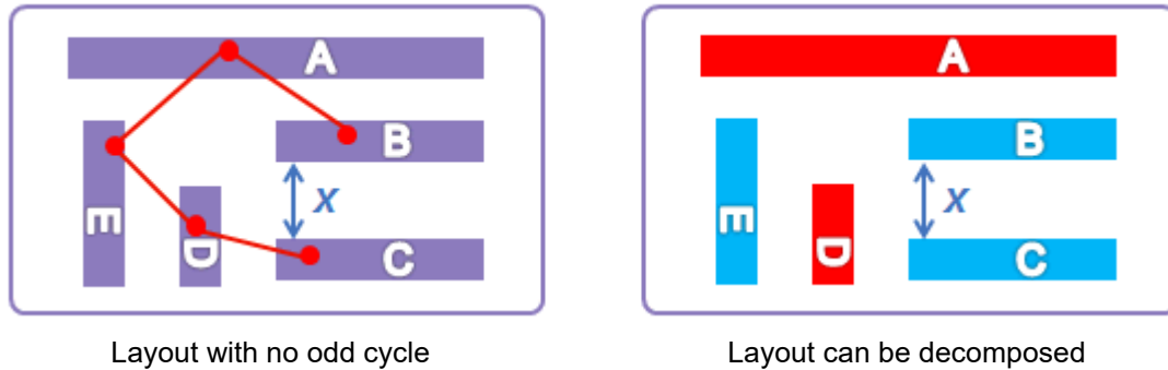
Figure 164 No Odd-Cycle Violation
