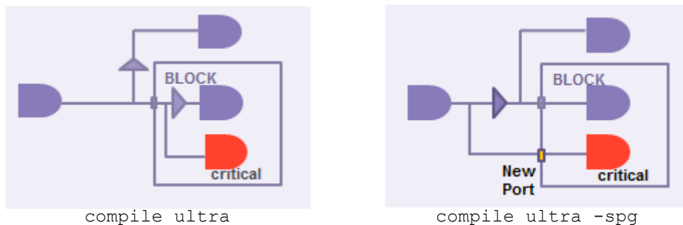
Figure 91 Buffering Across the Hierarchy Comparison
