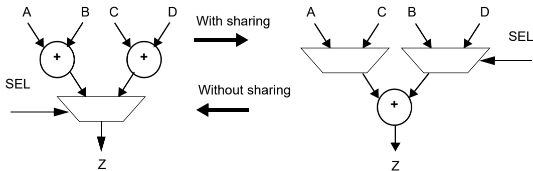
Figure 96 Design With and Without Sharing
