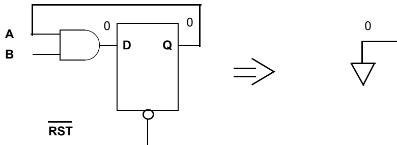
Figure 105 Constant Output Sequential Element That Cannot Escape Its Reset State
