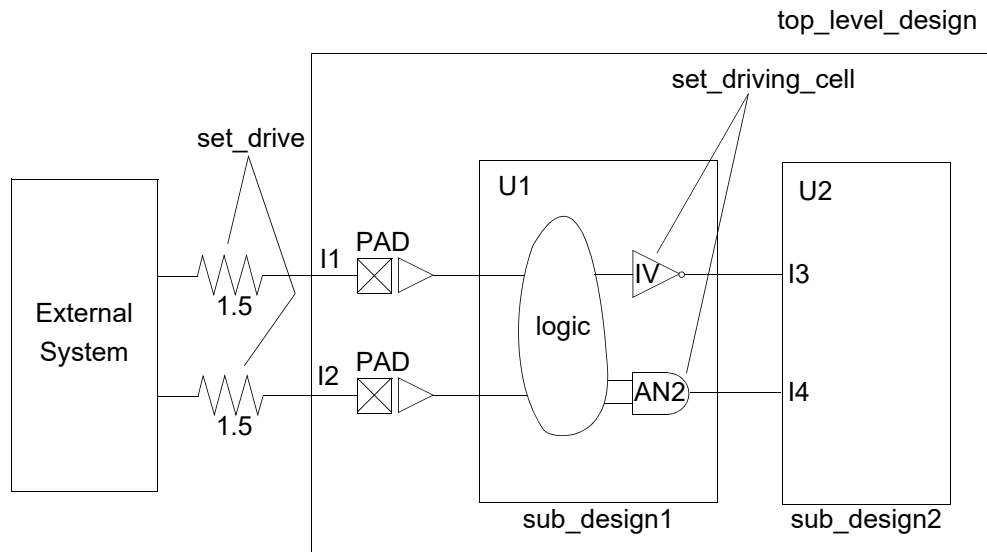
Figure 23 Drive Characteristics
