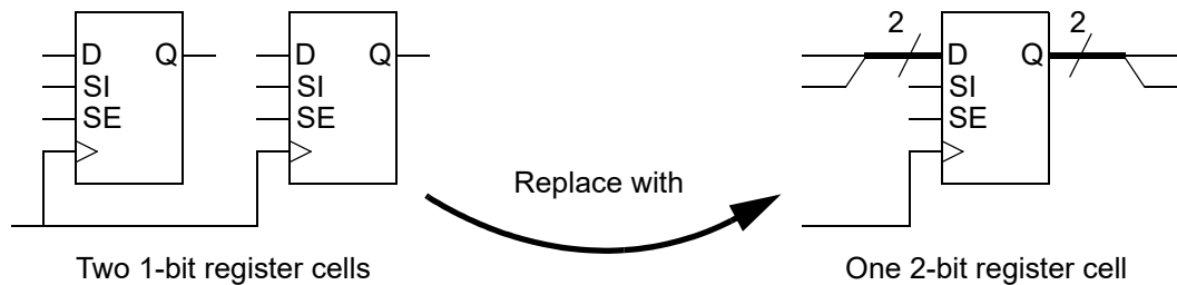
Figure 86 Replacing Multiple Single-Bit Register Cells With a Multibit Register Cell
