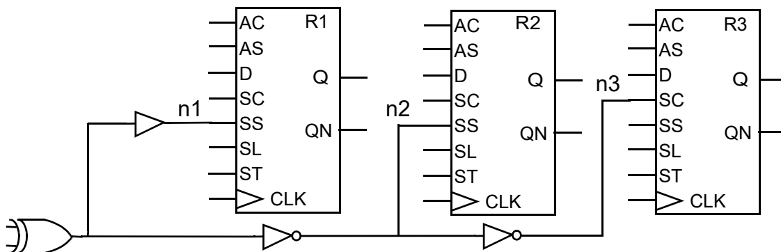
Figure 129 Equivalent Control Net Example
