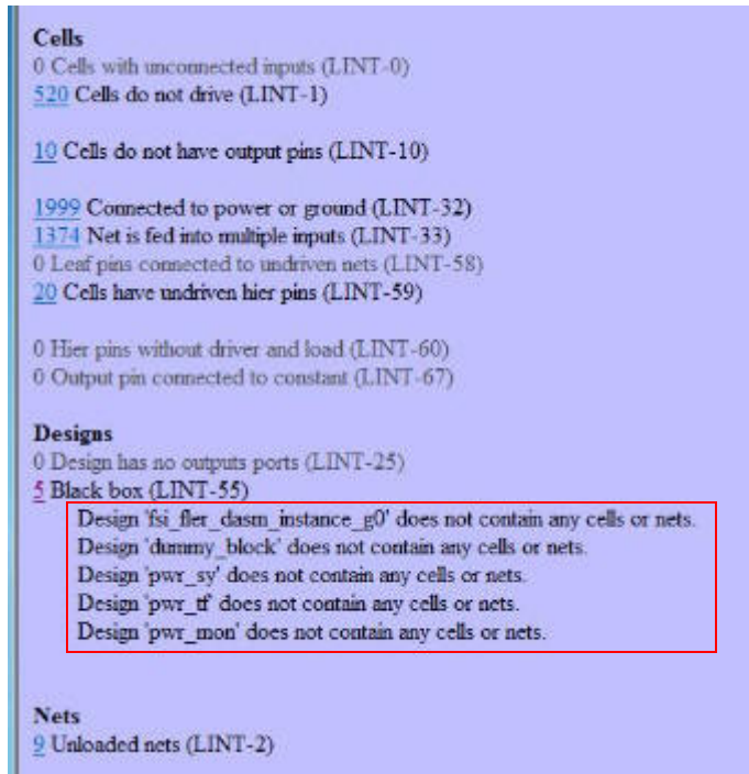
Figure 173 HTML check_design Report Example
