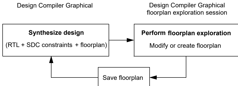
Figure 151 Floorplan Exploration Flow
