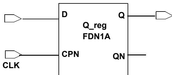
Figure 109 Register Mapped To Logic Library
