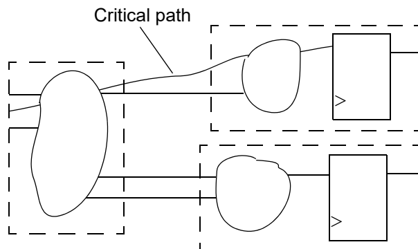
Figure 10 Poor Partitioning of Related Logic
