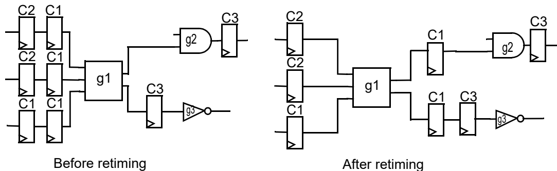
Figure 131 Forward Retiming Example
