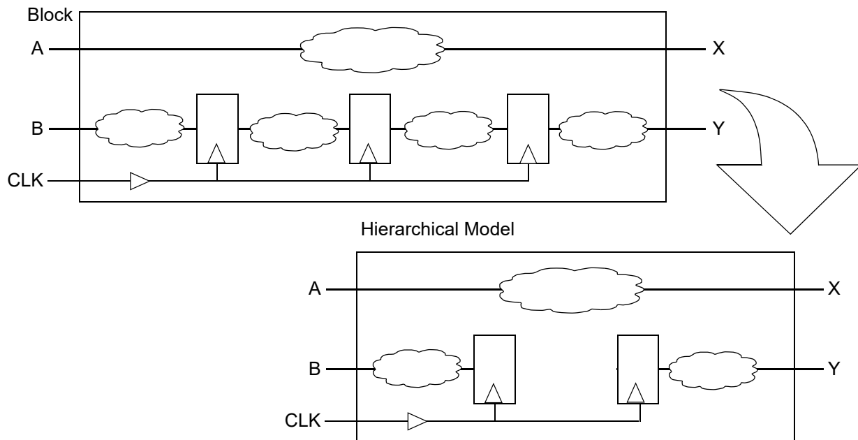
Figure 166 A Block and Its Hierarchical Model
