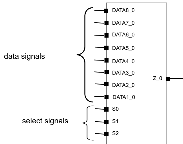
Figure 102 MUX_OP Generic Cell for an 8-bit Data Signal
