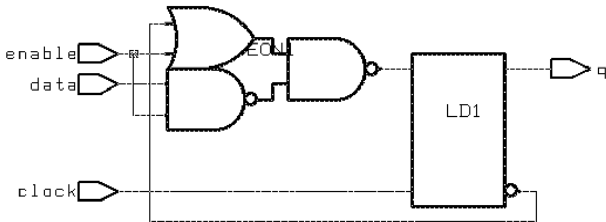
Figure 183 Synthesized Design for a D Latch With Enable
