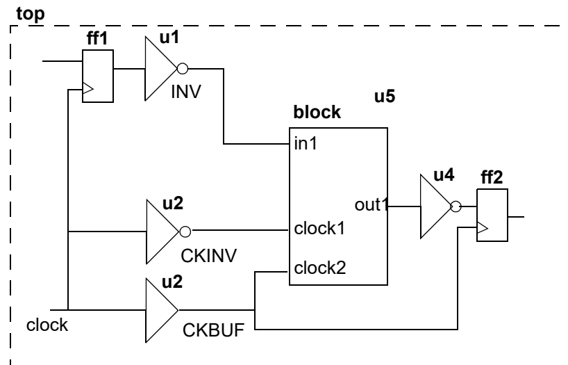
Figure 43 Characterizing Sequential Design Drive, Timing, and Load Values
