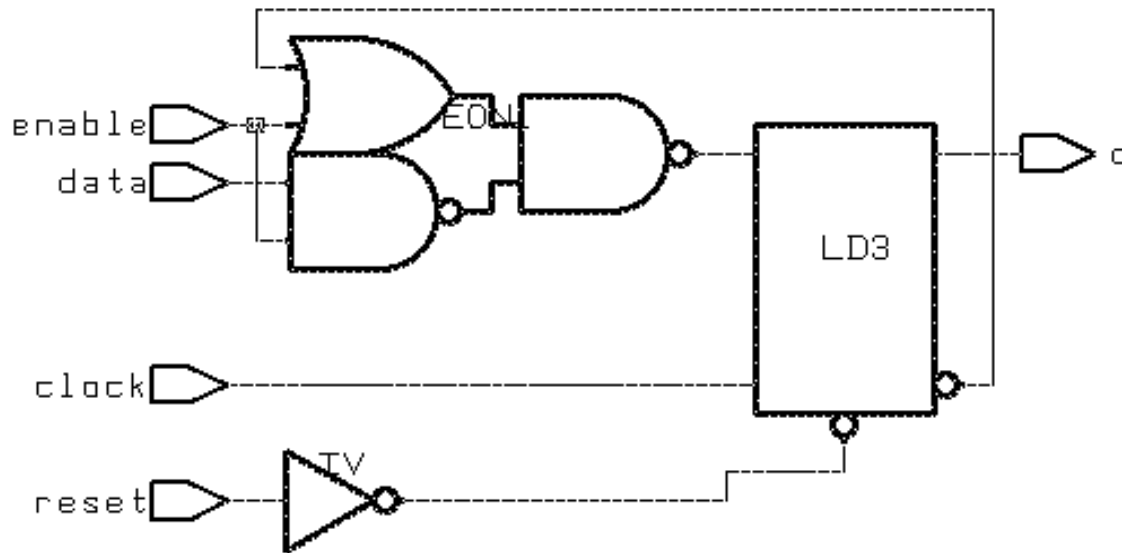
Figure 185 Synthesized Design for a D Latch With Enable and Asynchronous Reset
