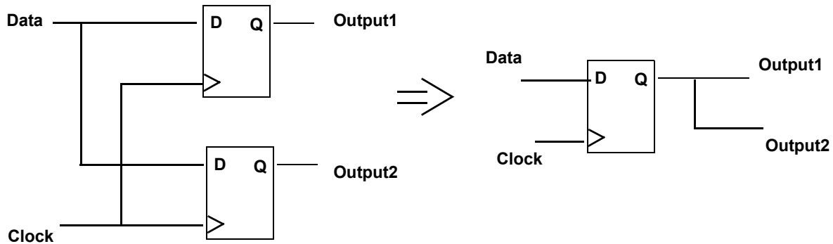
Figure 106 Merging Equal and Opposite Registers
