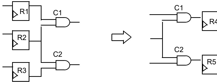
Figure 124 Forward Moves for Non-Critical Registers
