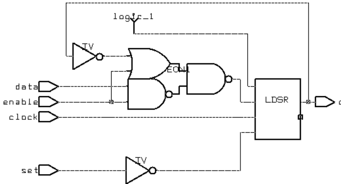
Figure 186 Synthesized Design for D Latch With Enable and Asynchronous Set
