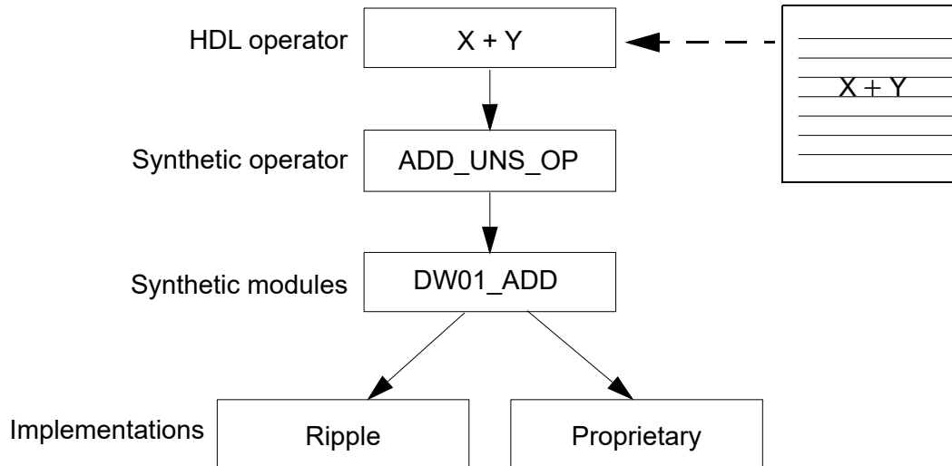
Figure 94 DesignWare Overview
