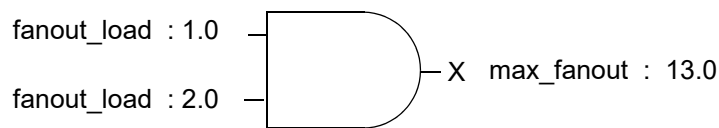
Figure 29 fanout_load and max_fanout Attributes
