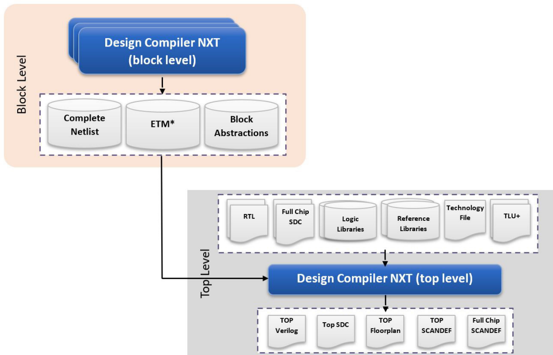
Figure 160 Top-Level Synthesis Using Design Compiler NXT Block Models
