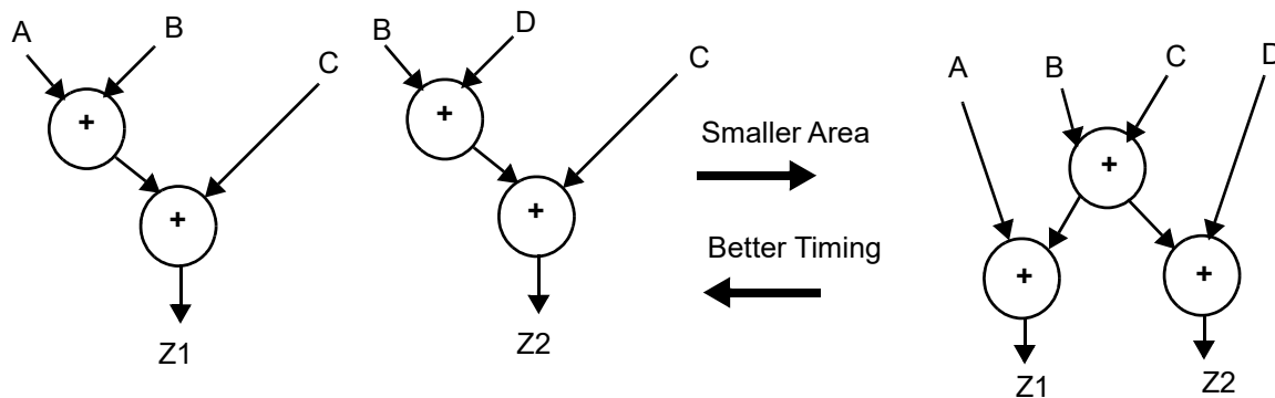
Figure 95 Sharing and Unsharing of Arithmetic Subexpressions
