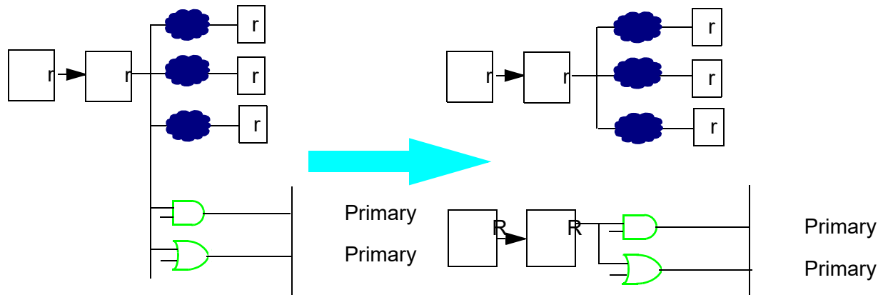
Figure 118 Replicating Registers For the Transitive Fanout
