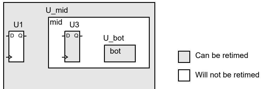
Figure 125 Design With Both Retimable and Nonretimable Cells
