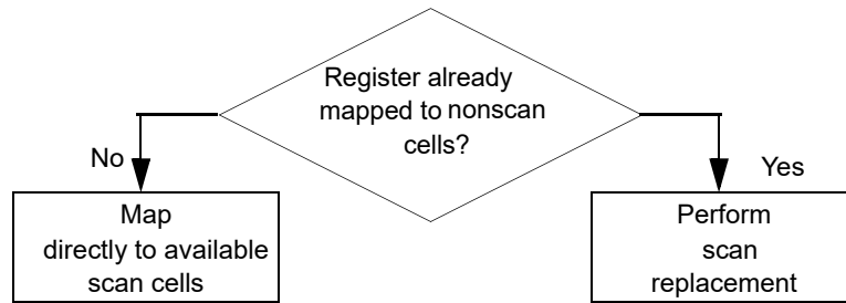
Figure 113 Mapping to Scan Cells
