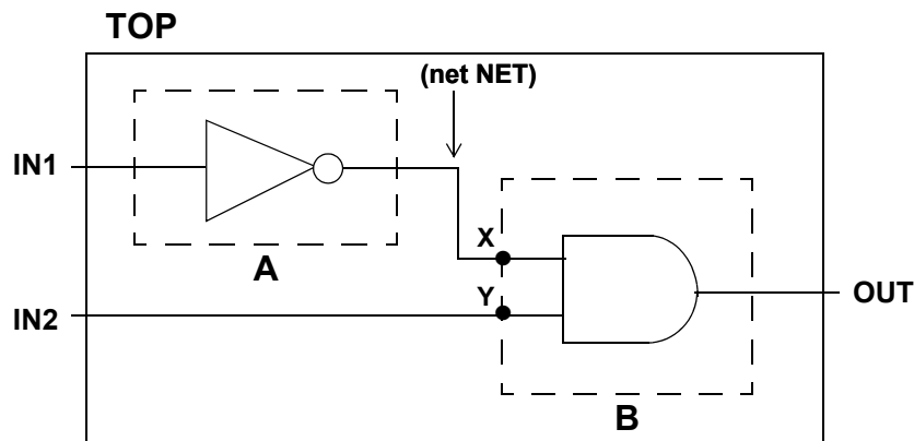
Figure 38 Hierarchical Design Example
