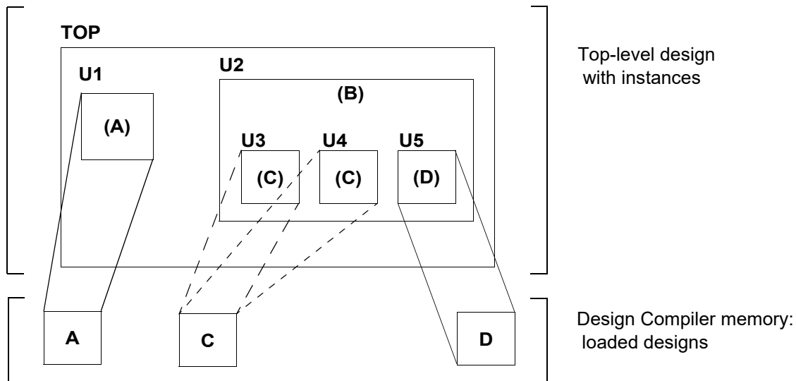
Figure 70 Multiple Instances of a Design Reference
