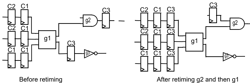
Figure 132 Backward Retiming Example
