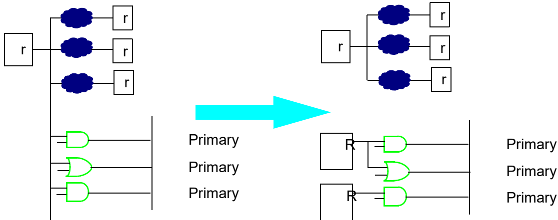
Figure 121 Replicating Registers By Using the -driven_by_original_register Option
