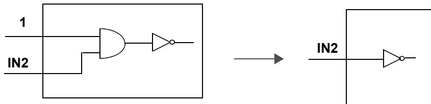
Figure 24 Simplified Input Port Logic
