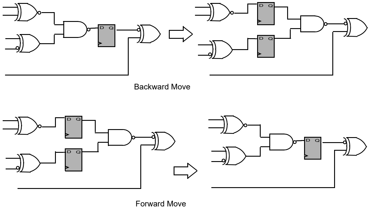
Figure 122 Adaptive Retiming
