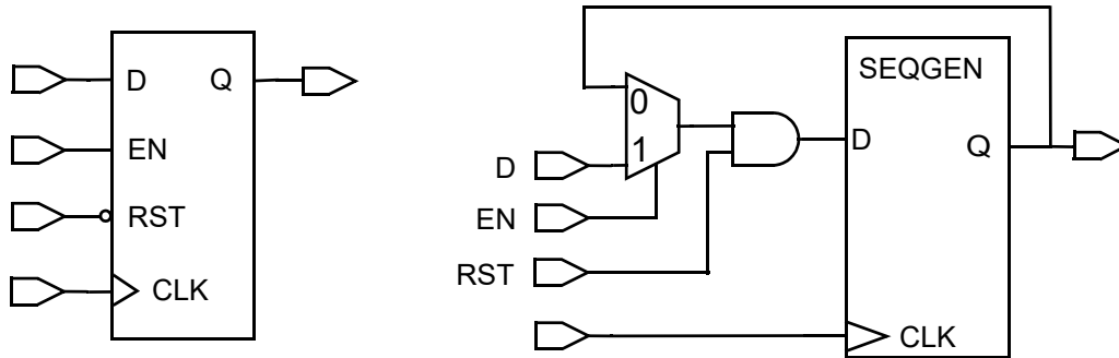
Figure 133 Transformation by Decomposition Example
