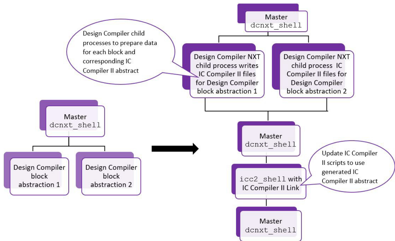
Figure 161 Top-Level Design With Two Block Abstractions of Design Compiler
