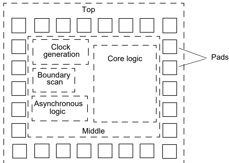
Figure 16 Recommended Top-Level Partitioning
