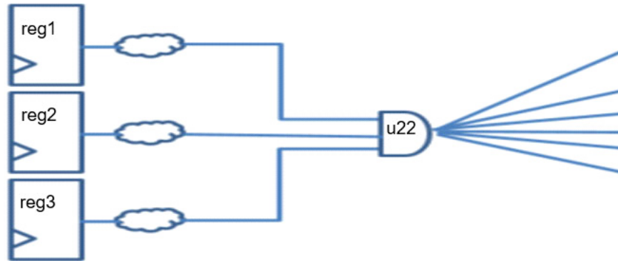
Figure 119 Multiple Registers That Drive a Large Fanout Through a Single Cell
