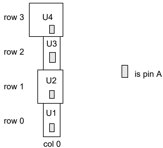
Figure 64 Relative Placement Group Aligned by Pins
