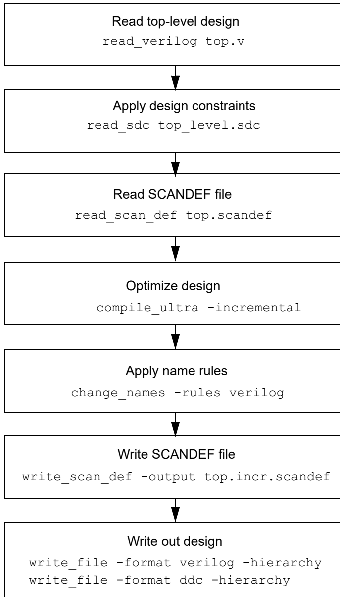
Figure 172 Netlist SCANDEF Flow Example
