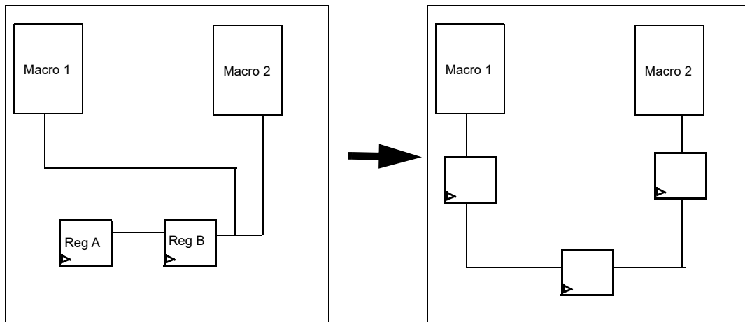
Figure 120 Register Replication Example
