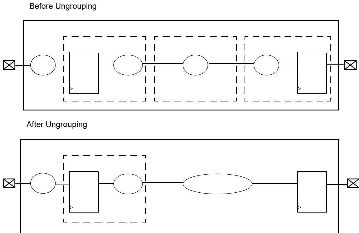
Figure 92 Automatic Ungrouping of Hierarchies
