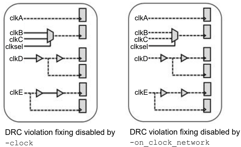
Figure 32 DRC Violation Fixing Disabled for Clock Nets
