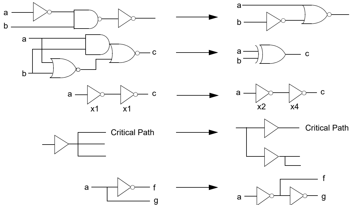
Figure 78 Local Optimization Steps
