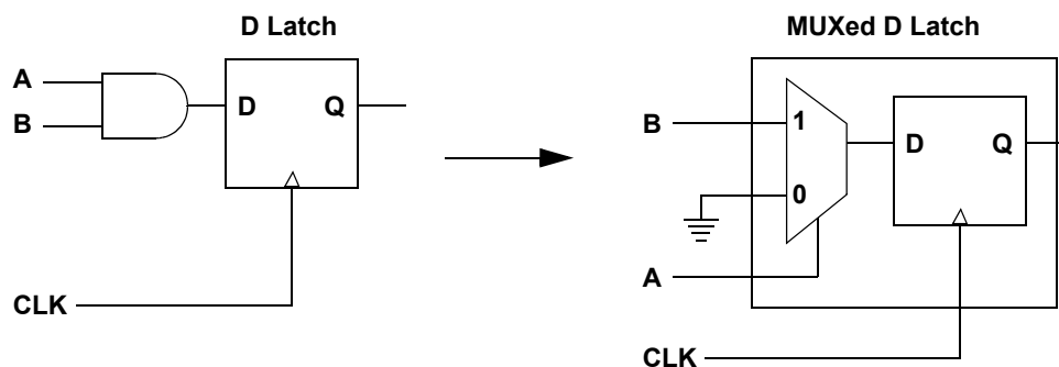
Figure 76 Sequential Optimization
