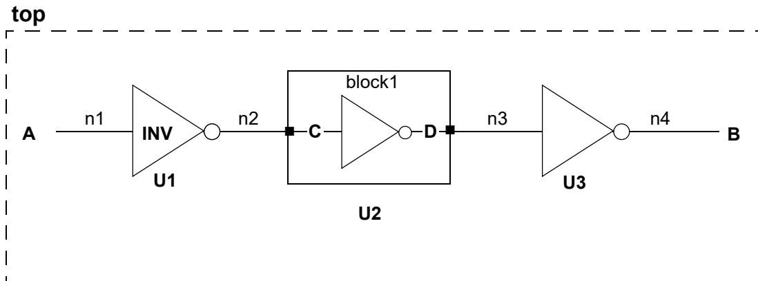
Figure 42 Characterizing Drive, Timing, and Load Values—Combinational Design
