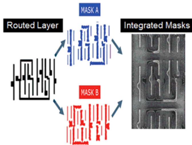
Figure 162 Double-Patterning Example
