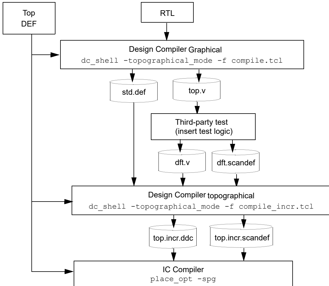
Figure 171 Incremental ASCII Physical Guidance Flow With a Third-Party DFT Flow
