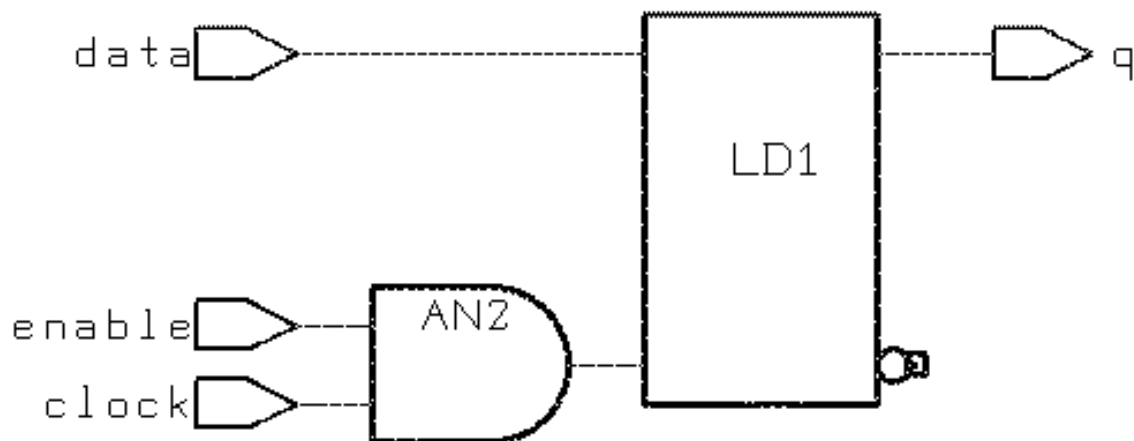
Figure 184 D Latch With Enable and Gated Clock
