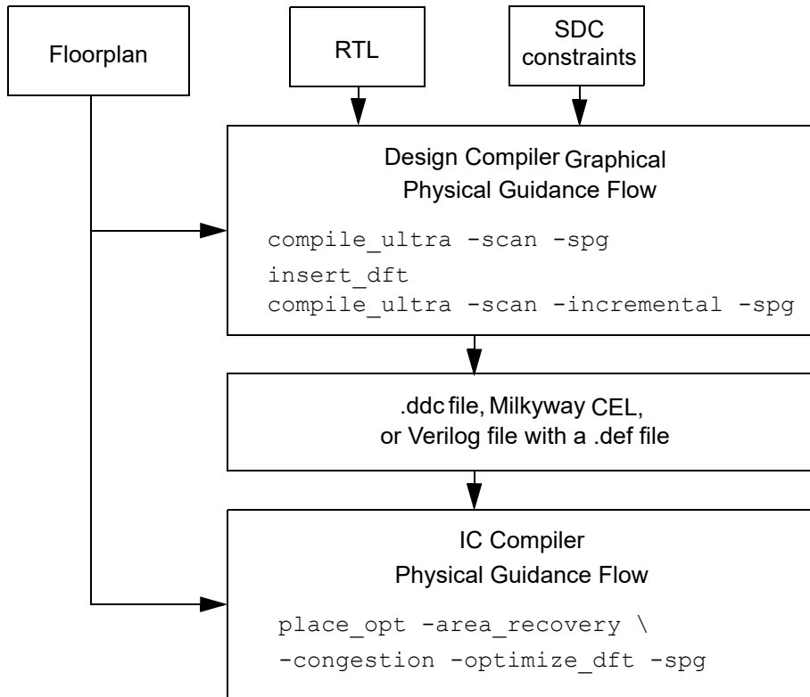
Figure 145 Physical Guidance Flow Example
