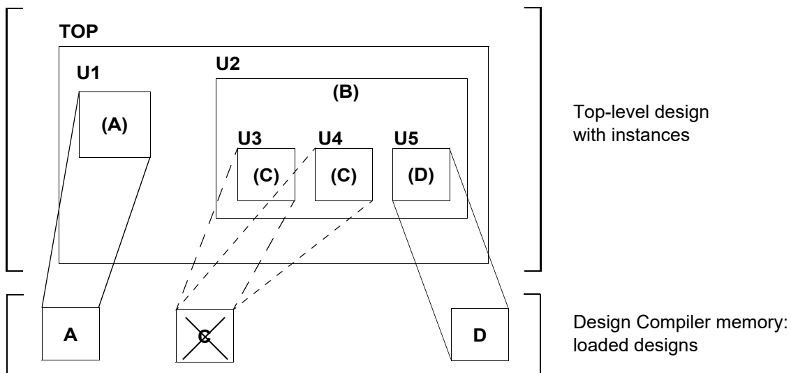
Figure 72 Compile-Once-Don't-Touch Results
