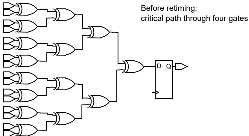
Figure 126 Circuit Before Retiming
