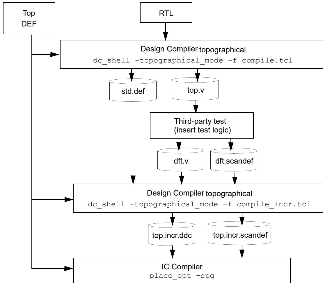
Figure 149 Physical Guidance Third-Party Test Flow
