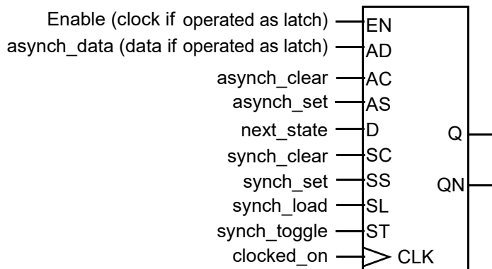
Figure 128 Relevant Pins of the SEQGEN Cell
