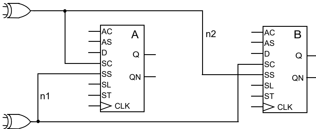
Figure 130 Swapping of Control Net for Registers in the Same Class
