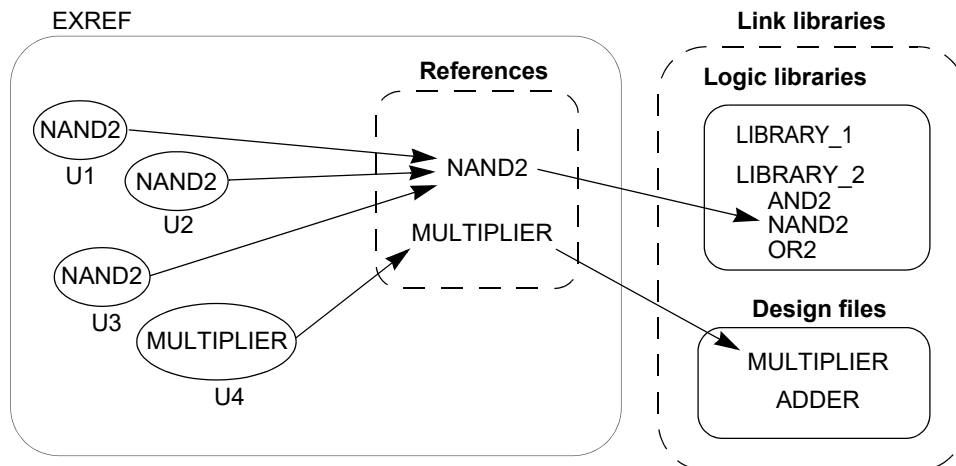
Figure 20 Resolving References
