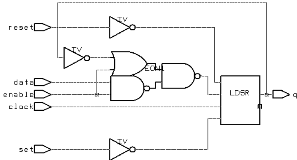
Figure 187 Synthesized Design for D Latch With Enable and Asynchronous Set and Reset
