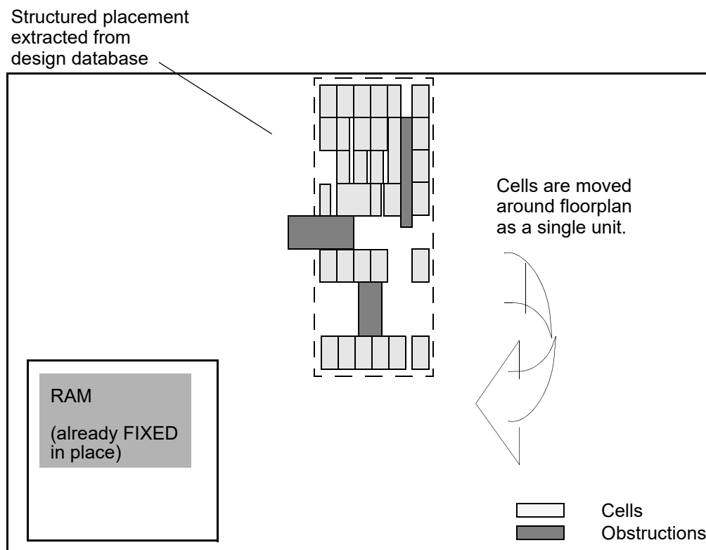
Figure 56 Relative Placement in a Floorplan
