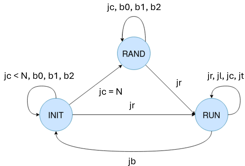
Figure 9: State machine
