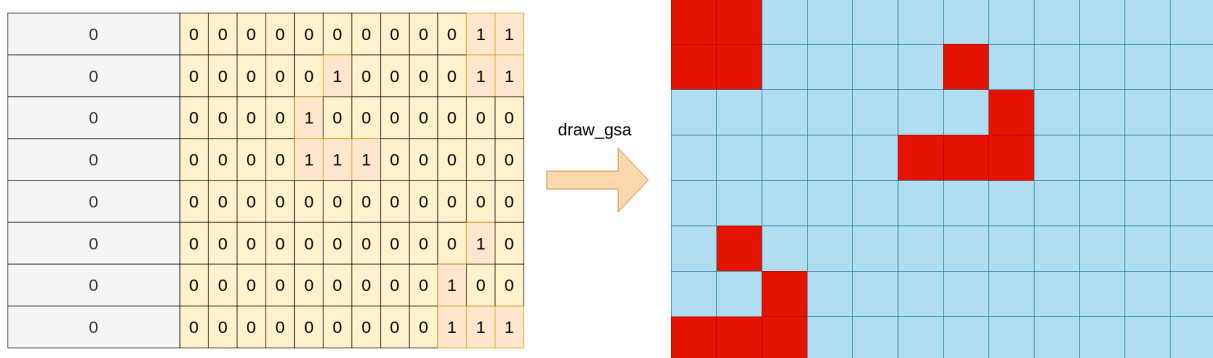
Figure 10: Example of draw_gsa application
