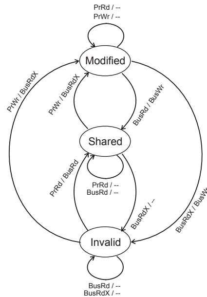
Figure 204: State transition diagram of MSI cache coherence protocol
