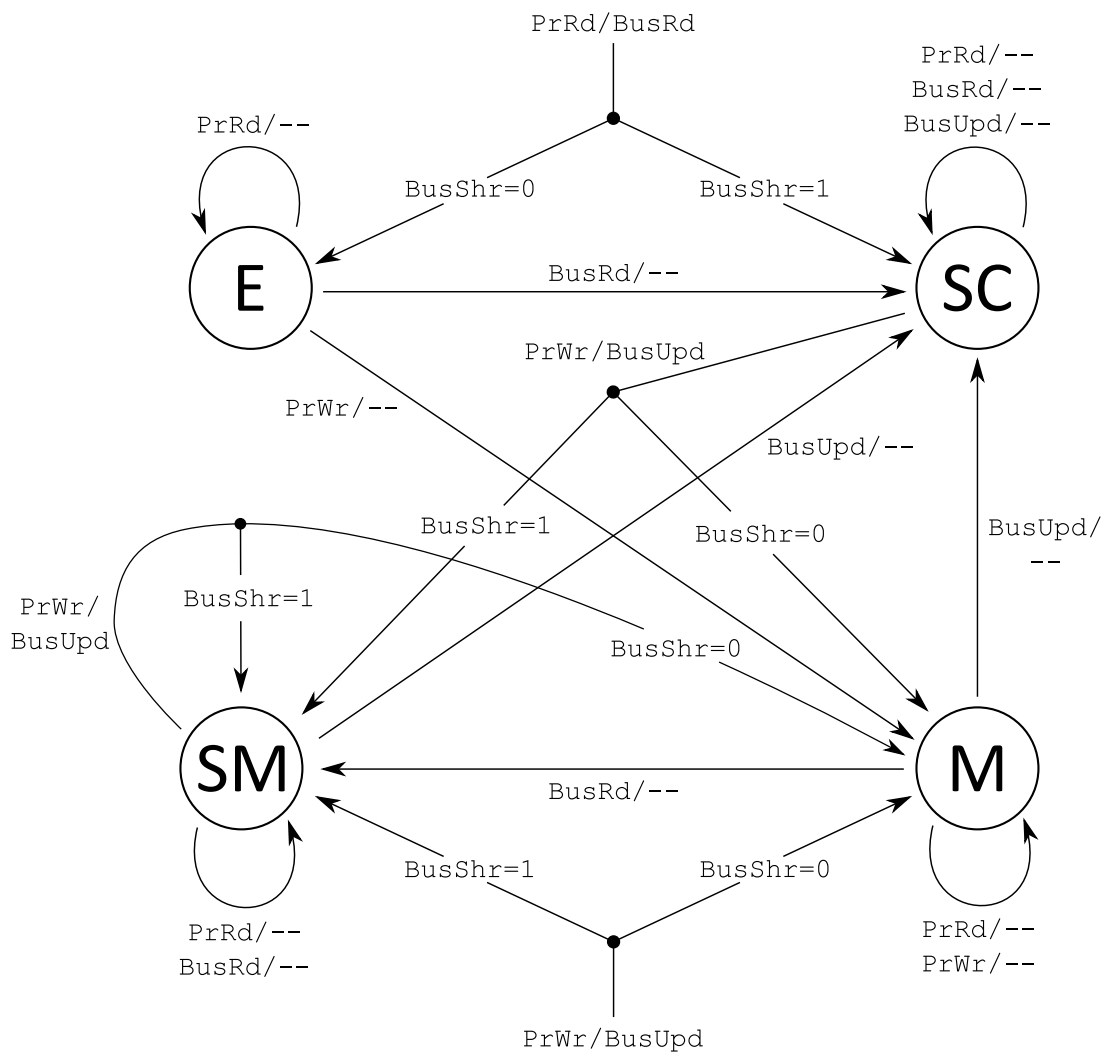
Figure 224: Dragon Cache Coherence Protocol
