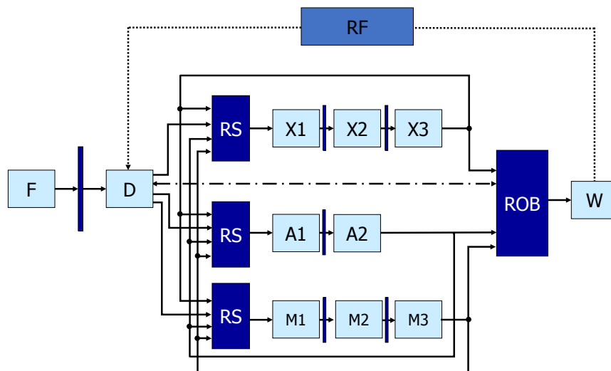
Figure 187: The dynamically scheduled, out-of-order processor.
