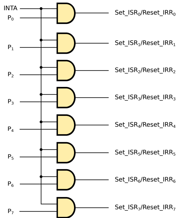
Figure 30: The logic used to generate the Reset_IIR n and Set_ISR n bits.
