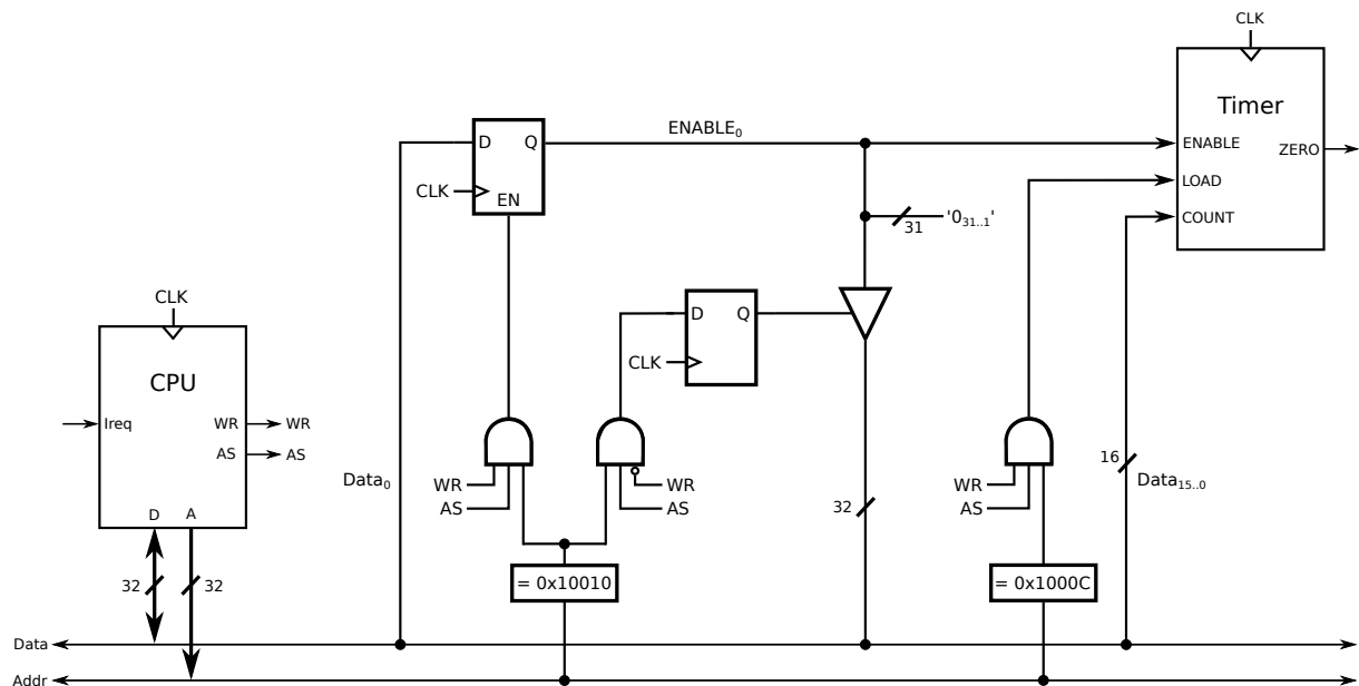
Figure 39: Connecting the timer to the processor.
