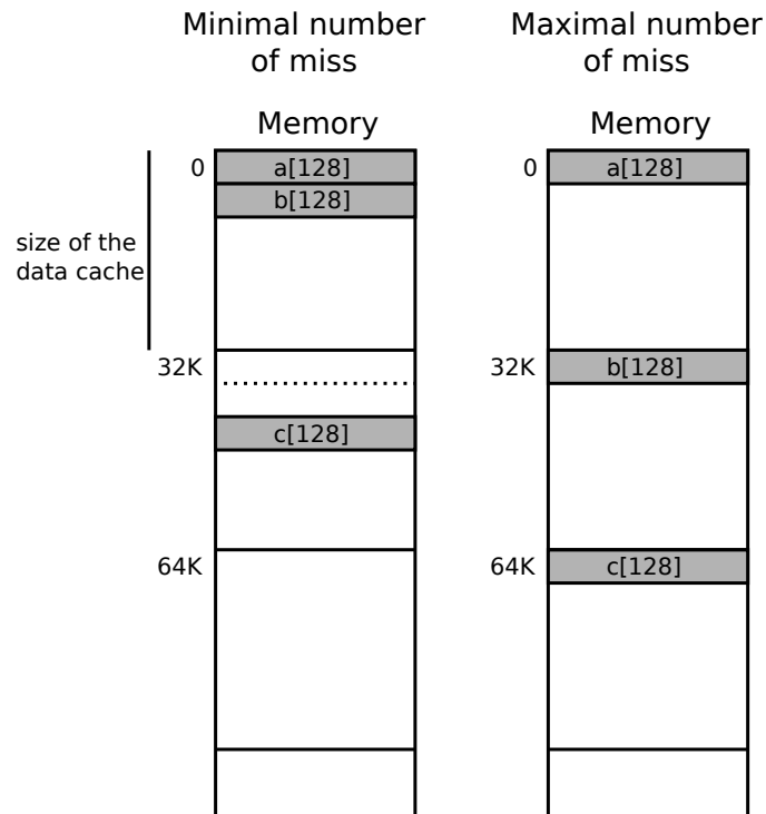
Figure 64: Placing arrays a, b and c
