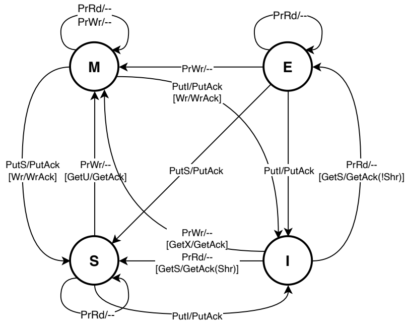
Figure 230: Cache state transition diagram of the cache.
