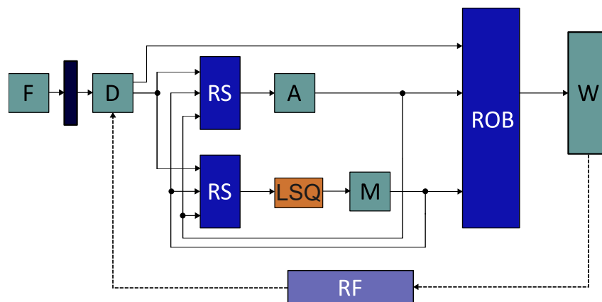
Figure 197: Dynamically scheduled processor architecture with load-store queue (LSQ).
