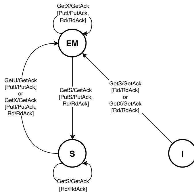
Figure 231: Cache state transition diagram of the directory.
