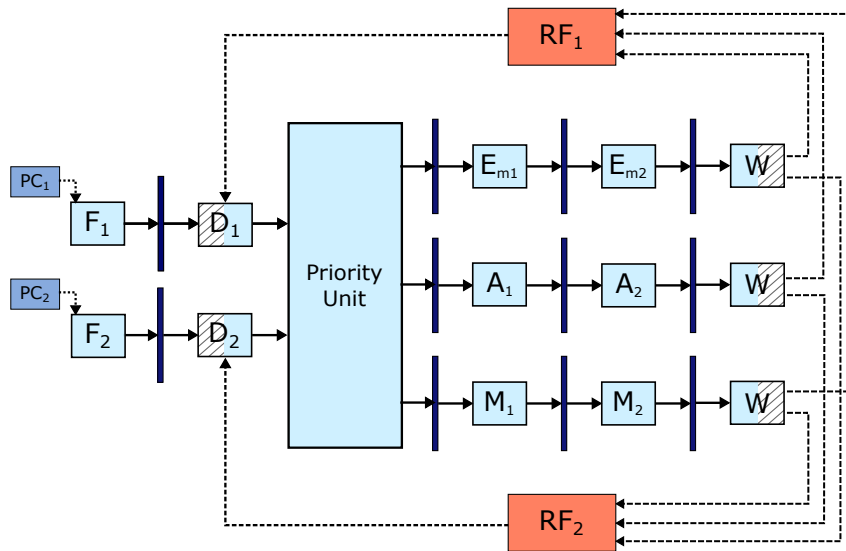
Figure 185: 2-thread processor with three pipelines.
