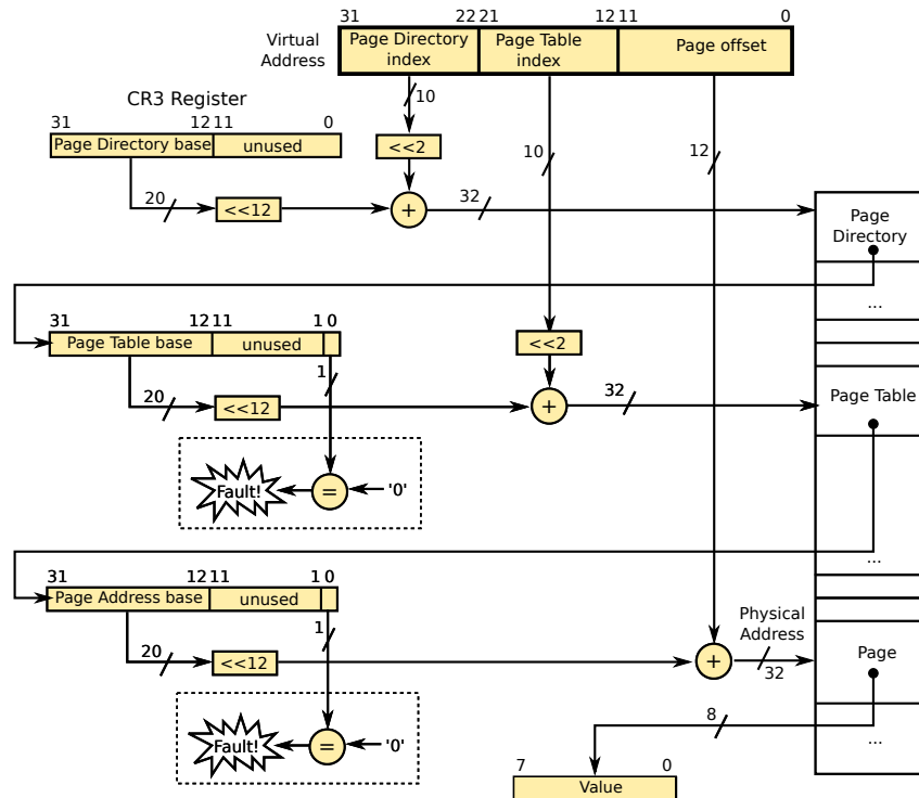
Figure 105: The virtual memory translation process.
