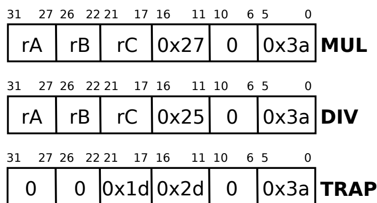
Figure 23: Instruction codes of mul , div and trap .
