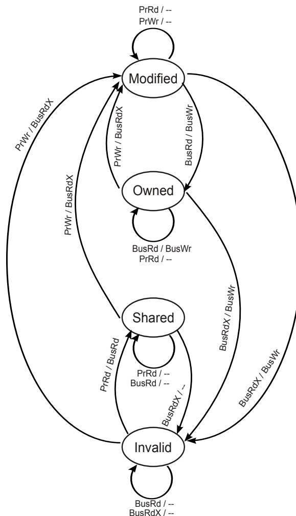
Figure 218: The MOSI protocol diagram.
