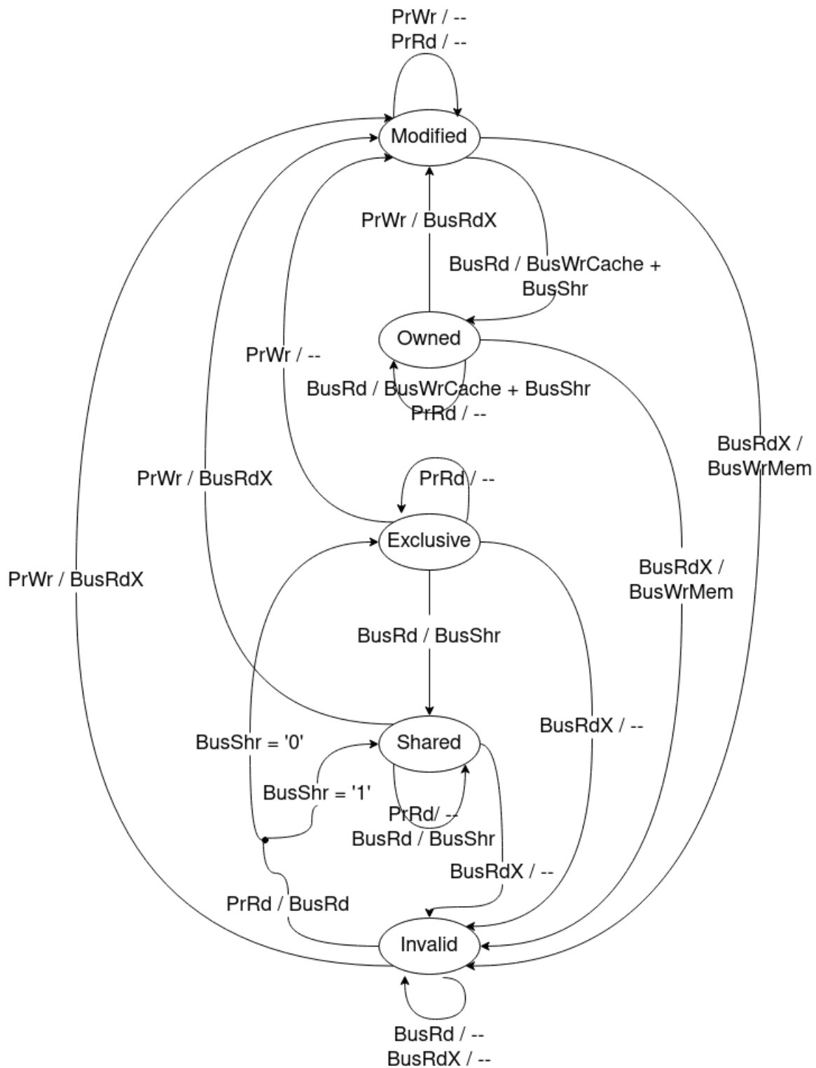
Figure 221: MOESI protocol state transition diagram.
