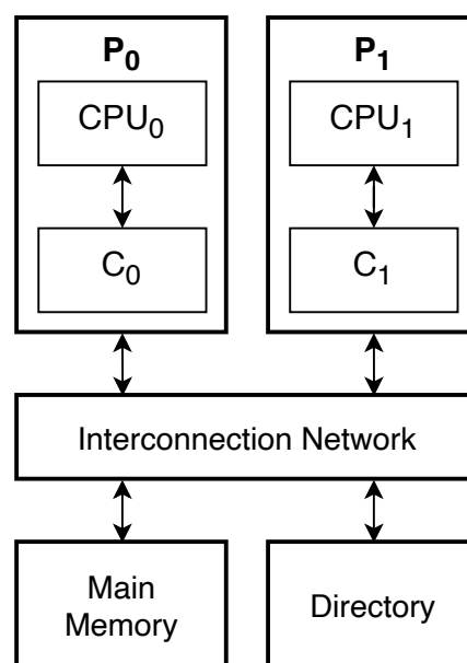
Figure 229: System architecture with two processors, a main memory, and a directory.
