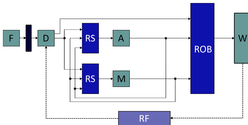
Figure 196: Dynamically scheduled processor architecture.
