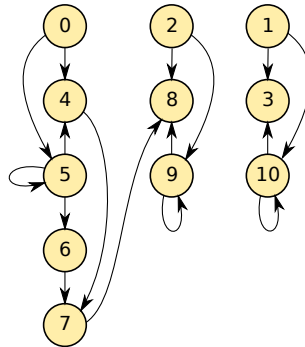
Figure 126: RAW dependencies
