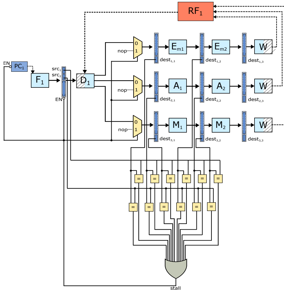
Figure 184: A processor with three pipelines for executing integer instructions.
