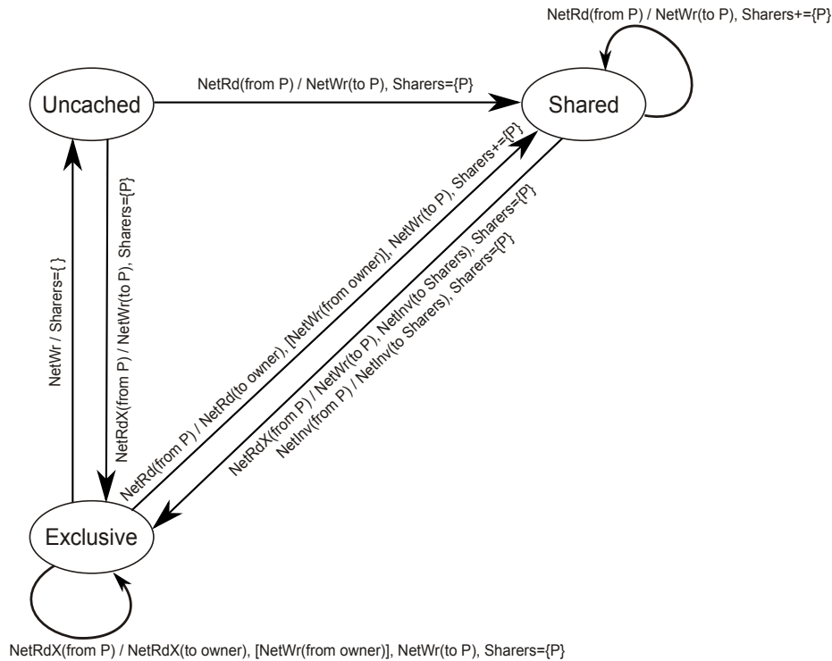
Figure 214: The protocol used to update the states of the directories.
