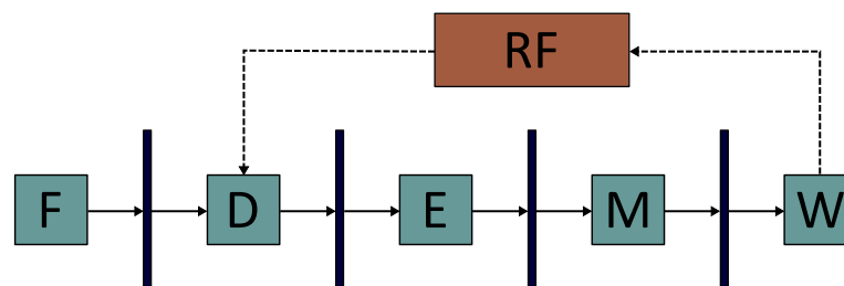
Figure 195: Simple pipelined processor architecture.
