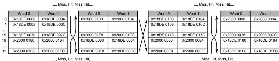
Figure 73: Cache state halfway with 4 word blocks
