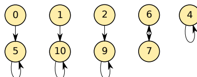
Figure 128: WAW dependencies
