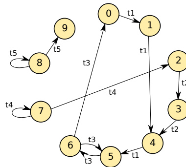
Figure 158: RAW dependencies
