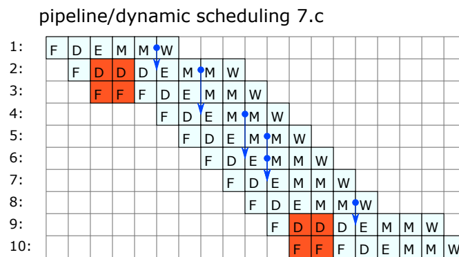
Figure 150: Execution diagram for architecture 4
