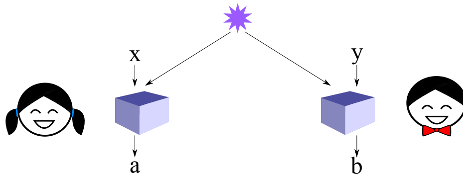
Figure 3.1: A non-local game. Alice and Bob are given questions x and y , and must return answers a and b . If Alice and Bob are quantum, then x and y label measurement settings and a and b are measurement outcomes.
