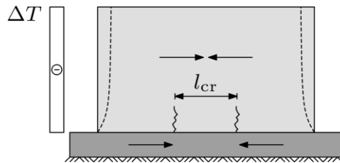
b) separating cracks due to external restraint of a wall on a foundation
