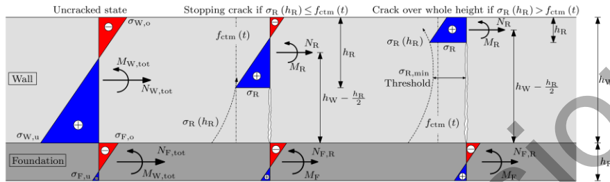
Fig. 8.26 Conceptual model for determination of the crack height in walls restrained by a foundation, based on the stress distribution in the uncracked state (Schlicke, 2014)
