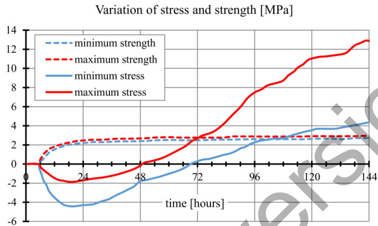
Fig. 8.19 Maximum and minimum stress/strength development from a full probabilistic analysis
