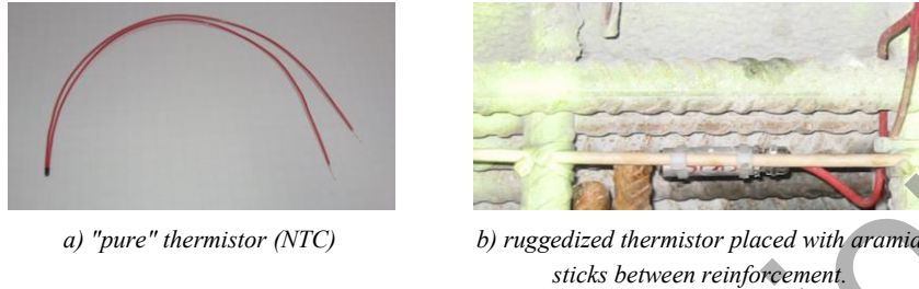
Fig. 9.16. Examples of thermistors (photos: D. Schlicke)
