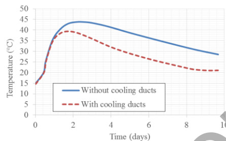
Fig. 6.8 Temperature evolution in the hottest point of the wall for the case in which the cooling pipes were used, and for the hypothetical case of absence of such pipes (simulation) - Adapted from Azenha et al. (2014)
