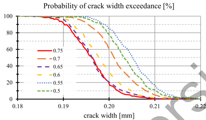
Fig. 8.31 Probability of crack exceedance for different crack criteria after (van der Ham, 2006a)
