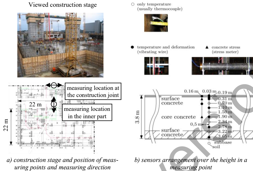
Fig. 9.32. Monitoring program ground slab Boxberg, measuring point “inner part of the slab” (photos: D. Schlicke; drawings: Schlicke, 2014)
