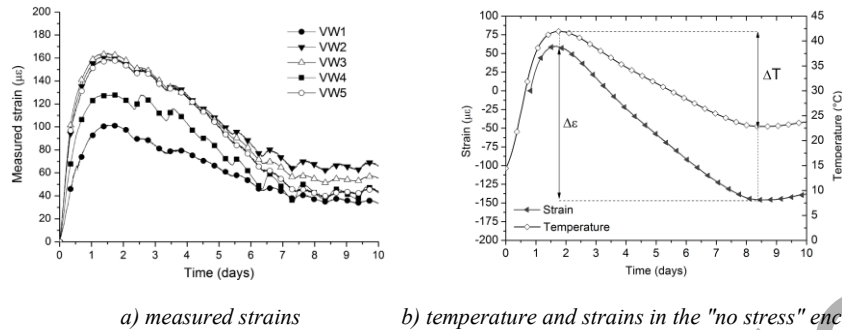
Fig. 9.31. Strain results in the monitored construction phase of Paradela's dam spillway (Azenha et al. , 2014)
