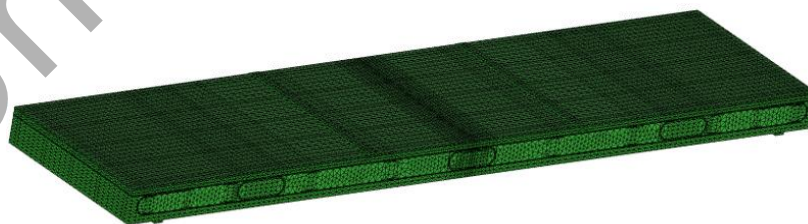
Fig. 7.39 3D finite elements mesh of the beam-slab
