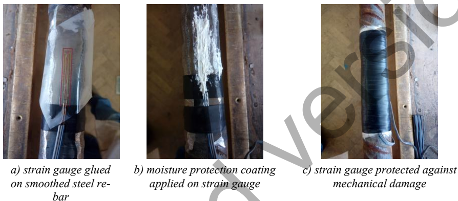
Fig. 9.18. Example of strain gauge installation on a steel rebar (Kanavaris, 2017)
