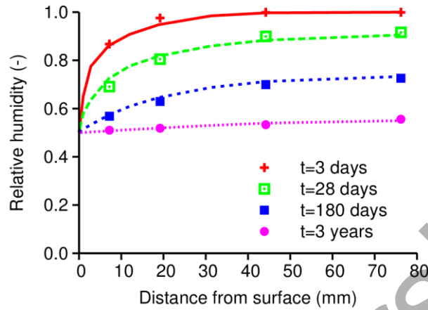
Fig. 7.5 Validation of cylinder drying (Hanson 1968)
