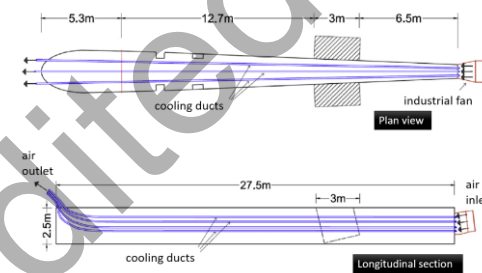
Fig. 6.7 Layout of the cooling ducts in the spillway wall – Adapted from Azenha et al. (2014)
