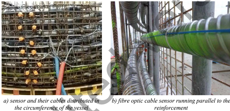
Fig. 9.35. Monitoring sensors in the VeRCoRs project (Oukhemanou, 2016)
