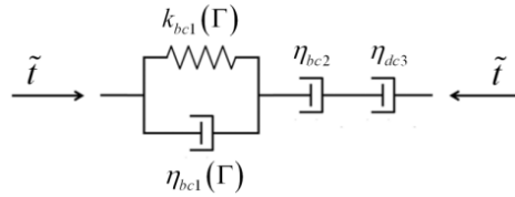
Fig. 7.21 Creep rheological model
