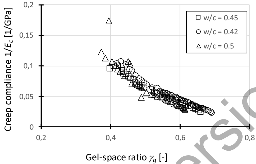
Fig. 4.21 Creep compliance in function of the gel-space ratio for three cement pastes with different W/C ratios (Irfan-ul-Hassan 2016).
