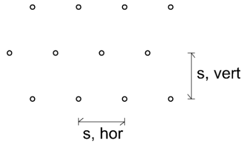
Fig. 6.3 Quincunx arrangement of adjacent cooling pipes for optimized performance
