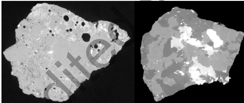
Fig. 10.8. Cross-section of 3D Computerised Tomography microscans for the recycled (left) and natural aggregates (right).
