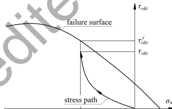
Fig. 7.33 Graphical interpretation of damage intensity factor (adopted after (Majewski 2003))
