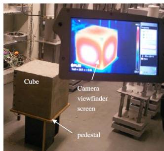
a) Thermal image of concrete cube using a thermal camera (Azenha et al. , 2011)
