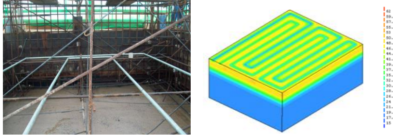
(a) In the field (photograph of W. P. Andrade) (b) Numerical simulation (T in °C)
