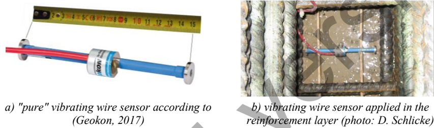
Fig. 9.19. Vibrating wire sensor for embedment in concrete
