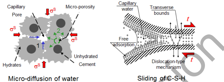
Fig. 4.16 An example of mechanisms for basic creep (Ruetz 1968, Lohtia 1970, Acker and Ulm 2001).
