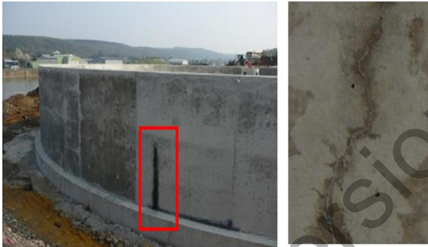
Fig. 8.4 Water treatment plant showing cracking due to the restrained shrinkage at early age and some self-healed cracks (photo: A. Darquennes)
