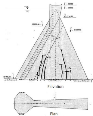
Fig 1.3 Vertical cracks in the buttress of Itaipú dam (adapted from Betioli et al, 1997).
