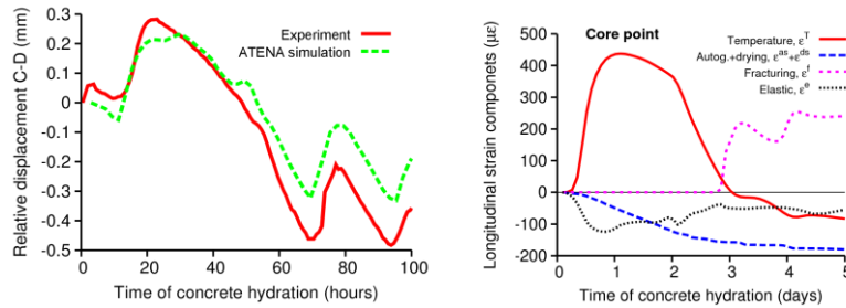
Fig. 7.10 Validation of RG8 ConCrack experiment - experiment overview (by CEOS.fr), cracks at 30 days, displacement of points C-D and strain decomposition at the core point
