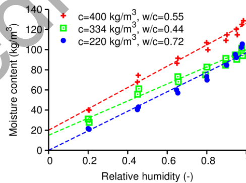
Fig. 7.3 Example of desorption isotherms for structural concrete (Hansen 1986) and linearization
