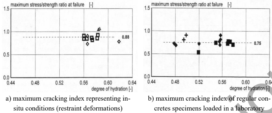
Fig. 8.15 Maximum cracking index (stress/strength ratio) in different conditions after (Lokhorst, 2001)
