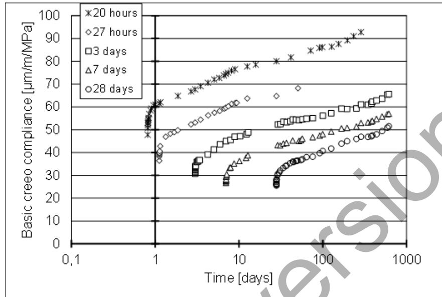
Fig. 4.17 Effects of loading age on basic creep in compression (Laplante 1993).
