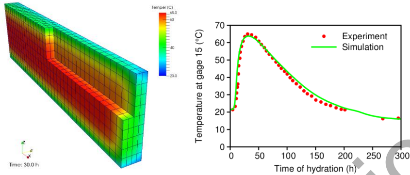
Fig. 7.12 Temperature field at 30 hours and the validation
