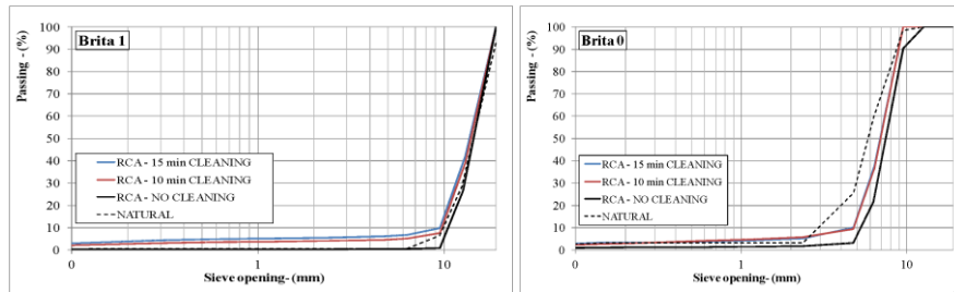
Fig. 10.9 .Grain size distribution comparison for natural and recycled aggregates (adapted from Koenders et al. 2014).
