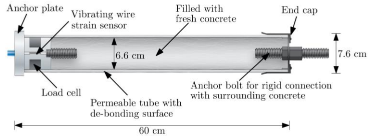
Fig. 9.26. Scheme of Geokon stressmeter, according to (Geokon, 2015)
