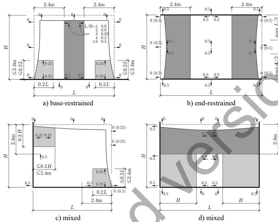
Fig. 8.8 Restraint coefficients in typical situations acc. to (EN 1992-3)
