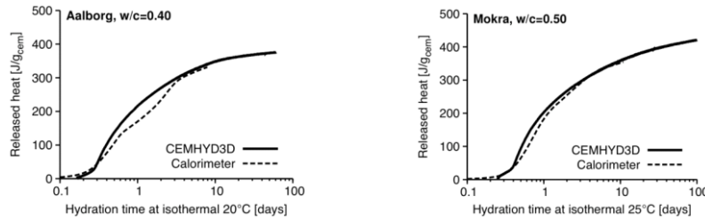
Fig. 2.10 Validation for isothermal calorimetry in terms of released heat (Šmilauer 2014)
