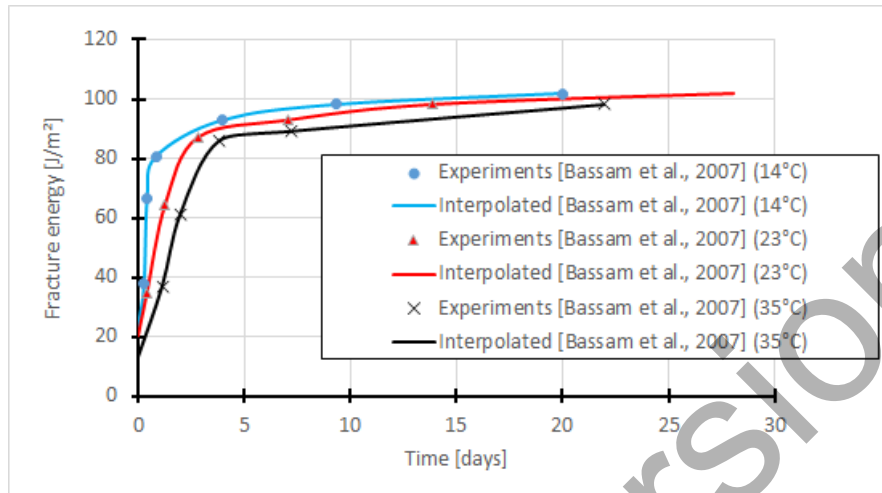
Fig. 4.7 Fracture energy according to time for different curing temperatures (Bassam et al. 2007).
