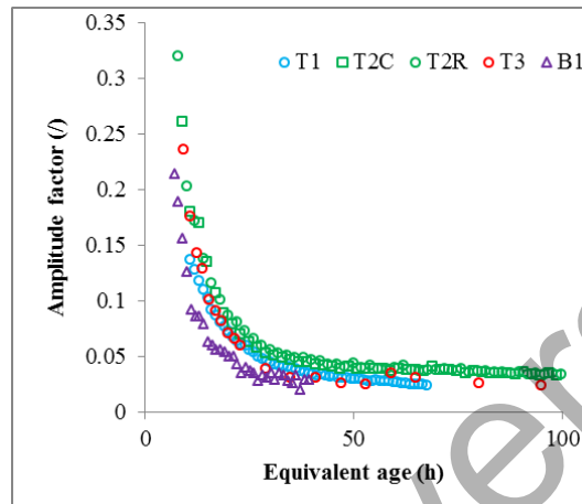
Fig. 4.20 Amplitude factor for creep and relaxation repeated minute-long loading tests in compression (Delsaute et al. 2016b).
