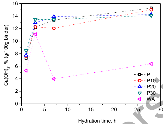
Fig. 10.4. Evolution of \text{Ca(OH)}_2 during hydration obtained from TG analysis: only 27 mass % of the Woody Ash (WA, with particles below 80 \mu\text{m} ) was considered as a binder (adapted from Ukrainczyk et al. 2016).
