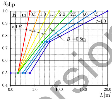
Fig. 8.11 Slip coefficient acc. to (Nilsson, 2000) after (Knoppik-Wróbel, 2015)
