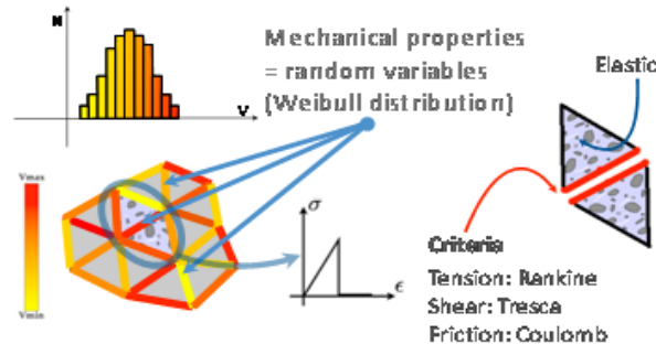
Fig. 7.34 Probabilistic concrete cracking model
