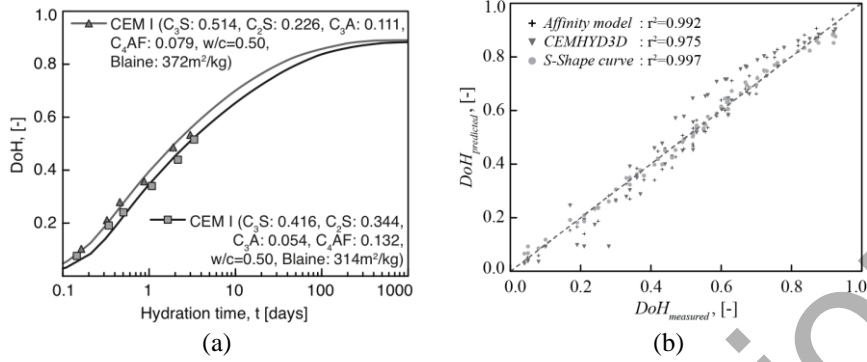
Fig. 2.5 Affinity hydration model: (a) validation based on microstructure-property link from Eq. 2.21 and (b) Scatter plot of measured versus predicted \alpha (Leal da Silva and Šmilauer 2015)
