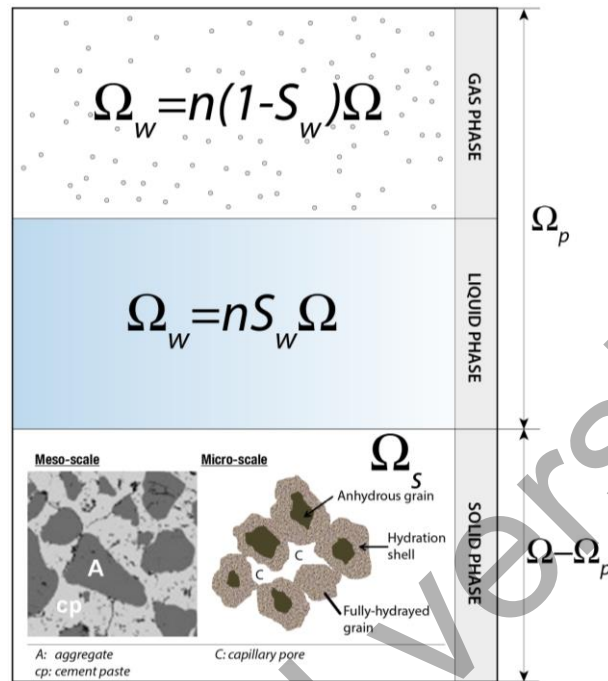
Fig. 7.15 Schematic representation of a non-saturated porous material
