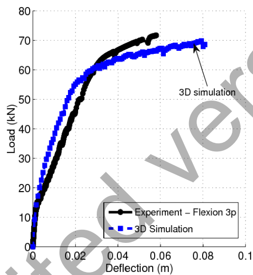
Fig. 7.40 Load-Deflection curves-Comparison between experience and numerical simulation
