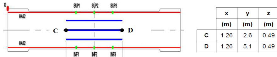
Fig. 7.23 Position of the displacement measurement points (and coordinates)
