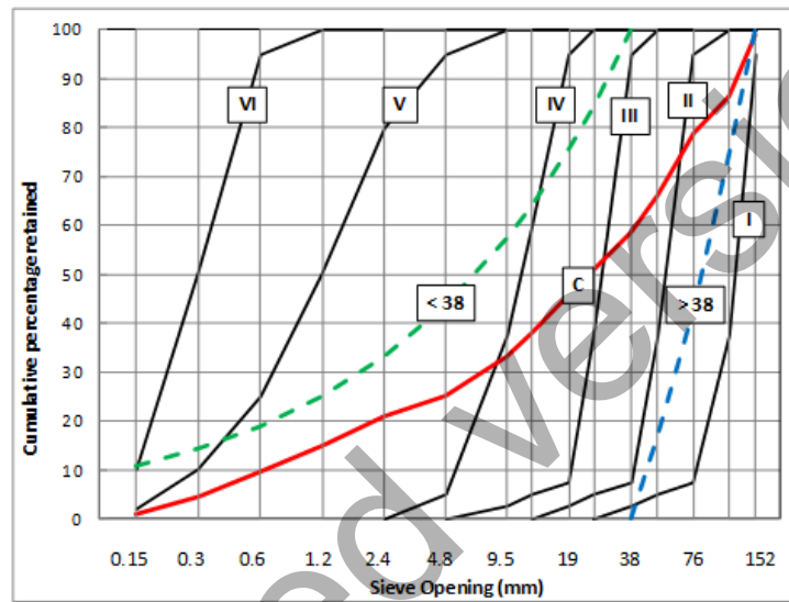
Fig. 5.13 - Grading curves of individual (black), combined (red C) and sieved (dotted lines) fractions
