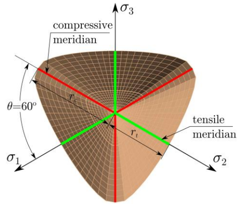
Fig. 7.31 Deviatoric and axiastic sections of failure surface with the modified 3-parameter Willam–Warnke criterion (MWW3, adopted after (Majewski 2003))
