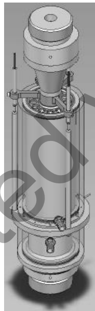
Fig. 1.7 Sketch of BTJASPE, a new testing device was designed at IFSTTAR aimed at measuring automatically the evolution of the stiffness of a concrete cylinder in compression at early age (since the setting time up to a couple of days) (Boulay et al, 2012).
