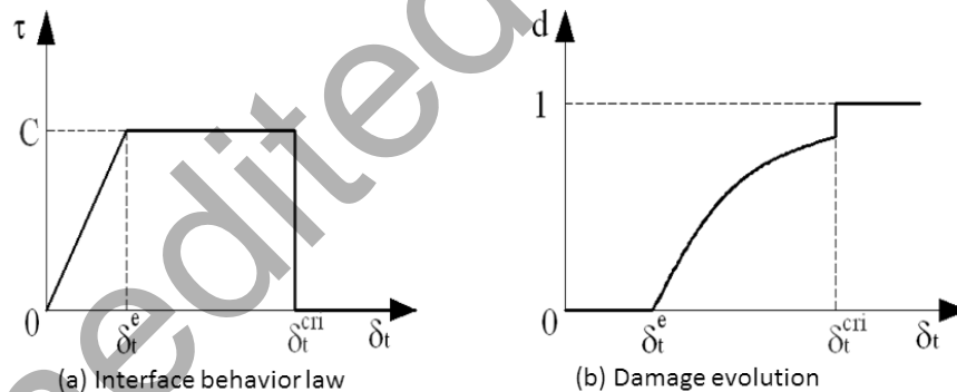
Fig. 7.35 (a) Steel-concrete interface behaviour law (b) Damage evolution
