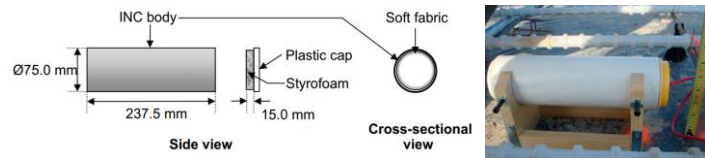
Fig. 9.24. Scheme and photo of the enclosure used by (Yeon et al. , 2013)
