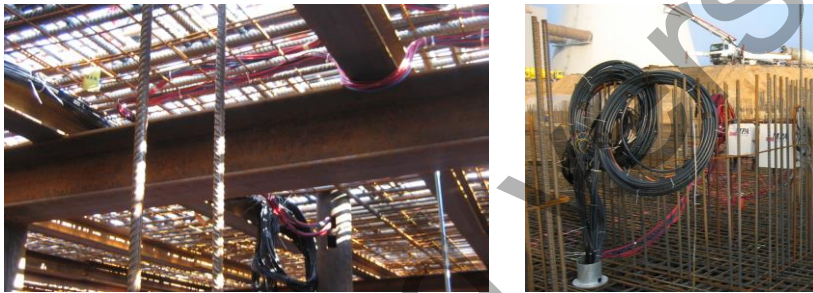
Fig. 9.4. Cable routing and arrangement of the data logger in the monitoring program of the 4.0 m thick power plant slab Boxberg (photos: D. Schlicke)
