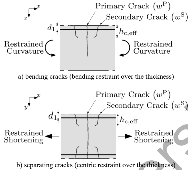
Fig. 8.32 Crack systems consisting of a primary crack and secondary cracks, here A_{c,eff} < A_c
