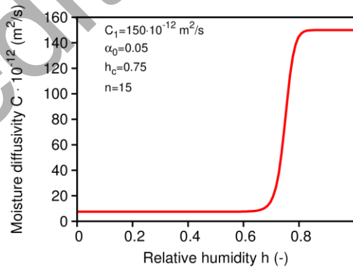
Fig. 7.4 Example of concrete moisture diffusivity (Bažant and Najjar 1972)
