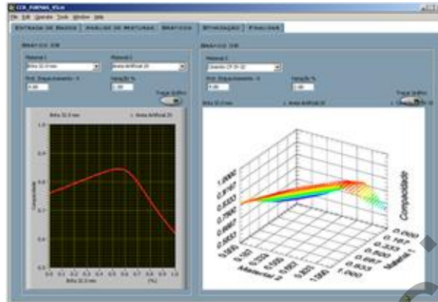
Fig. 5.17 Optimization of RCC mixes using the Compressive Packing Model.
