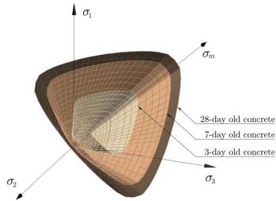
Fig. 7.32 MWW3 failure surface for hardening concrete: a. calibration based on experimental results, b. development during hardening process (adopted after (Klemczak 2007))
