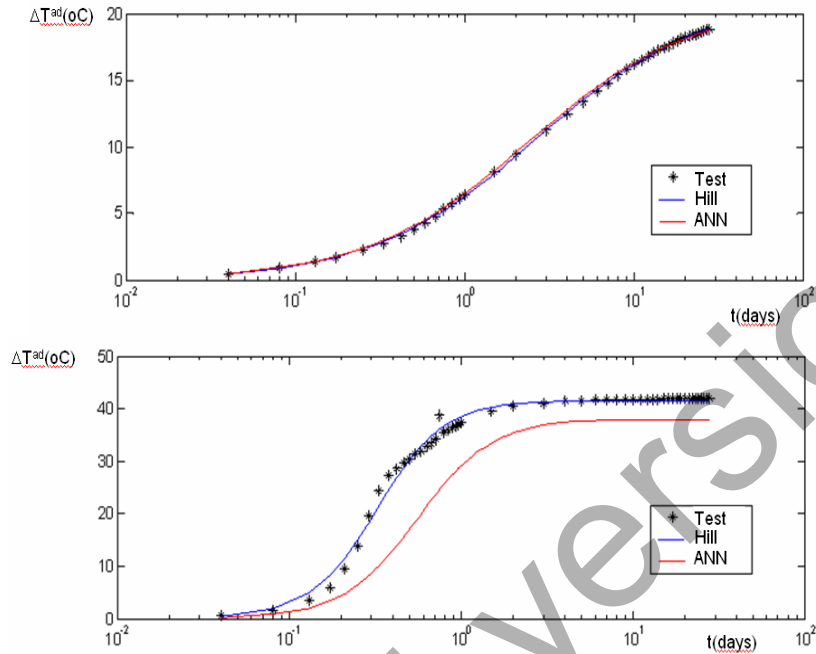
Fig. 2.14 Best and worst fits of the ANN model.
