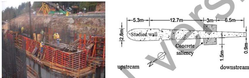
Fig. 9.28. Wall of entrance of Paradela's dam spillway: construction phase studied (photo: M. Azenha; drawing: Azenha et al. , 2014)
