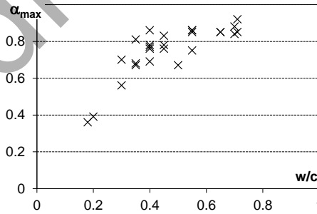
Fig. 2.1 Maximal degree of hydration for Portland cement pastes with different w/c ratios (experimental data reported in(Waller 1999))
