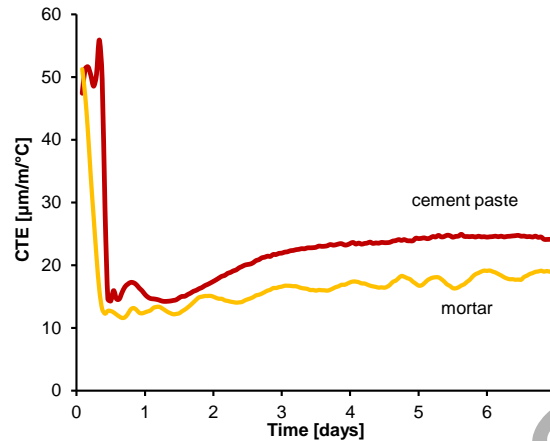
Fig. 3.2 Evolution of CTE of w/c 0.30 cement paste and mortar (with 40% vol. aggregates) during hardening in sealed conditions. For details see (Wyrzykowski and Lura 2013a).
