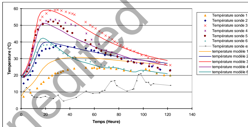
Fig. 7.1 Temperature prediction on Civaux Wall (thickness 1.2 m; height 2.4 m) during hydration (Briffaut 2010)
