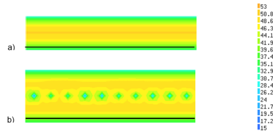
Fig. 6.6 Calculated temperatures for the instant of peak temperature ( t=24 hours): a) 1.5m lift thickness without cooling pipes; 2.4m lift thickness with cooling pipes [Units: °C] - study made at the University of Minho (unpublished)
