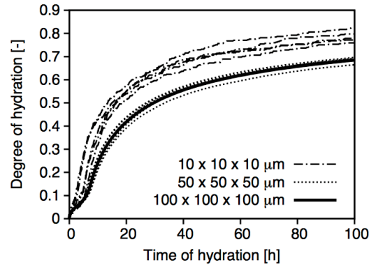
Fig. 2.9 Effect of RVE sizes on degree of hydration with Blaine fineness 250 \text{ m}^2/\text{kg} and w/c = 0.5 (Šmilauer and Krejčí 2009)
