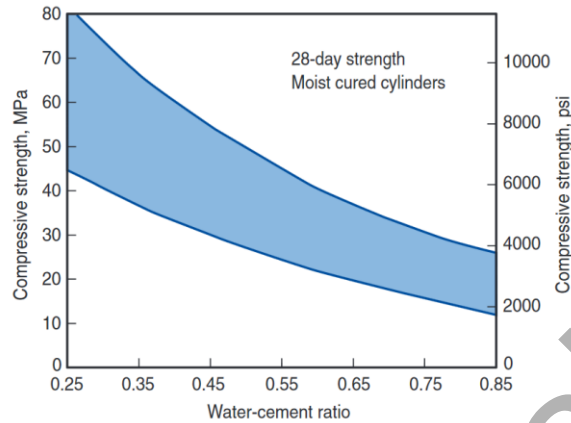
Fig. 5.1 Effect of water-cement ratio on compressive strength [Kosmatka et al. 2002].
