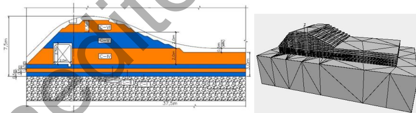
Fig 1.5 Construction scheme and finite element mesh. ( Funahashi Jr and Kuperman, 2010).
