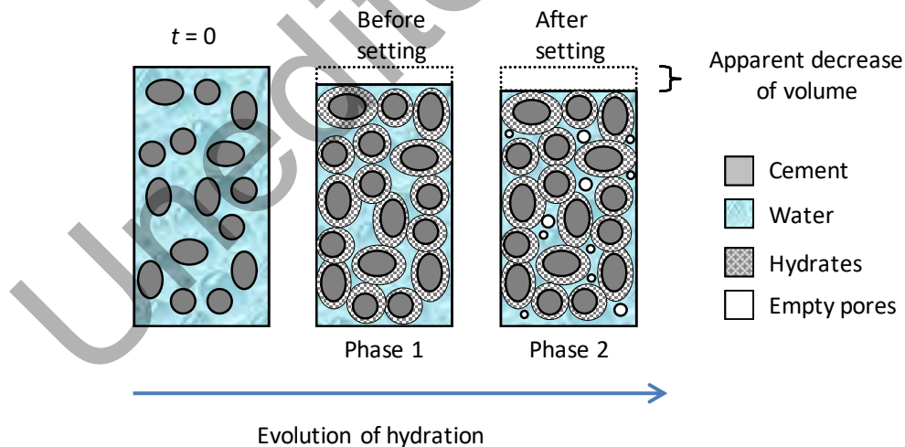
Fig. 4.11 Phases of autogenous shrinkage development.
