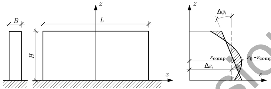
Fig. 8.6 Determination of stresses in a wall-on-slab structure caused by internal restraint according to compensation plane method acc. to (JSCE, 2011)
