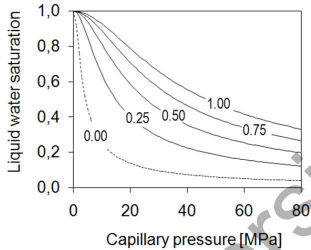
Fig.7.20 Desorption isotherms: the numbers in the diagram indicate the hydration degree (adapted from Sciumé et al. 2013)
