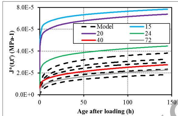
Fig. 4.24 Creep compliance evolution for age at loading of 15 – 20 – 24 – 40 and 72 hours for an ordinary concrete (Delsaute et al. 2017a) and comparison with the Model Code 2010.
