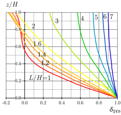
Fig. 8.10 Basic resilience coefficient acc. to (Nilsson, 2000) after (Knoppik-Wróbel, 2015)
