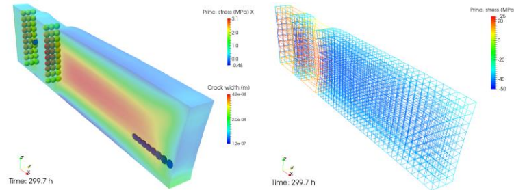
Fig. 7.14 First principal stress, cracks and stress in reinforcement at 300 hours
