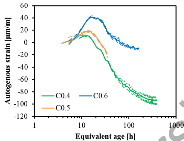
Fig. 4.15 Evolution of the autogenous strain for different water-cement ratios (0.4 – 0.5 and 0.6). Adapted from (Delsaute, 2017b).
