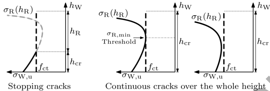
Fig. 8.27 Possible results of the graphically determined crack height in the wall
