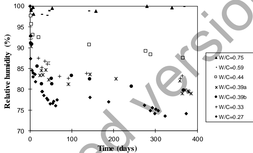
Fig. 4.12 Drop of relative humidity in autogenous conditions for different water to cement ratio (Yssorche-Cubaynes et Olivier, 1999).
