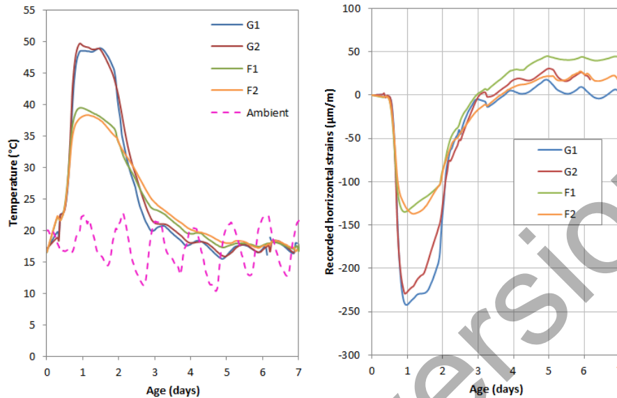
a) Recorded temperatures in various locations in the “gusset”
