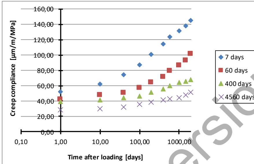
Fig. 4.22 Creep compliance for different age at loading (Browne and Blundell 1969).
