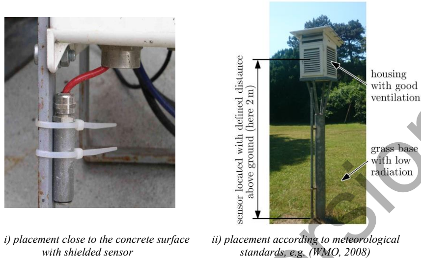
Fig. 9.11. Measurement of ambient air temperature (photos: D. Schlicke)
