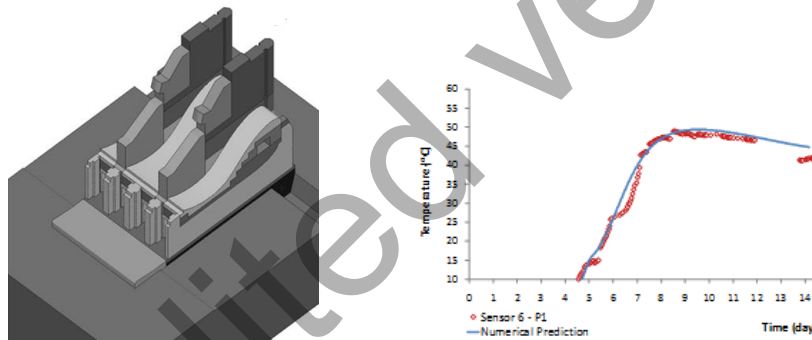
Fig. 2.15 FEM Model of the spillway and comparison between temperature history measured in the bulk of the pier and obtained by using the adiabatic rise curve determined by inverse analysis.
