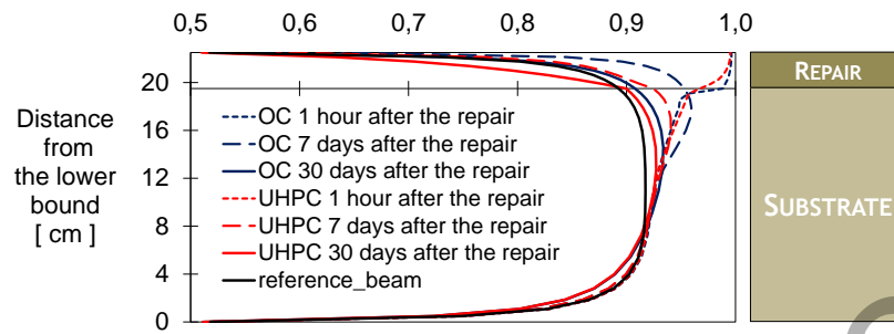
Fig. 7.29 Relative humidity at 1 hour, 1 week and 1 month after repair for the two simulated cases (adapted from Sciumé et al. 2013)
