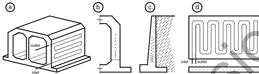
Fig. 6.2 Examples of embedded concrete pipe systems layouts for (a) tunnel segment, (b) gallery wall (linear set-up), (c) retaining wall (staggered set-up) and (d) slab. (Sfikas et al. 2016)
