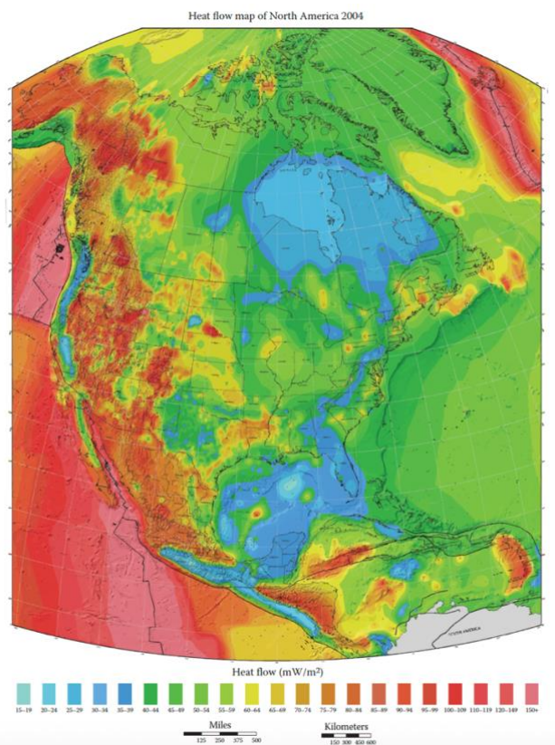
Heat flow map of North America 2004. (from Glassley)
