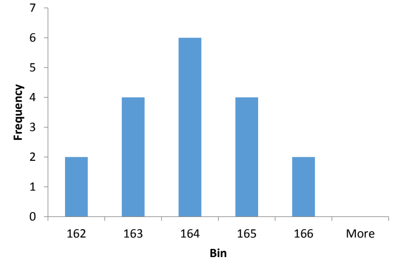
Histogram Pines
